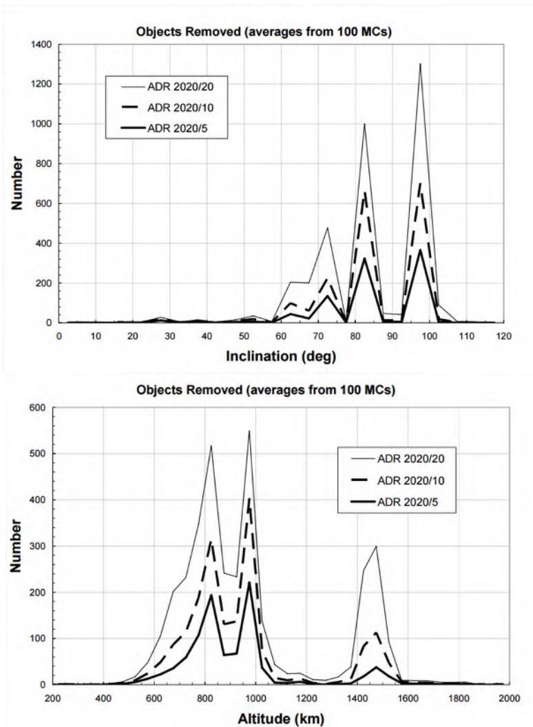
Figure 7. Debris Object Populations. The grouping of ‘worst offending’ objects into a small range of orbits enables the removal of multiple objects with a single launch through the use of secondary payload ADR systems.
