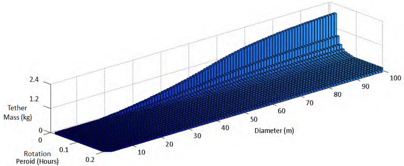
Figure 14. WRANGLER Tether Design. WRANGLER can de-spin massive asteroids using an extremely small tether.
