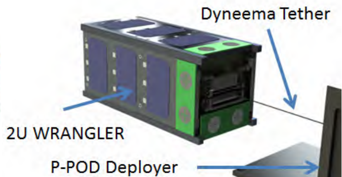
Figure 18. 2U WRANGLER Deployment from P-POD The tethered WRANGLER concept is compatible with a range of CubeSat standard deployers for easy integration into existing mission architectures.
