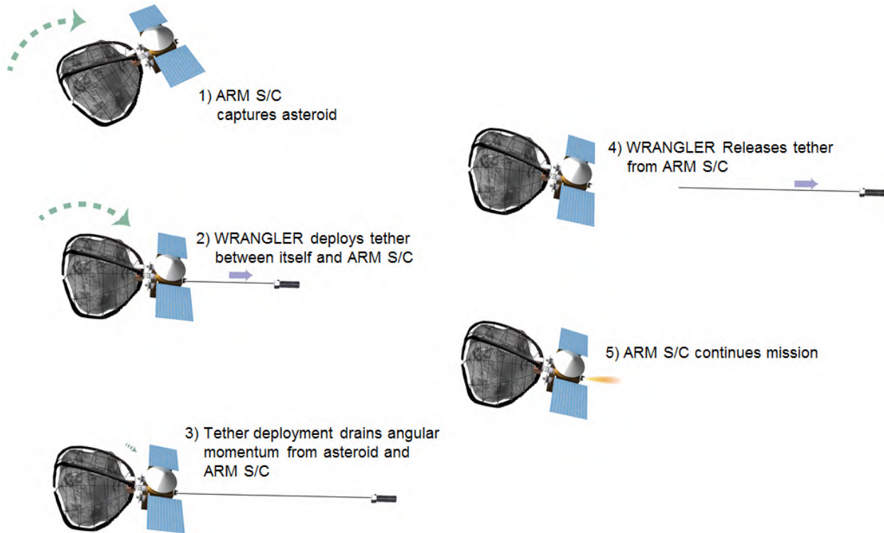
Figure 5. Deployable WRANGLER CubeSat CONOPS. WRANGLER can be integrated into existing ARM architectures to enable significant mass savings .
