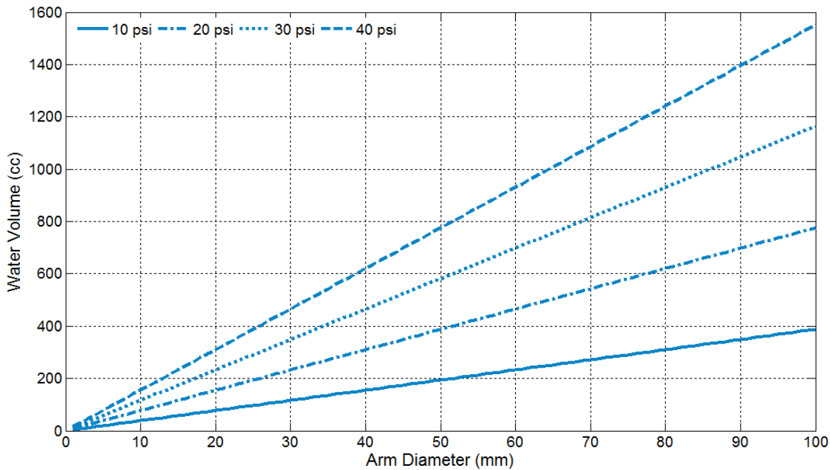
Figure 23. Water Requirements for HYDROS inflation of GRASP. HYDROS provides a mass and volumetrically efficient way to generate gas for inflation of GRASP.
