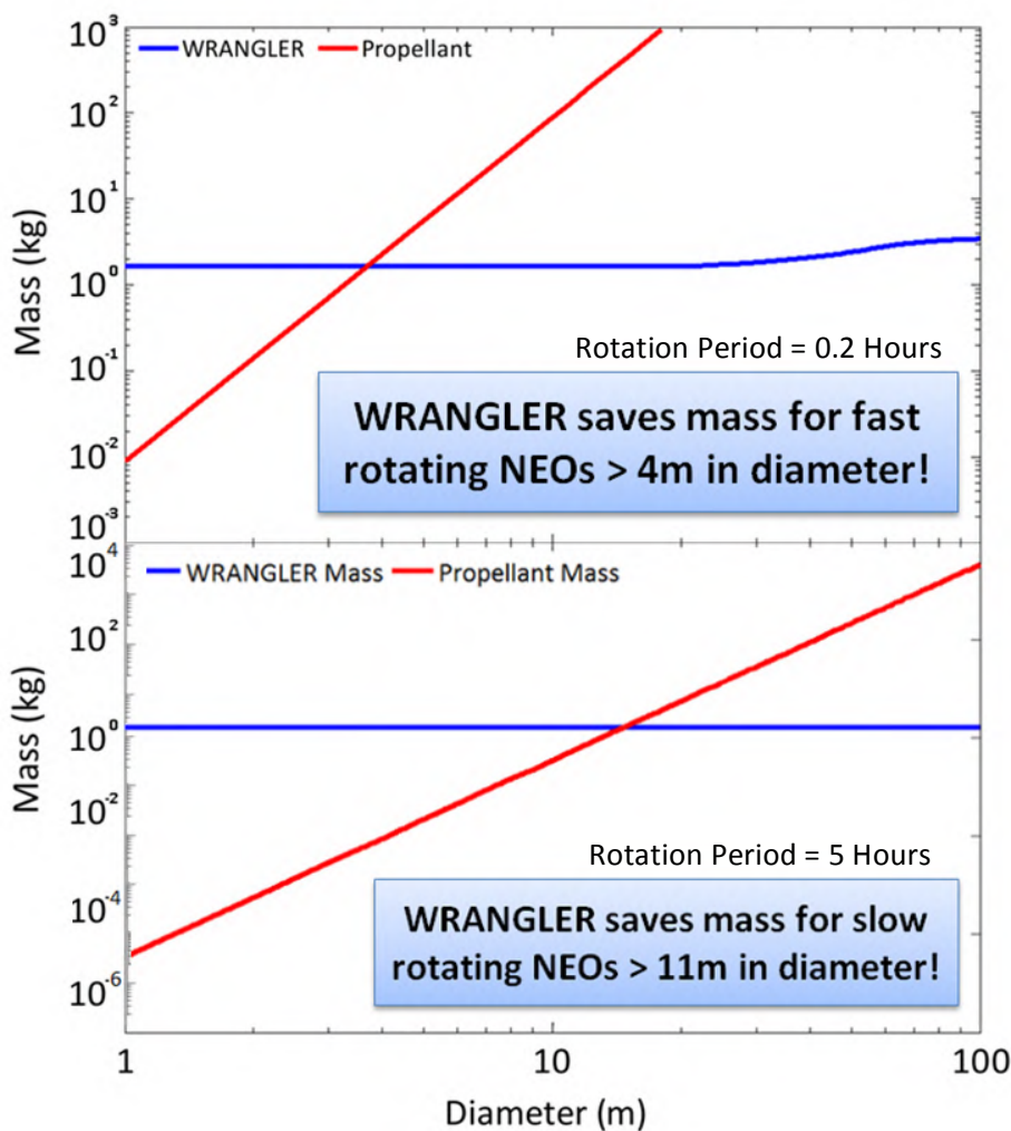
Figure 25. Comparison between a tethered WRANGLER system and the mass of propellant required to de-spin a target. WRANGLER reduces de-spin mass requirement by orders of magnitude for large fast and slow rotators.
