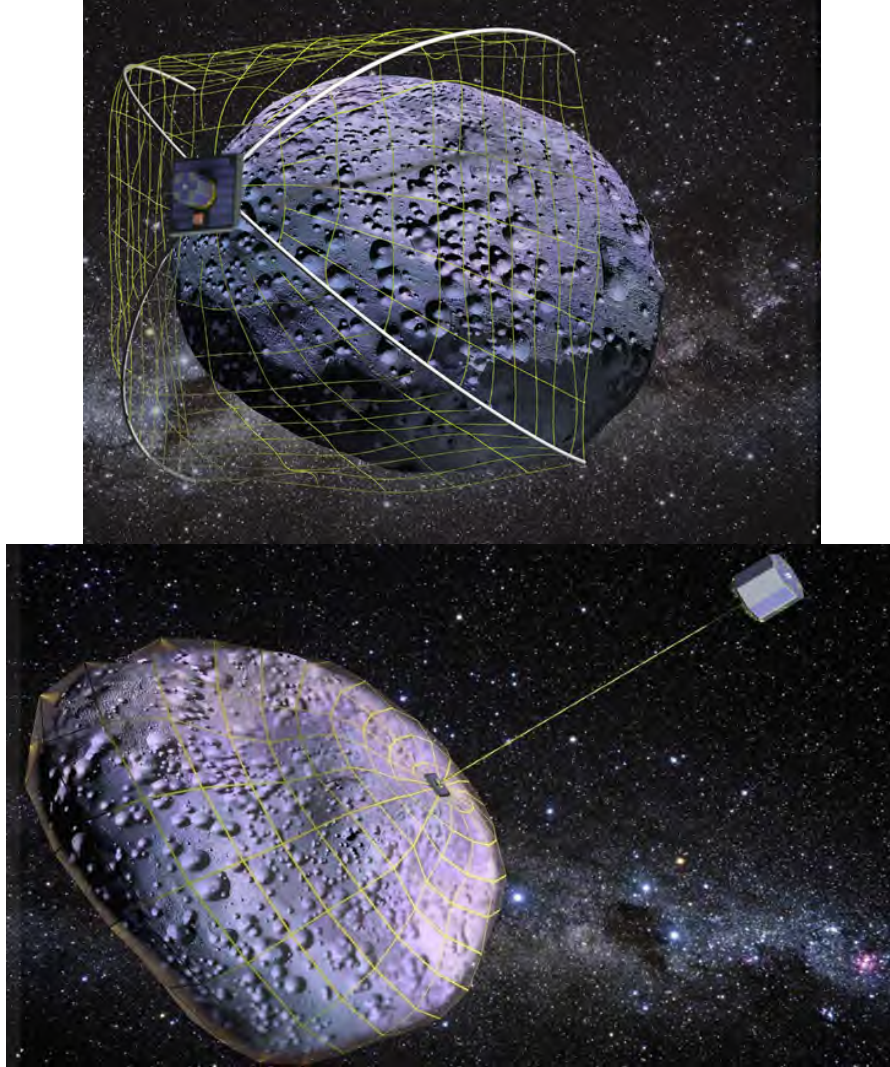
Figure 2. Free-Flying WRANGLER Capturing and De-spinning an Asteroid. WRANGLER attaches itself to a rotating asteroid and then uses a lightweight tether to drain angular momentum from the object, enabling a tiny, low-mass nanosatellite to de-spin a massive asteroid.
