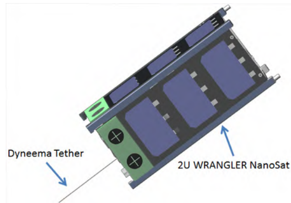
Figure 3. WRANGLER CubeSat Concept. A tethered CubeSat can dramatically reduce the mass required for ARM to de-spin its target object.
