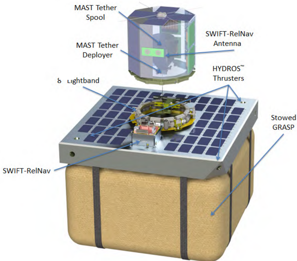
Figure 19. Free-flying WRANGLER Conceptual Design.
