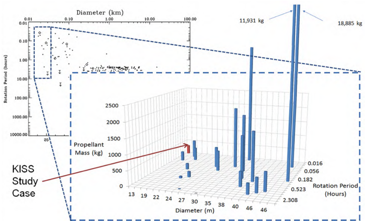
Figure 24. Propellant Required to De-Spin NEOs. The majority of NEOs feasible for near future recovery require massive amounts of propellant to de-spin.
