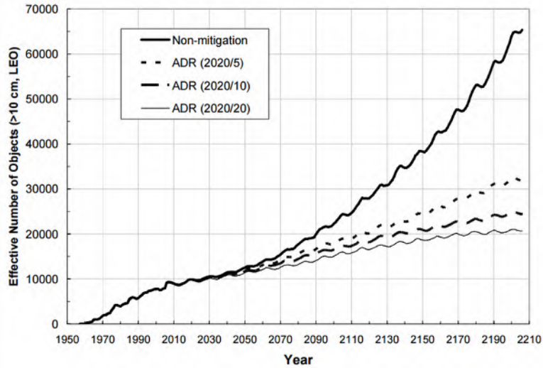
Figure 6. Effectiveness of ADR Missions. Removing as few as 5 objects a year can have a significant impact on the projected orbital debris population.
