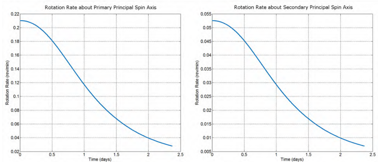
Figure 13. Successful WRANGLER De-Tumble of Asteroid Spinning about Two Principle Axes of Rotation.
