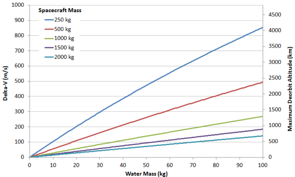
Figure 27. HYDROS Deorbit Performance Across a Range of Target and Water Masses. Small ADR systems utilizing the HYDROS thruster
