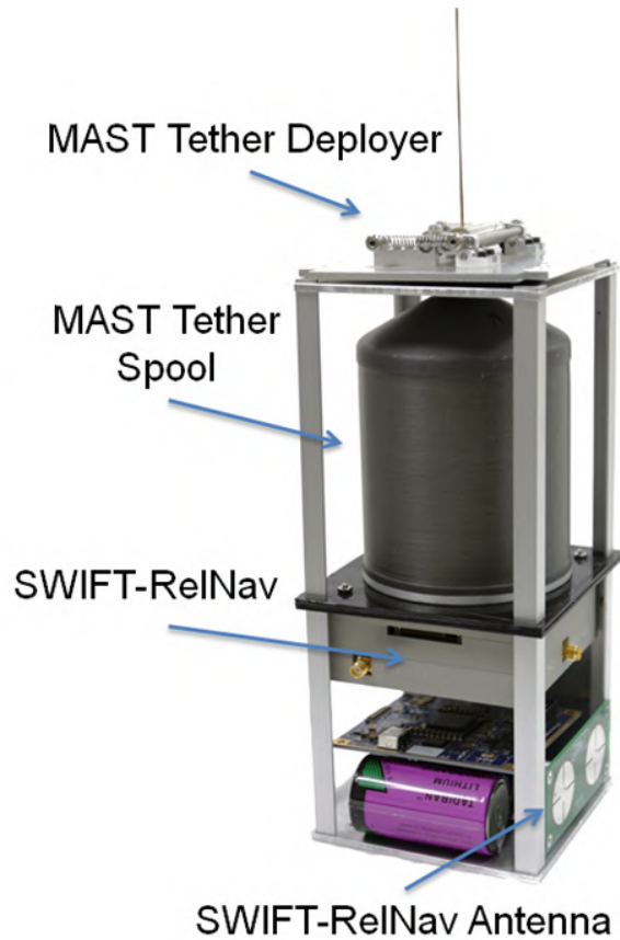
Figure 16. Photo of WRANGLER 2U Mock-Up. The 2U WRANGLER design integrates existing high TRL, flight qualified technologies.
