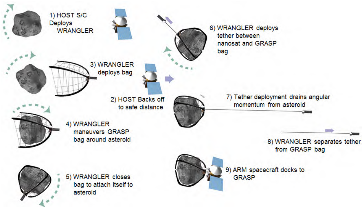
Figure 4. Free-Flying WRANGLER CONOPS. Utilizing TUI’s GRASP technology WRANGLER can de-spin massive asteroids with a low mass nanosatellite scale system ahead of primary ARM spacecraft.
