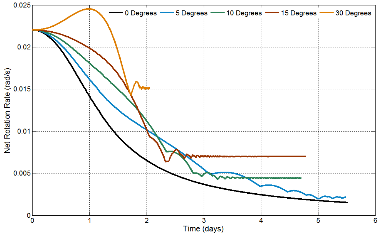
Figure 11. Effect of Off-Axis Tether Attachment. WRANGLER must be attached at the equatorial spin axis of the target in order to conduct the most effective de-spin.
