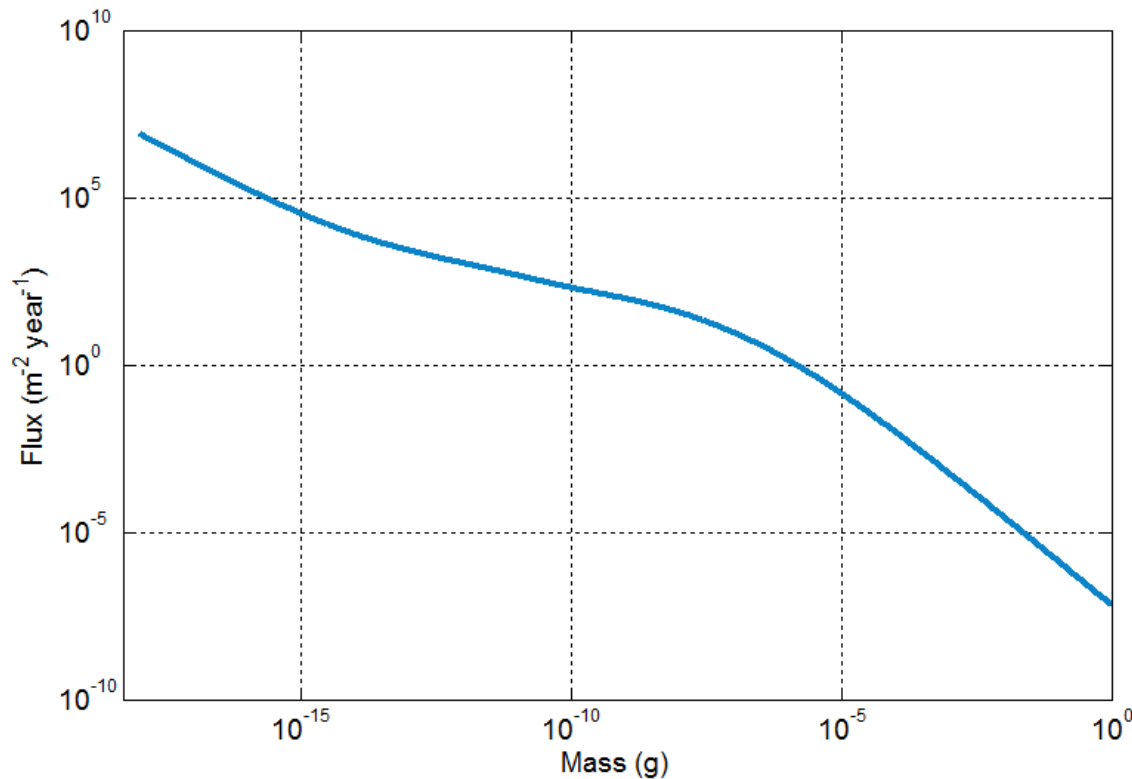
Figure 29. Grün Interplanetary Micrometeoroid Cumulative Flux.
