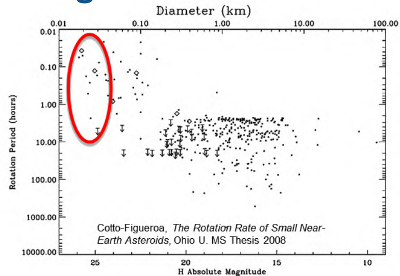
NEA Population. Most small NEAs are “fast rotators”.
