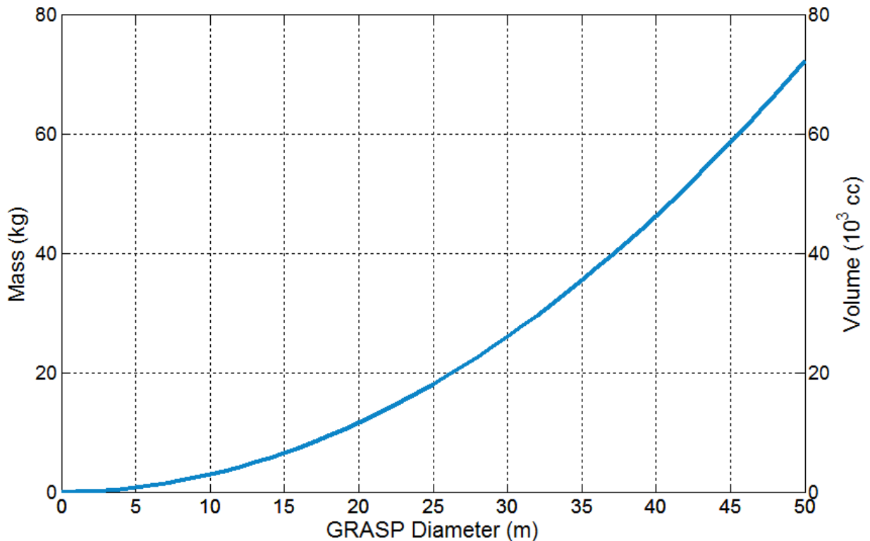
Figure 21. GRASP Sizing with a thin-film bag. GRASP can be readily scaled for asteroid retrieval or ADR missions.
