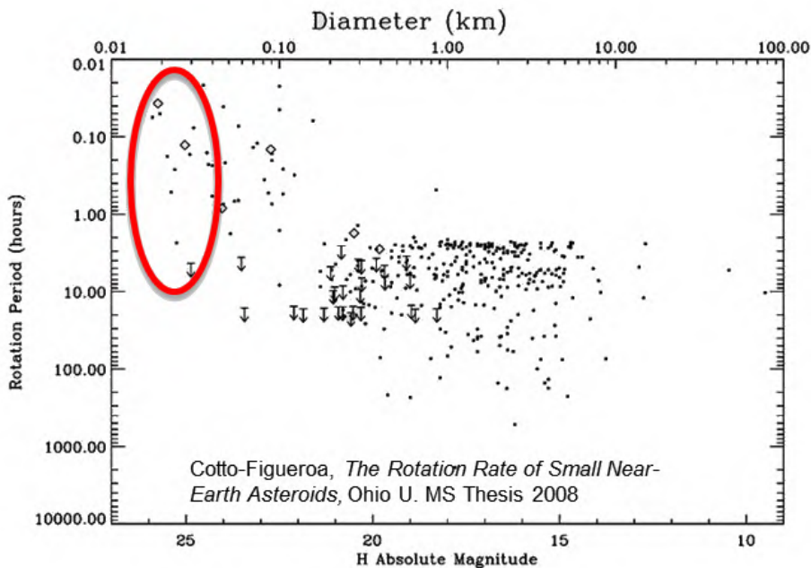
Figure 1. NEA Population rotation periods vs. size. 1 Most small NEAs are “fast rotators.”
