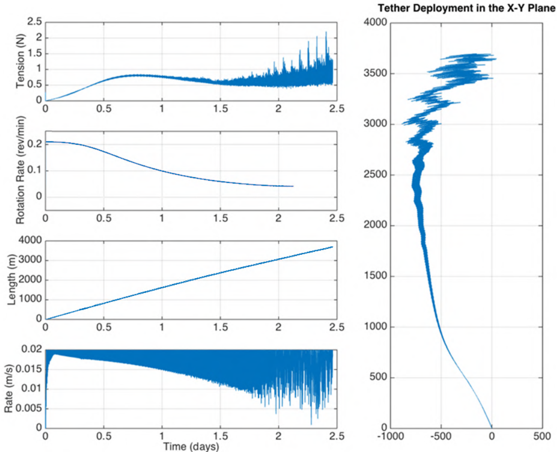
Figure 10. Successful WRANGLER Deployment From a 1000t Asteroid Rotating at 0.22 RPM. WRANGLER can effectively de-spin asteroids without incurring unwanted tether dynamics.
