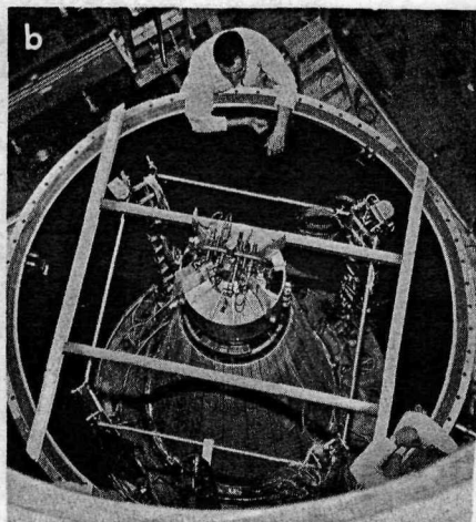
Figure 4 (a) SNAP-10A in orbit. It functioned successfully. (See cover.) (b) This earthbound counterpart generated electricity continuously under simulated space conditions for more than a year.
