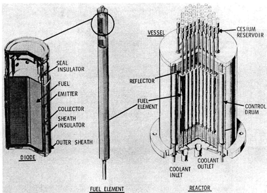
Figure 25 Thermionic diodes (left) can be assembled like flashlight batteries in long fuel elements (center). The elements are then arranged to make a reactor core as shown on the right.
