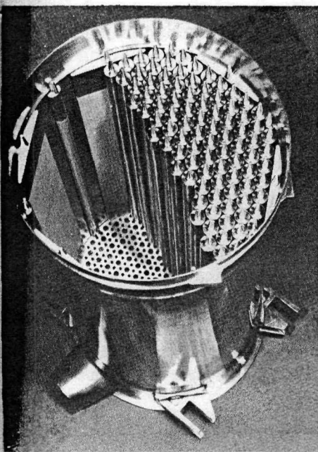
Figure 12 The SNAP-2 reactor. Movable reflector pieces vary the rate of power production.
