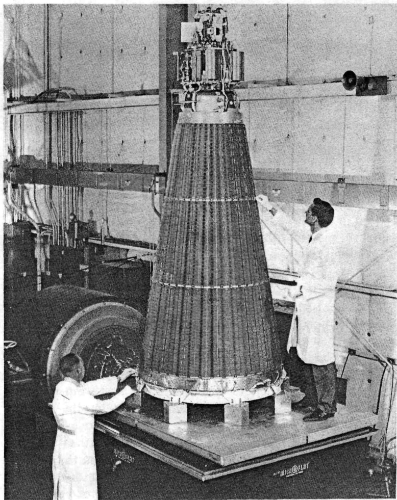
Figure 19 The complete SNAP-10A power plant showing the reactor perched on top of the conical radiator-thermoelectric element assembly (also shown on the cover). A rocket launch shroud surrounded this power plant during the launch period, but was blown off with explosive bolts once the reactor was in orbit.
