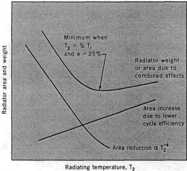
Figure 18 Sketch showing qualitatively how increasing the temperature ( T_2 ) decreases radiator area on one hand due to the Stefan-Boltzmann Law, but increases it on the other due to loss of cycle efficiency, as described by the Carnot efficiency equation. ( T_1 is assumed to be constant.)
