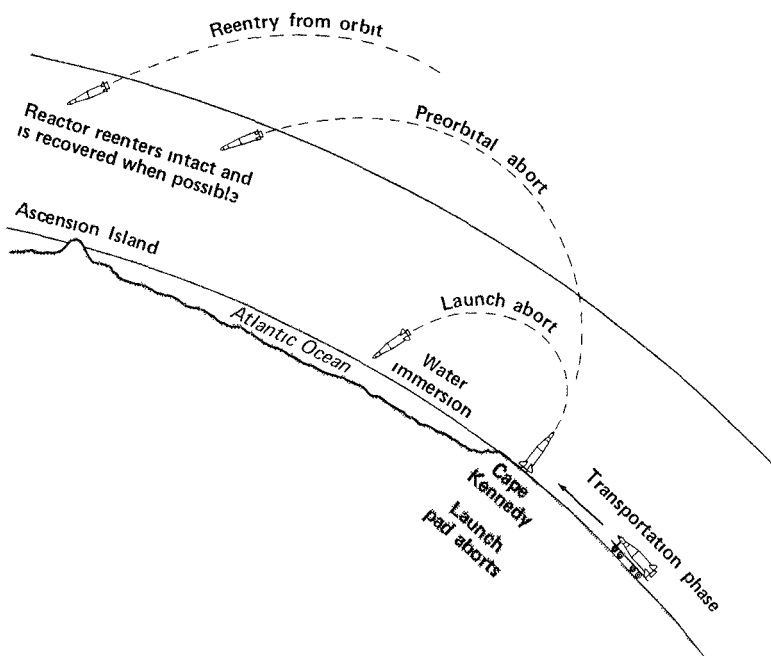
Figure 22 Possible accidents and situations that nuclear safety engineers must anticipate to guarantee safety.
