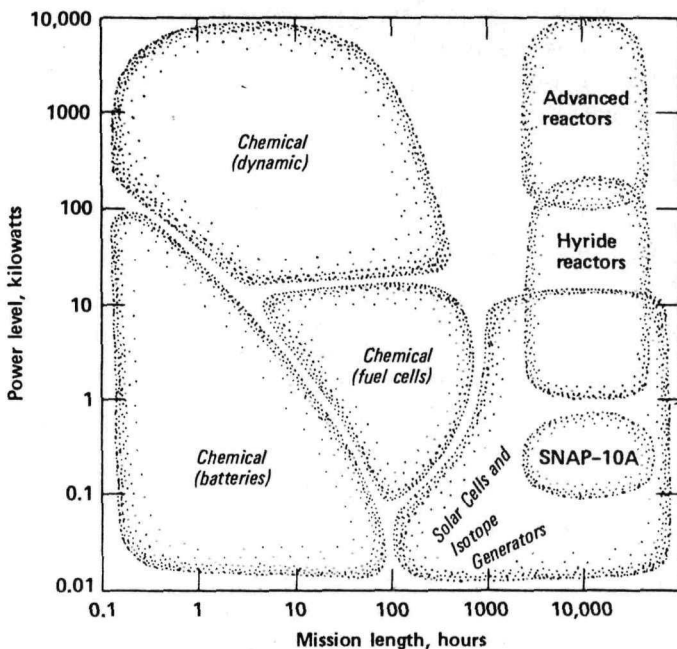
Figure 6 Areas of superiority for various space power plants. Generally, the higher the power level and the longer the mission, the greater the superiority of nuclear reactor power. Superiority on this chart means least weight.
