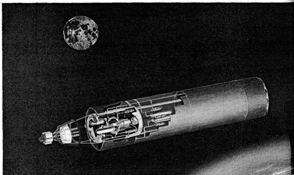
Figure 20 Artist's conception of a SNAP-50 power plant as it would appear in earth orbit.
