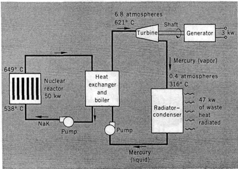
Figure 15 Schematic diagram of SNAP-2 nuclear power plant.
