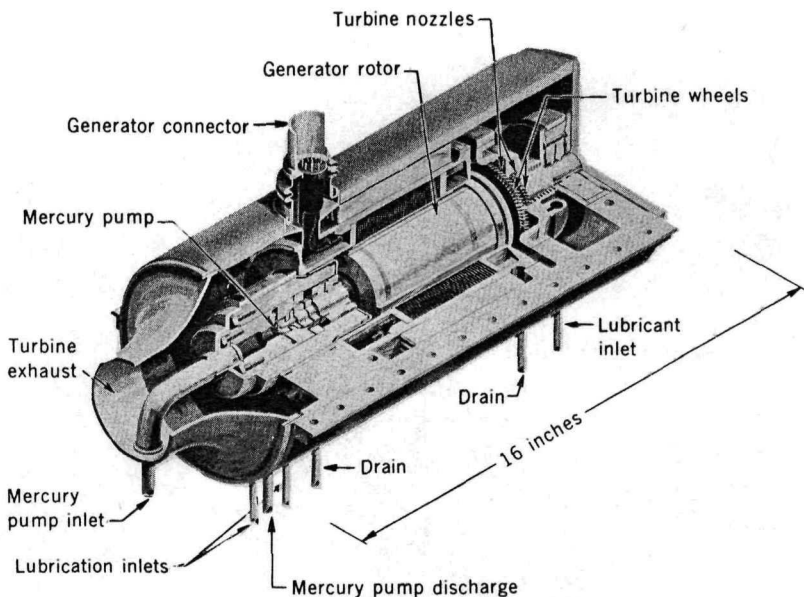
Figure 16 Combined turbine-generator-pump unit.
