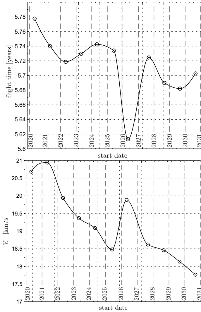
Figure 1: Top: minimum flight time from Earth to Uranus for launch year in 2020-2030. Bottom: the corresponding hyperbolic excess speed V_{\infty} .
