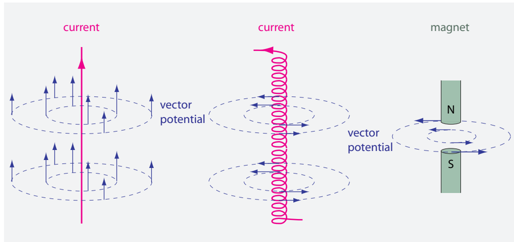
FIGURE 39 Vector potentials for selected situations.
