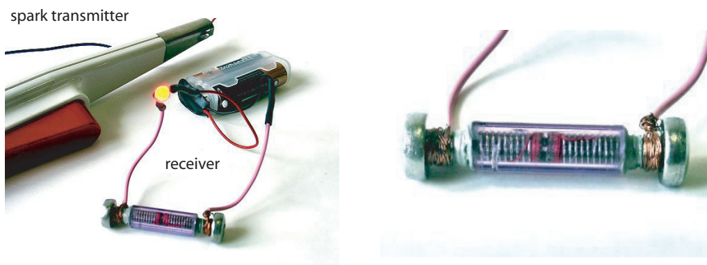
FIGURE 48 The simplest radio transmitter possible, a gas lighter and a wire, together with the simplest receiver possible, built from a battery pack, a light emitting diode, and a simple coherer made from a ball pen housing, two screws and some metal powder (© Guido Pegna).
