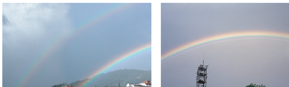
FIGURE 49 The primary and secondary rainbow, and the supernumerary bows below the primary bow (© Antonio Martos and Wolfgang Hinz).
