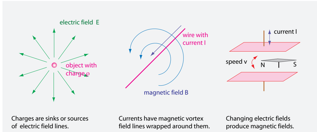
FIGURE 36 The first of Maxwell's field equations of electrodynamics illustrated in three drawings.
