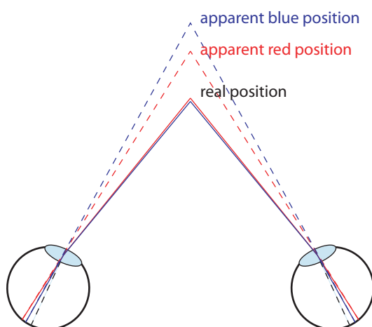
FIGURE 122 The relation between the colour depth effect and the lens dispersion of the human eye.
