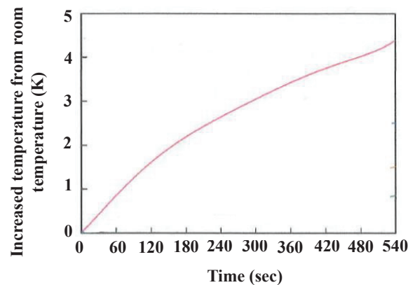
Fig. 4 Temporal change in temperature of the LiNbO 3 crystal during pulse UV laser irradiation.
