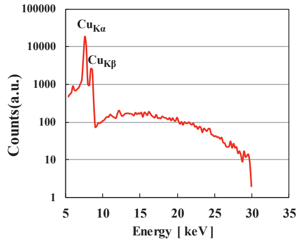
Fig. 2 X-ray spectrum generated by using a Cu target and a LiNbO 3 crystal excited by a pulse UV laser.
