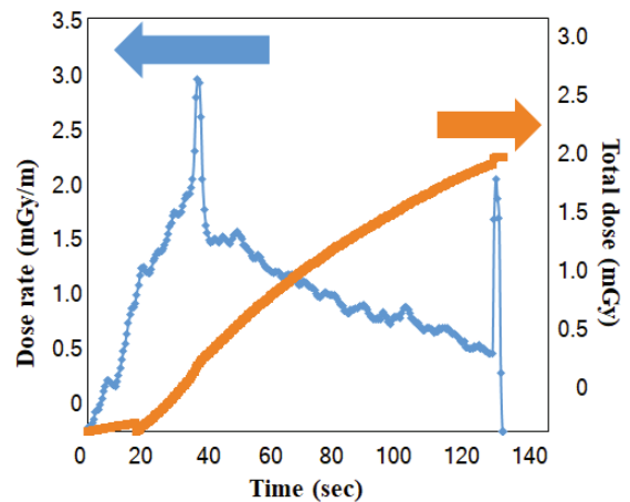
Fig. 3 Temporal response of the X-ray generation excited by 266 nm UV light. (a) and (b) indicate a dose rate and a total dose, respectively.
