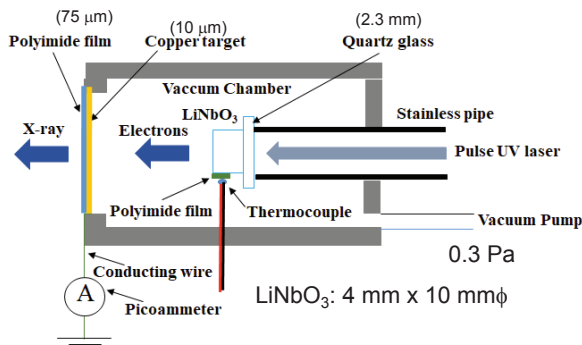
Fig. 1 Experimental setup of the X-ray source
