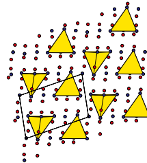
\text{Tb}_{11}\text{O}_{20} ( \delta 1 )
