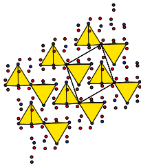
\text{Pr}_7\text{O}_{12} ( \iota )
