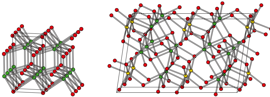
Figure 3-16. Structures of A-type (left) and B-type (right) sesquioxides of the lanthanoids projected almost along the common axis. Metals green (seven-coordinated) and yellow (six-coordinated), oxygens red.
