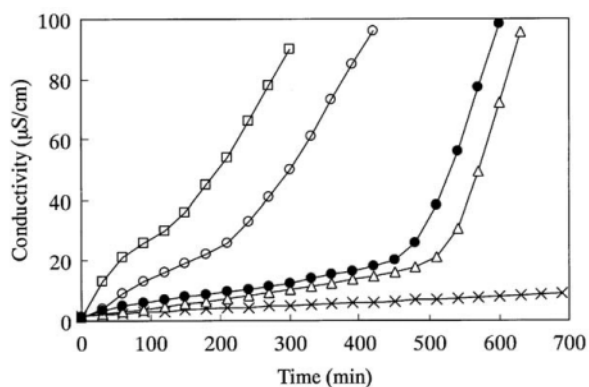
Figure 9-34. Evaluation of the catalytic activity at 120°C. ×: blank (without catalyst), □: undoped CeO 2 , Δ: 20mol% Ca 2+ -doped CeO 2 , ●: 20mol% Zn 2+ -doped CeO 2 , and ○: 30 mol% Eu 3+ -doped CeO 2 . (Reprinted with permission from ref 53. Copyright 2003 Elsevier Science)
