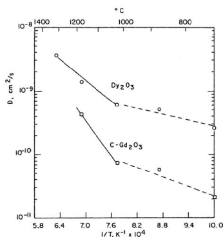
Figure 5-4. Temperature dependence of oxygen diffusion coefficients ( P_{O_2} > 10^{-10} atm) in Dy 2 O 3 and cubic (C-type) Gd 2 O 3 . (Reproduced with permission from ref. 7. Copyright 1974 American Ceramic Society.)
