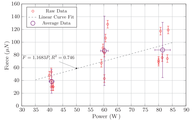
Fig. 19 Graph of forward and reverse thrust vacuum testing.
