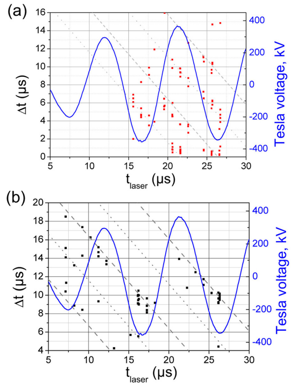
FIG. 5. \Delta t as a function of t_{\text{laser}} for L = 50 cm (a) and L = 100 cm (b) (scatter plots). The oblique lines represent the time position of positive (dotted lines) and negative (dashed lines) Tesla voltage peaks. The evolution of the Tesla voltage (blue solid line) in time is also given for convenience.
