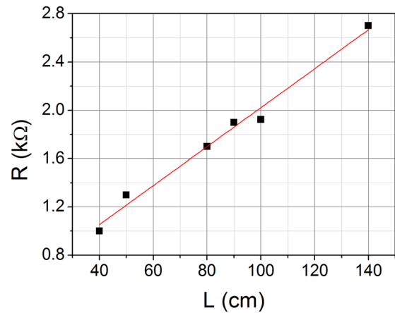
FIG. 8. Evolution of the operational resistance R with the gap length L (scatter plot) and linear fit (red solid line). Only breakdown occurring in the voltage range -360 \text{ kV} < U_{bd} < -300 \text{ kV} was taken into account.
