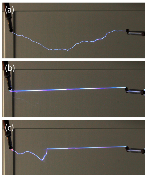
FIG. 3. Time-integrated images of spark discharges: without any apparent guiding (a), fully guided (b), and partially guided by the laser filament (c). The laser pulse comes from the left and the gap length is fixed to 32 cm.
