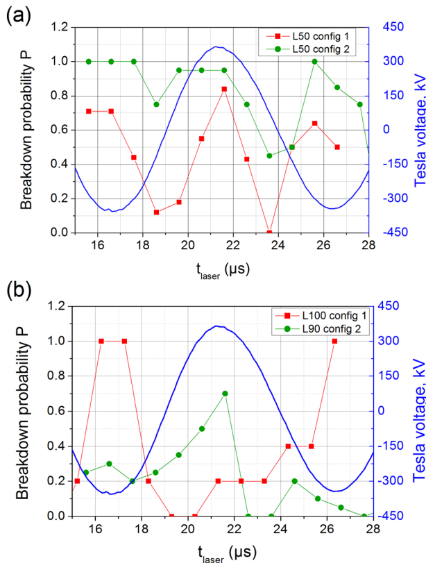
FIG. 4. Evolution of the breakdown probability P with t_{\text{laser}} . (a): L = 50 cm, configuration 1 (red solid curve and squares) and configuration 2 (green solid curve and circles). (b) L = 100 cm, configuration 1 (red solid curve and squares) and L = 90 cm, configuration 2 (green solid curve and circles).
