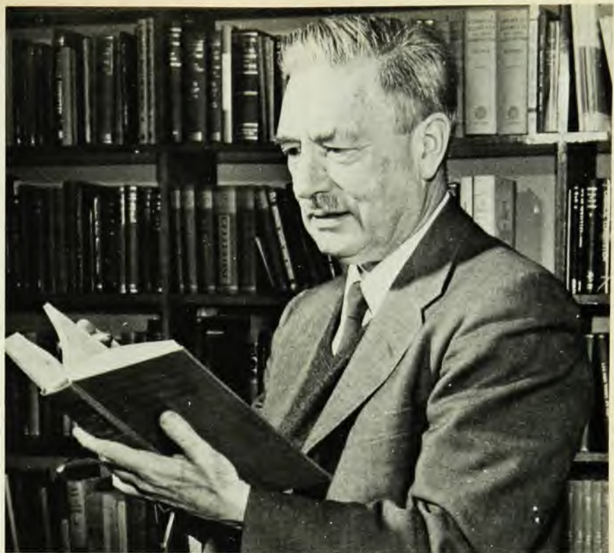
DEBYE
