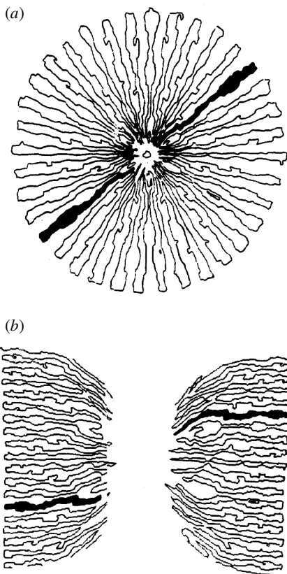
Figure 6. Action of the retinocortical map on the funnel form constant. (a) Image in the visual field; (b) V1 map of the image.
