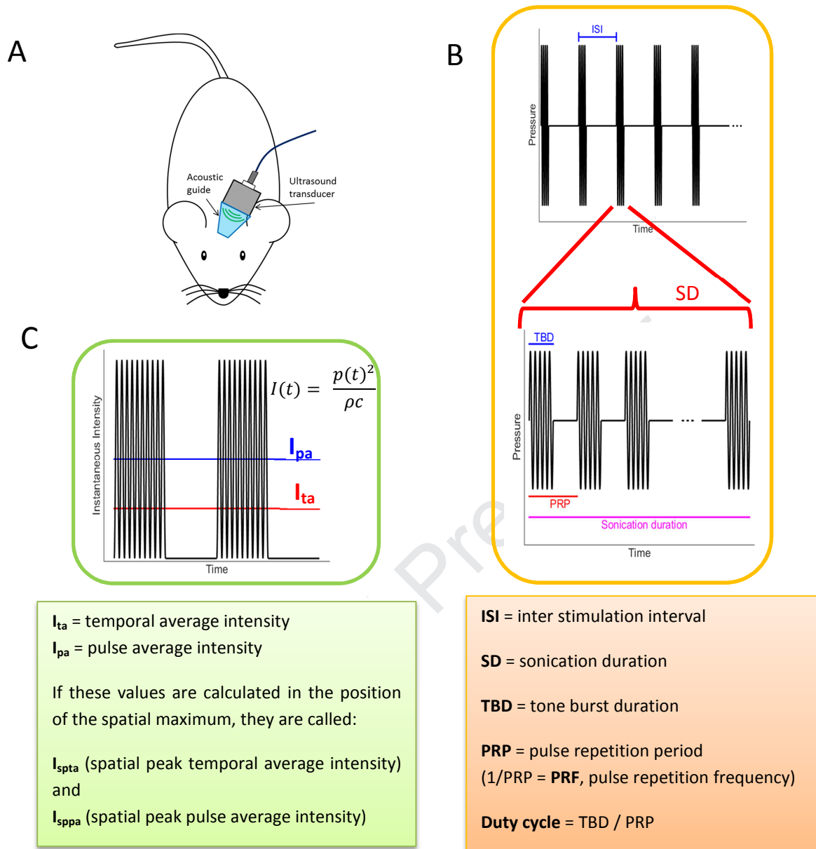
Figure 2: Overview of the TFUS setup and parameters. A) The ultrasound pressure wave is generated by a transducer and delivered to the target through a guide filled with acoustic gel. B) The pressure stimulus over time is shown to indicate the main parameters. C) The main intensity values are shown for a fixed space position, together with their relationship with the pressure signal.
