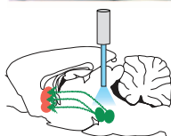
Stimulation of dopamine neurons
