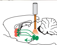
Silencing of dopamine neurons
