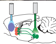
Top-down control of striatal dopamine signaling
