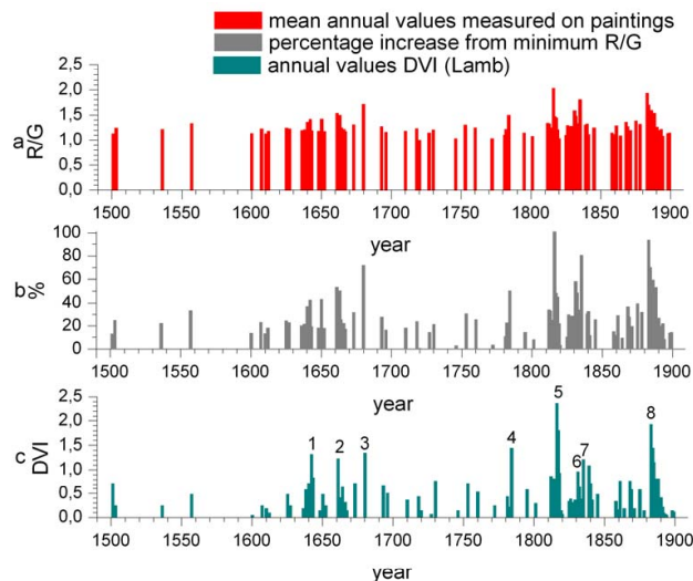
Fig. 2. (a) The mean annual value of R/G measured on 327 paintings. (b) The percentage increase from minimum R/G value shown in (a). (c) The corresponding Dust Veil Index (DVI). The numbered picks correspond to different eruptions as follows: 1. 1642 (Awu, Indonesia-1641), 2. 1661 (Katla, Iceland-1660), 3. 1680 (Tongkoko & Krakatau, Indonesia-1680), 4. 1784 (Laki, Iceland-1783), 5. 1816 (Tambora, Indonesia-1815), 6. 1831 (Babuyan, Philippines-1831), 7. 1835 (Coseguina, Nicaragua-1835), 8. 1883 (Krakatau, Indonesia-1883).
