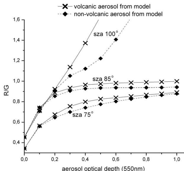
Fig. 4. Nomogram of R/G and aerosol optical depth as resulted from the model for three solar zenith angles calculated for non-volcanic and volcanic aerosols used to calibrate the measurements on paintings.
