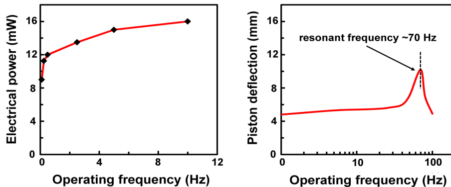
Fig. 8. (left) Lens electrical power consumption (at 160 V) as a function of switching frequency and (right) lens actuators' mechanical displacement as a function of frequency.
