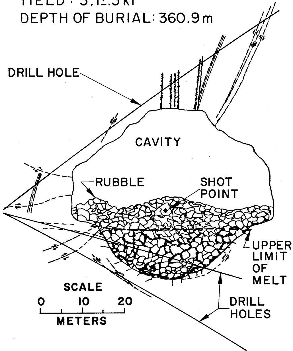
Fig. 8. Gnome cavity profile.
