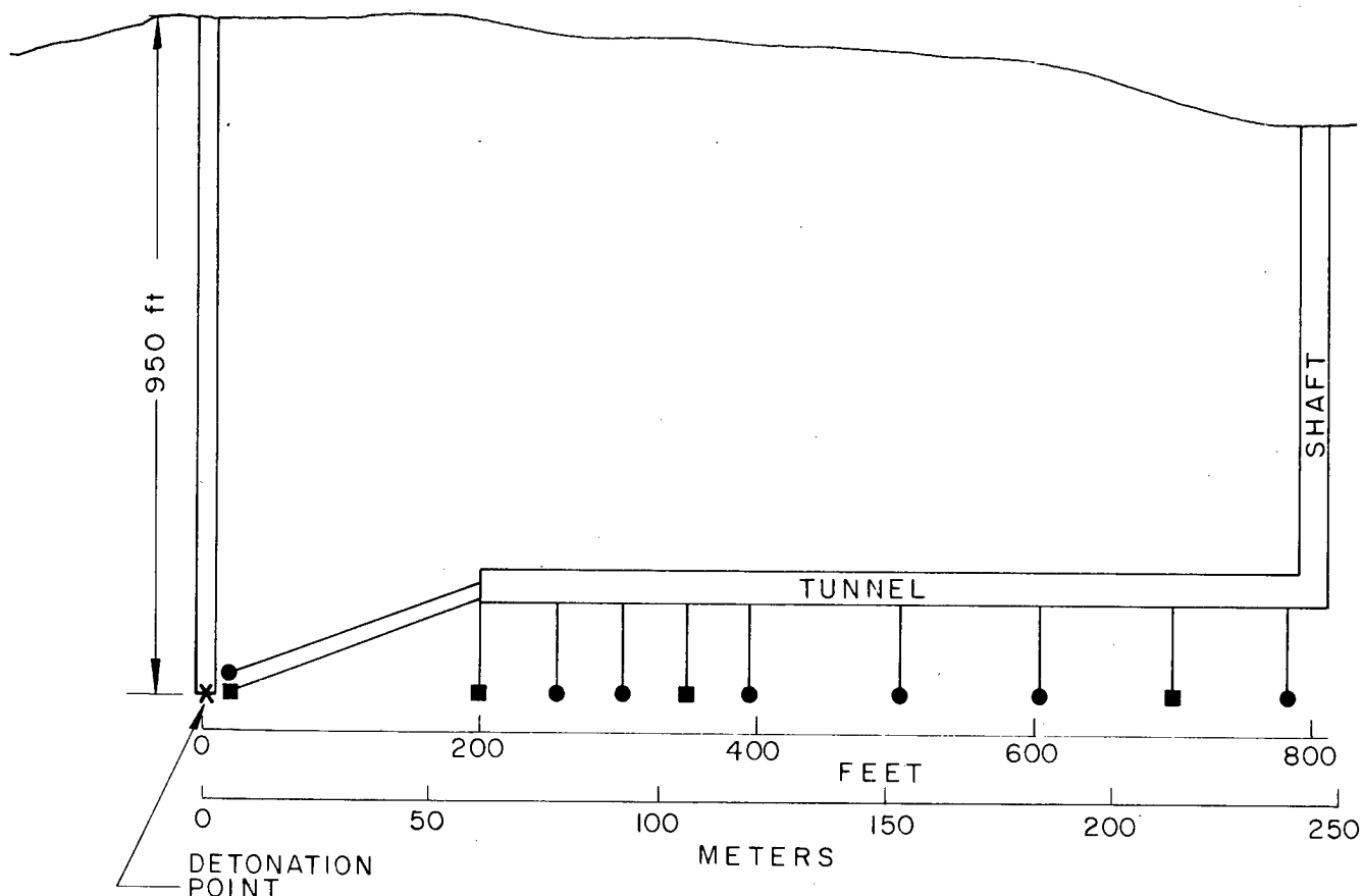
Fig. 1. Layout of instrumentation of Hardhat event.
