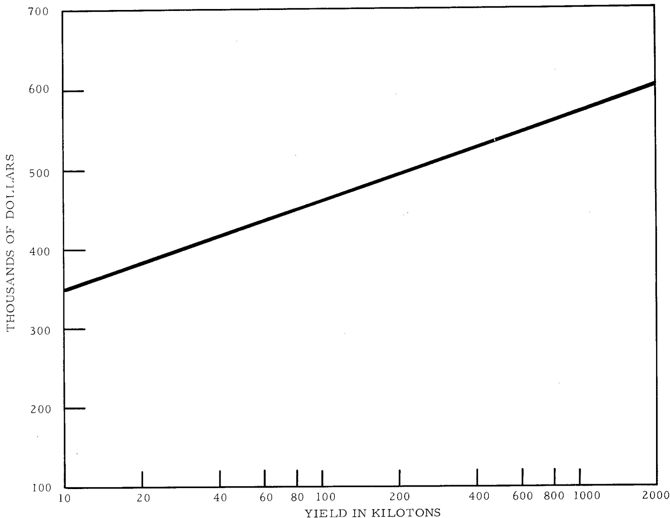
Fig. 1. Projected charges for thermonuclear explosives.
