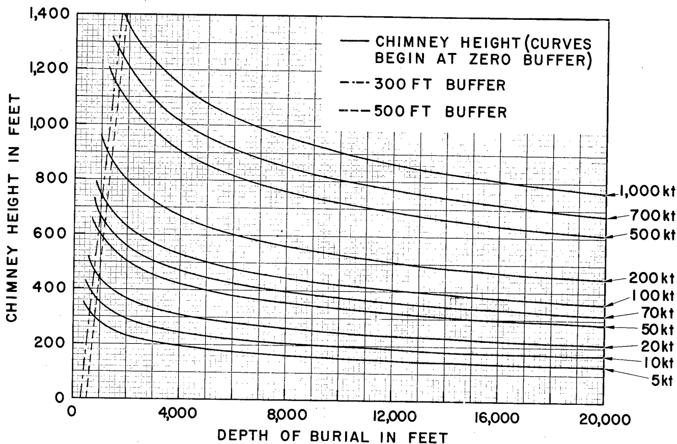
Fig. 3. Chimney height for underground nuclear explosions in granitic rock.
