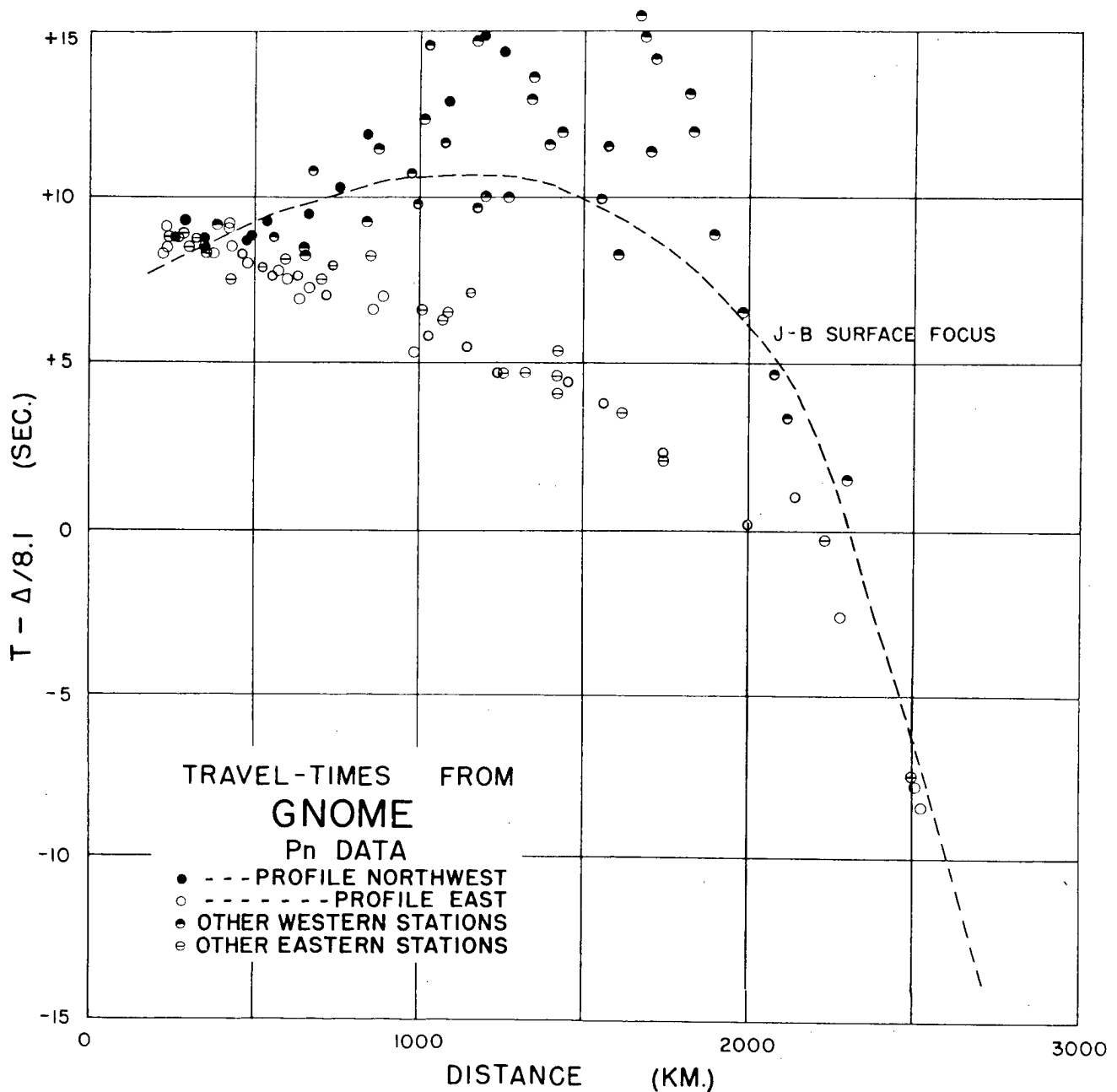
Fig. 4. Reduced travel times for P-waves from Gnome by profiles.
