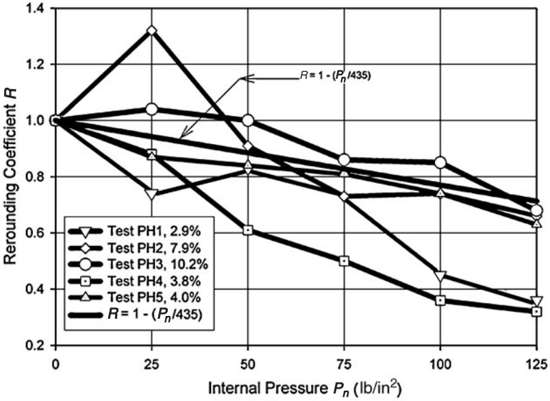
Figure 4.21 Rerounding coefficient from test data—poor haunch condition.
