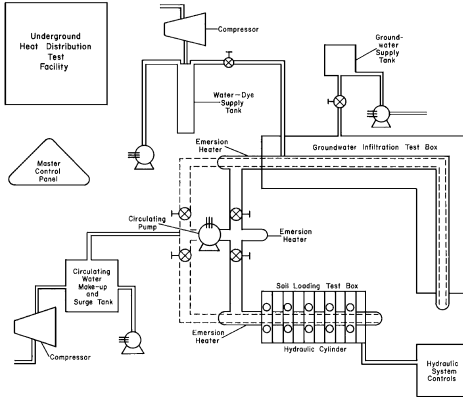
Figure 6.51 Underground heat distribution test facility schematic.
