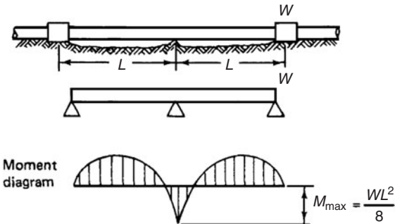
Figure 2.16 Longitudinal bending of conduits.
