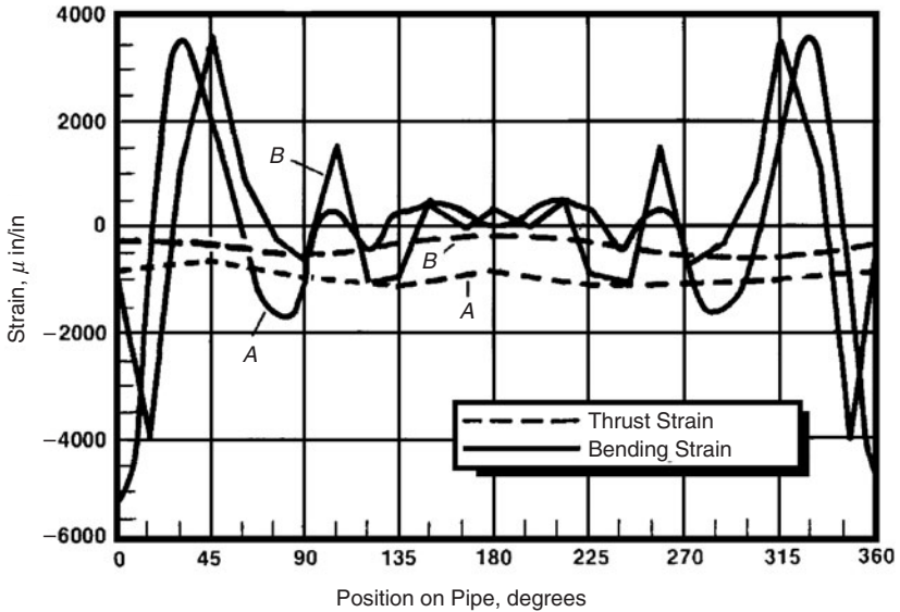
Figure 3.55 Pipe strain as function of circumferential position, conditions as in Fig. 3.54.
