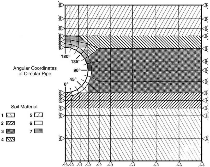
Figure 3.37 Finite element mesh for a buried pipe.
