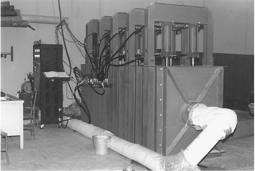
Figure 6.57 Soil load cell showing the insulation used on return piping.
