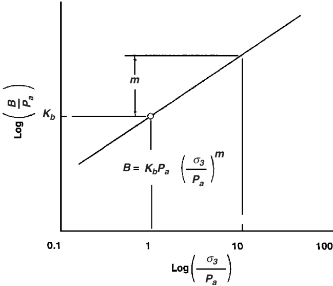
Figure 3.41 Variation of bulk modulus with confining pressure. (After Duncan et al. 6 )
