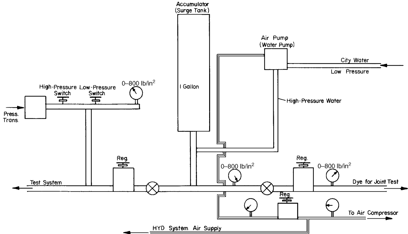
Figure 6.54 Schematic of pressure controls.
