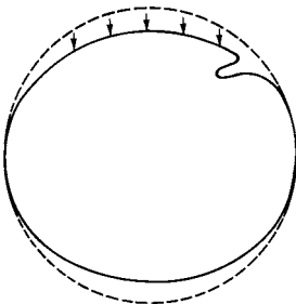
Figure 3.22 Localized wall buckling.
