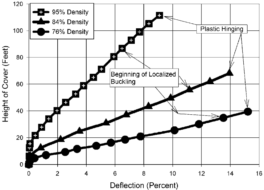
Figure 6.19 Vertical deflection for the three tests in silty-sand soil at various densities.
