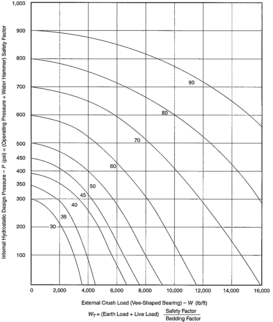
Figure 4.5 Combined loading curves for 24-in asbestos-cement pressure pipe. (Reprinted, by permission, from ANSI/AWWA C403-98. 2 Copyright © 1998, American Water Works Association.)
