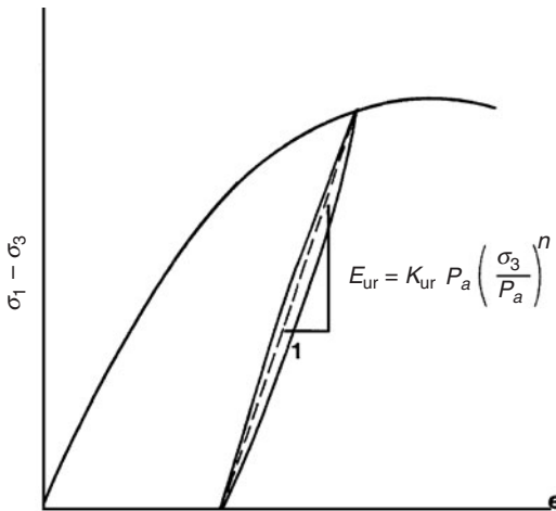
Figure 3.43 Unloading-reloading modulus. (After Duncan et al. 6 )
