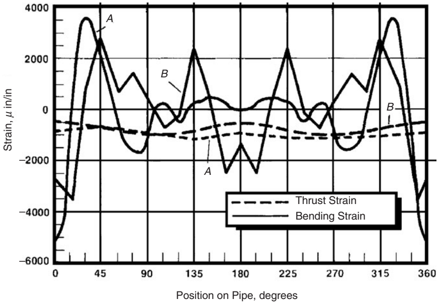
Figure 3.57 Pipe strain as a function of circumferential position, conditions as in Fig. 3.56.
