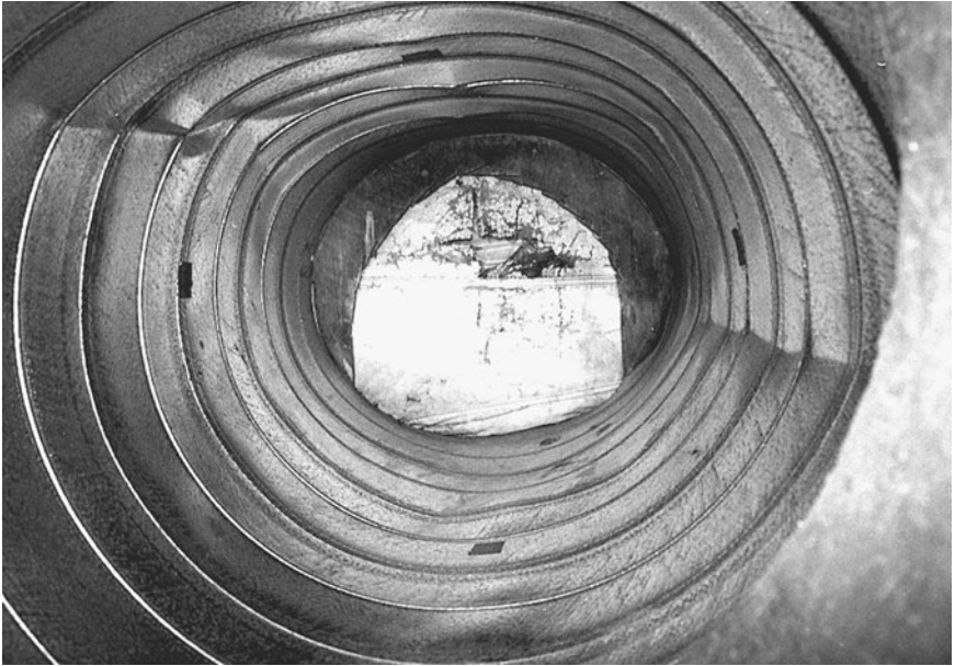
Figure 6.17 Inside pipe at completion of test 3. The cover height is 110 ft.
