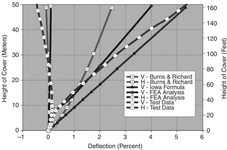
Figure 3.32 Comparison of test results with various analytical methods for a 48-in-diameter HDPE pipe buried in silty-sand soil compacted to 97 percent standard Proctor density.
