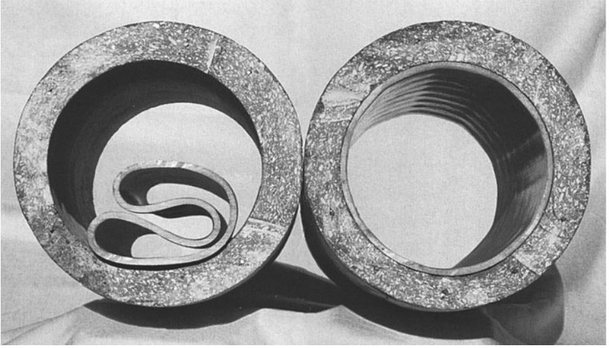
Figure 8.14 Portrayal of the folded pipe as inserted and how it appears after expansion. (Courtesy of Ultraliner.)
