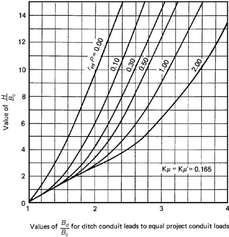
Figure 2.6 Curves for transition-width ratio. (Reprinted, by permission, from Spangler and Handy, Soil Engineering , 4th ed., Harper & Row, 1982.)
