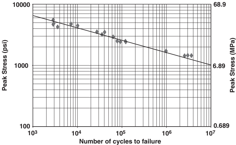
Figure 4.9 Vinson’s data showing failure stress versus number of cycles.
