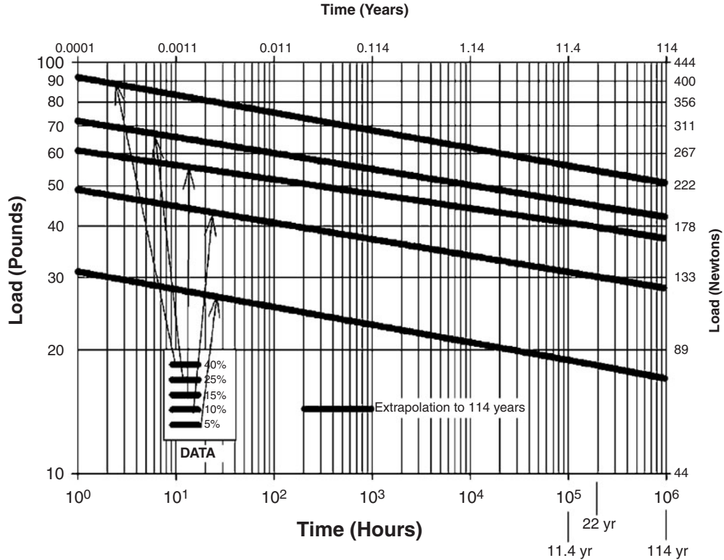
Figure 7.13 Relaxation curves for filled, notched PVC pipe rings at specified deflections and a temperature of 40°F.
