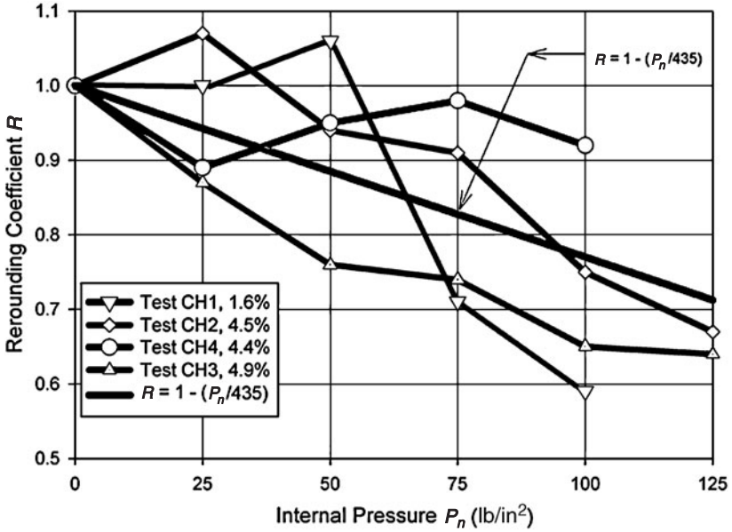
Figure 4.23 Rerounding coefficient from test data—poor haunch condition.
