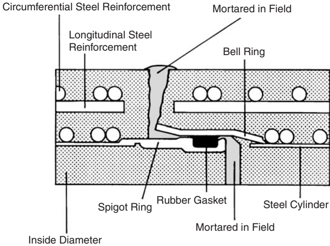
Figure 5.7 Wall cross section of reinforced concrete cylinder pipe. (Reprinted, by permission, from Bulletin No. 200, United Concrete Pipe Corporation. )
