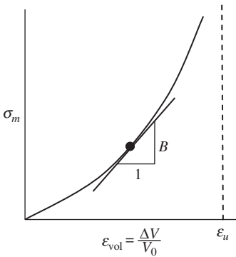
Figure 3.42 Illustration of mean stress versus volumetric strain during a hydrostatic compression test.
