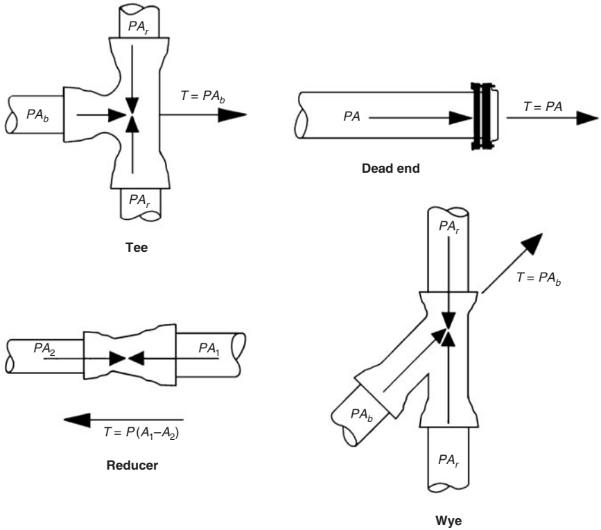
Figure 4.28 Thrust forces. (Reprinted, by permission, from Thrust Restraint Design for Ductile Iron Pipe , Ductile Iron Pipe Research Association.)
