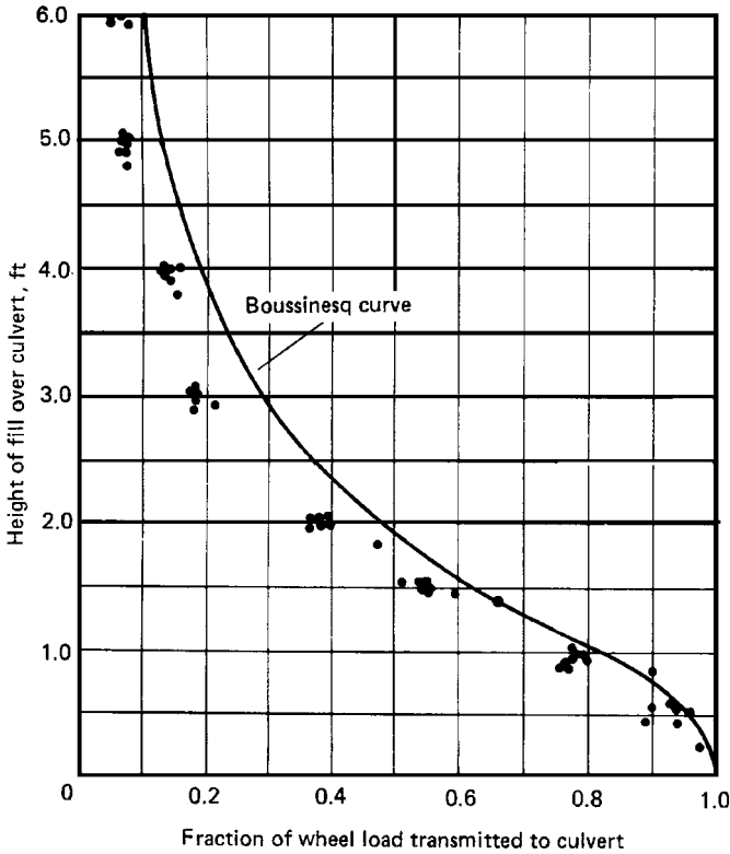
Figure 2.18 Distribution of surface live loads versus loads on a plane at depths of cover. Boussinesq solutions versus actual measurement. (Reprinted, by permission, from Spangler and Handy, Soil Engineering, 4th ed. , Harper & Row, 1982.)
