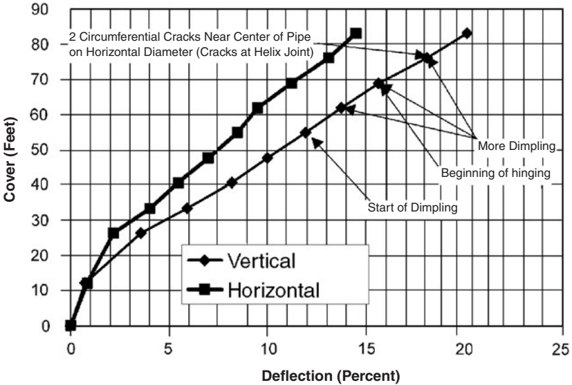
Figure 7.65 Load deflection curves for 42-in-diameter HDPE pipe. Soil is silty sand compacted to 83 percent of standard Proctor density. Measurements are made at center of pipe.
