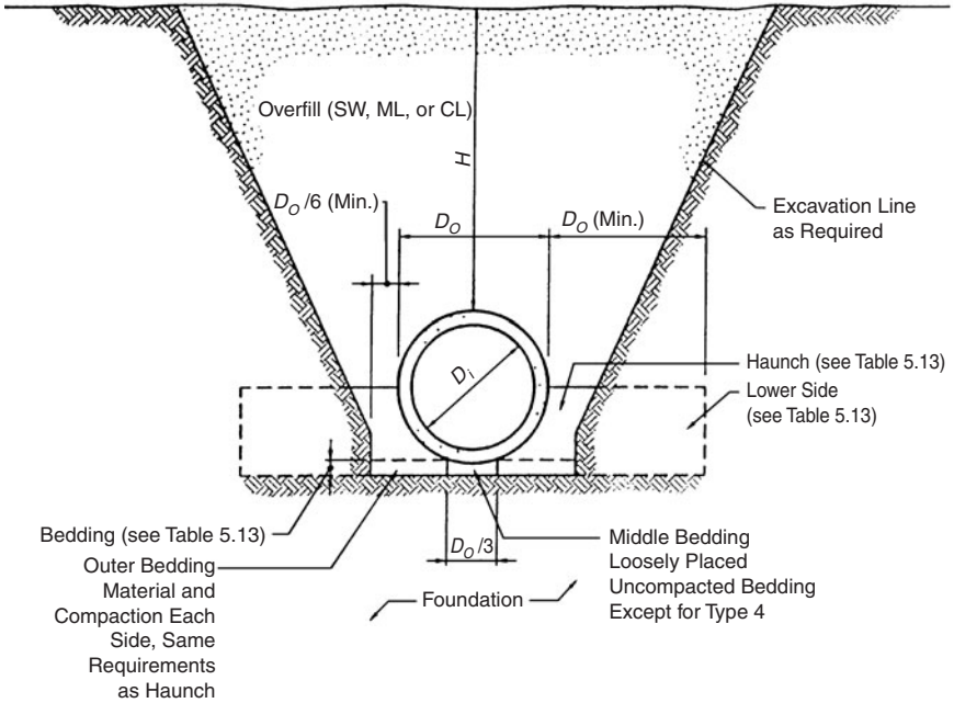
Figure 5.11 Standard trench installations.
