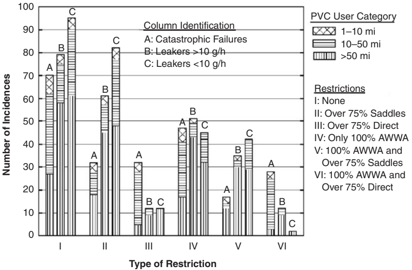
Figure 7.24 Stacked bar graph showing reported tapping problems.
