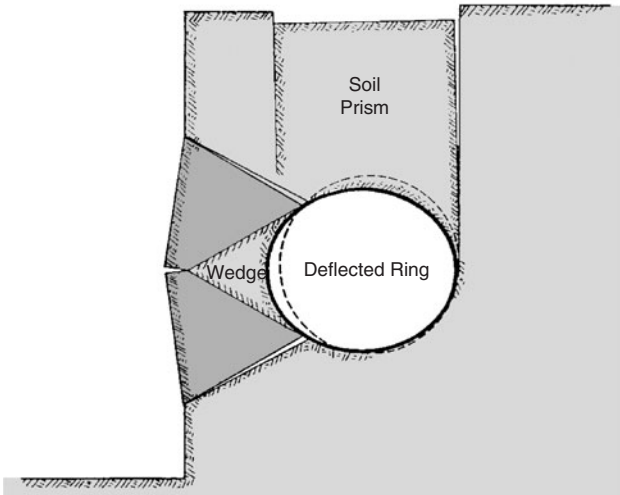
Figure 3.28 Formation of a soil prism on the pipe as a collapse mechanism forms.
