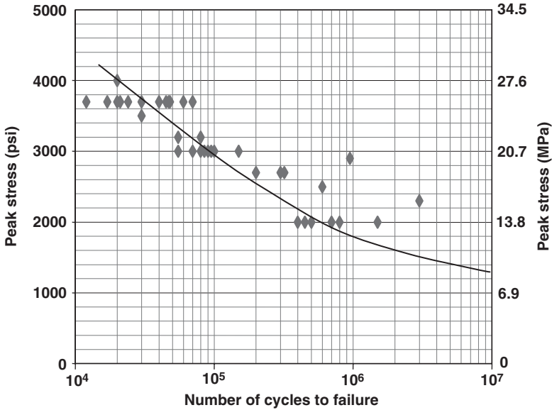
Figure 4.10 Reproduction of Huck’s peak stress data.
