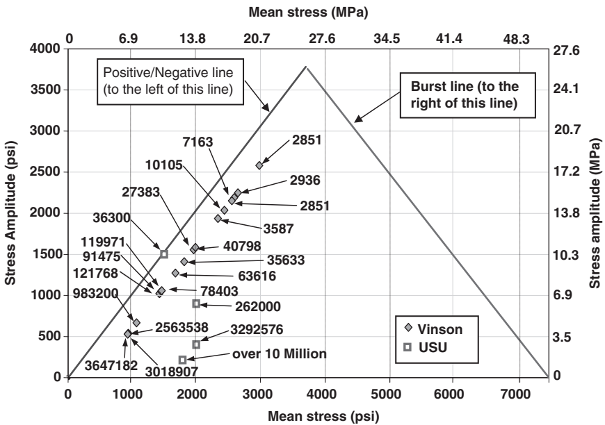
Figure 4.15 Vinson’s (1981) and tests One-Four data. Labels indicate cycles to failure.
