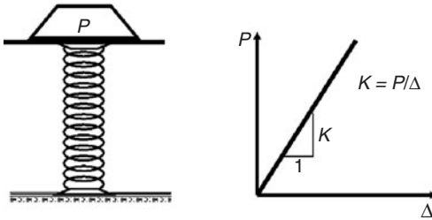
Figure 2.8 Graphic of linear spring.
