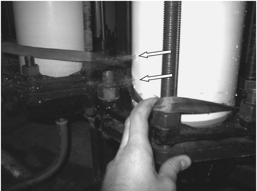
Figure 4.14 The failure of pipe 4 during Test Three.
