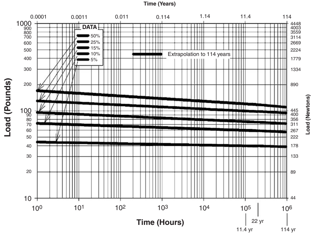
Figure 7.17 Relaxation curves for unfilled, unnotched PVC pipe rings at specified deflections and a temperature of 0°F.
