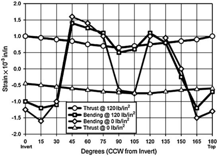
Figure 4.20 FEA rerounding data for pipe buried 20 ft deep in silty-sand soil compacted to 80 percent of Proctor density. Pipe stiffness = 36 lb/in 2 .
