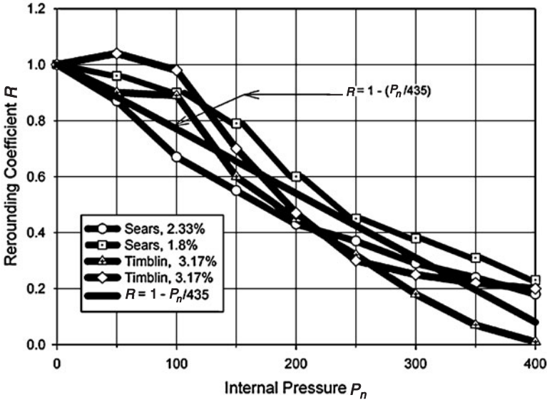
Figure 4.25 Rerounding coefficient from test data on both ductile iron and FRP pipes.
