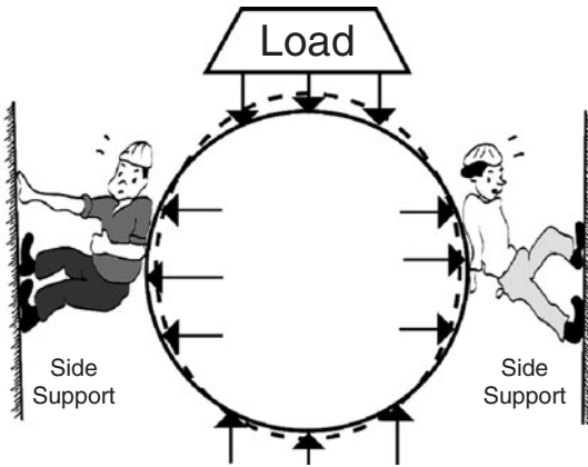
Figure 2.12 Graphic showing the contribution of sidefill soil in the performance of a flexible pipe.
