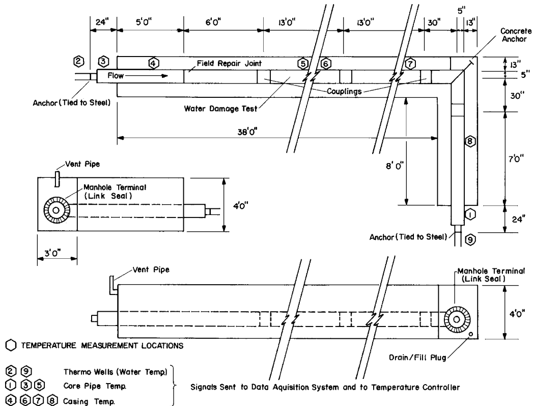
Figure 6.53 Test layout for water damage, water infiltration, and joint leakage tests. This schematic shows the test pipe layout including placement of the following: (1) couplings, (2) field repair joint, (3) concrete anchor on elbow, (4) anchor of pipe protrusion to the test cell, (5) the fitting where dyed water was inserted under pressure for the water damage test, (6) manhole terminals (link seals), and (7) thermocouples for temperature measurement and control.
