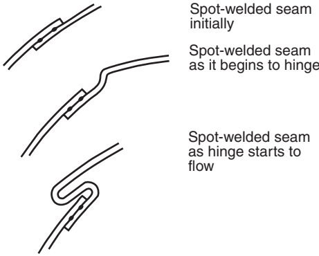
Figure 6.8 Diagrammatic sketch of welded seam showing typical formation of hinge followed by plastic flow.
