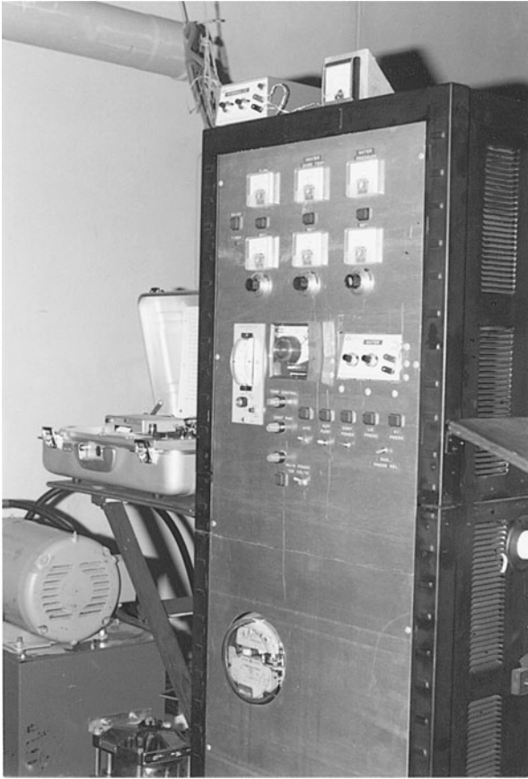
Figure 6.58 System control center with the following features: (1) temperature controller, (2) temperature fail-safe circuits, (3) pressure controls, (4) pressure fail-safe circuits, (5) dual control timer (concealed in photo), (6) flowmeter readout, (7) power meter with digitized output for data system, (8) associated warning lights for system operation. Safety controls were necessary because the system was operated at 500 lb/in 2 and 450°F. An electronically operated pressure relief valve was controlled by the fail-safe circuits. In addition, a manual pressure relief valve was incorporated into the system.
