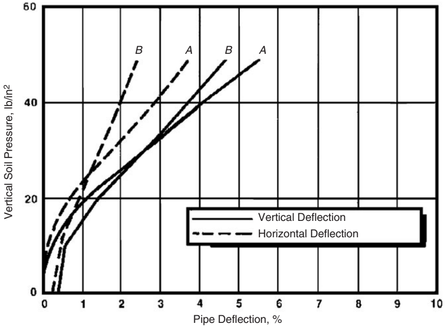
Figure 3.50 Vertical soil pressure versus pipe deflection. (A) Soil test cell data, 90 percent relative compaction; (B) FEA, no compaction simulation.
