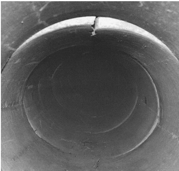
Figure 8.6 The inside of the broken rigid pipe test section after loading to a vertical soil pressure of 5040 lb/ft 2 (equivalent burial depth of 42 ft).
