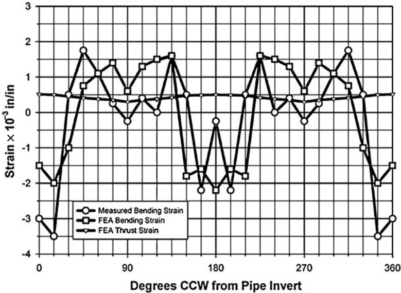
Figure 4.19 Rerounding data for pipe buried 20 ft deep in silty-sand soil compacted to 80 percent of Proctor density. Pipe stiffness = 36 lb/in 2 . Internal pressure is 100 lb/in 2 .
