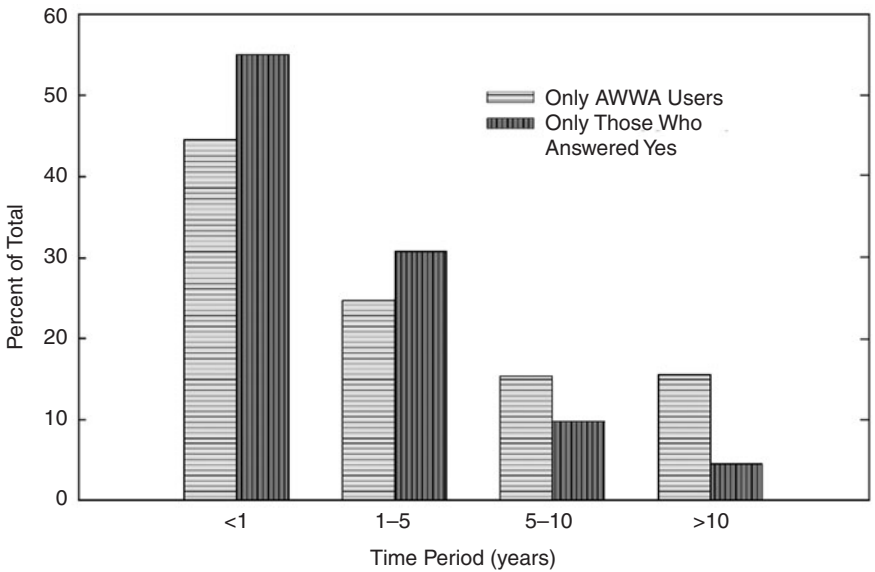
Figure 7.40 Comparison of when pipe problems occurred for AWWA C900/C905 PVC pipe users with those who reported problems with a particular manufacturer.
