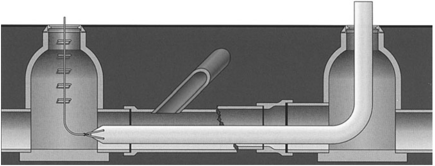
Figure 8.11 Diagram of liner pipe being pulled in a prepared host pipe. (Courtesy of Ultraliner.)
