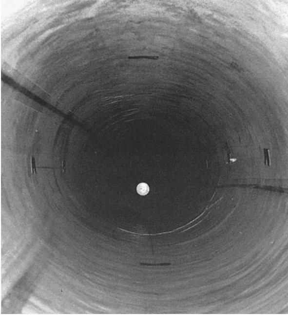
Figure 8.7 The inside of the broken rigid pipe test section after loading to a vertical soil pressure of 8700 lb/ft 2 .
