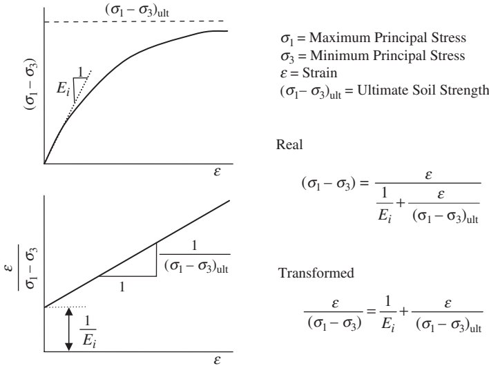
Figure 3.38 Hyperbolic presentation of a stress-strain curve. (After Duncan et al. 6 )
