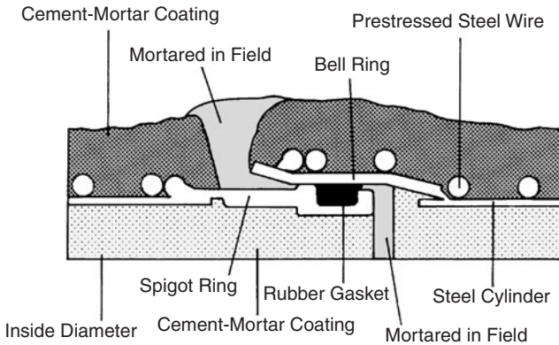
Figure 5.9 Wall cross section of pretensioned shot-cote concrete cylinder pipe. (Reprinted, by permission, from Bulletin No. 200, United Concrete Pipe Corporation. )
