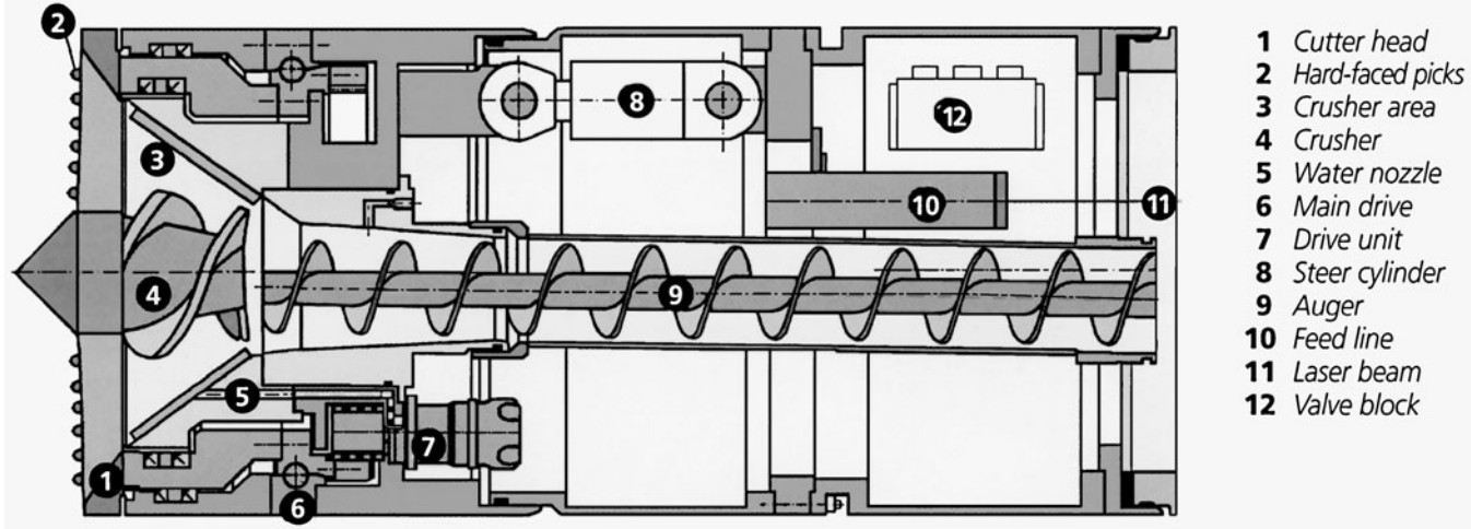
Figure 8.21 Microtunneling machine with auger material removal. (Courtesy of Herrenknecht GmbH, Germany.)
