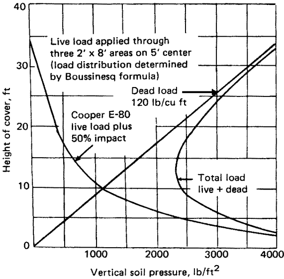
Figure 2.20 Cooper E-80 live loading. (Reprinted, by permission, from Handbook of Steel Drainage and Highway Construction Products , 2 American Iron and Steel Institute, Washington, D.C.)
