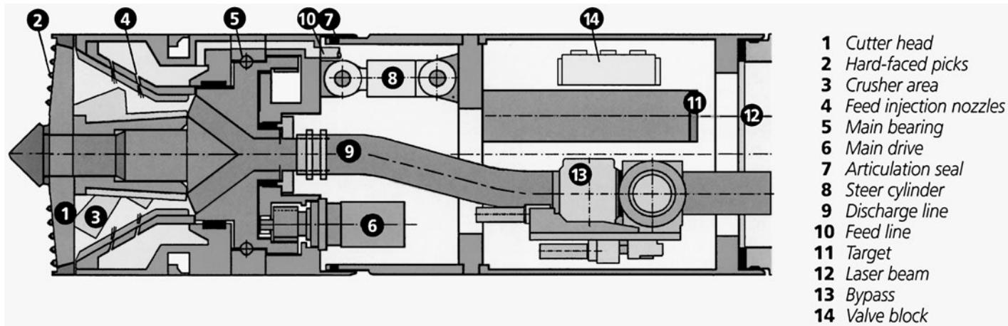
Figure 8.20 Microtunneling machine with slurry material removal. (Courtesy of Herrenknecht GmbH, Germany.)
