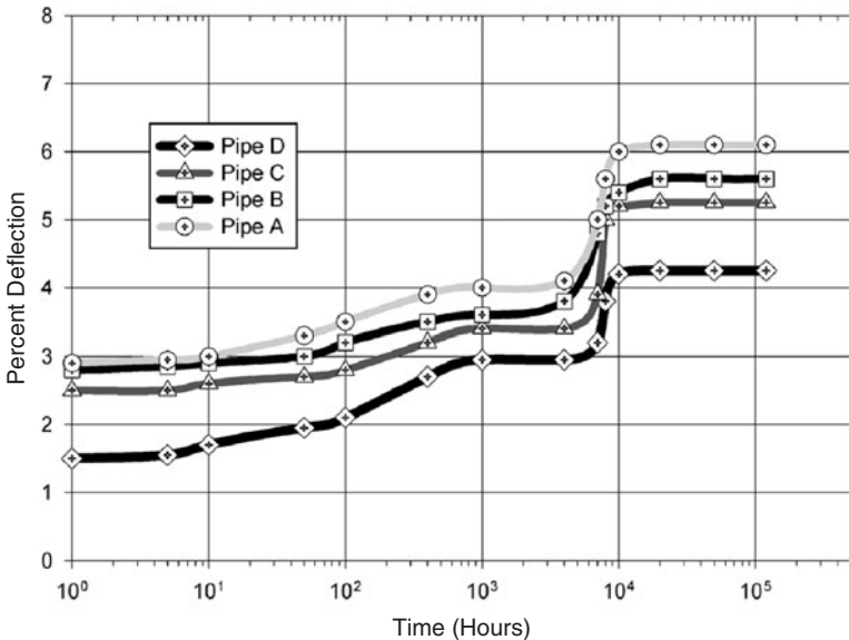
Figure 3.15 Deflection versus time for 10-in-diameter PVC sewer pipe (22-ft-deep embankment).
