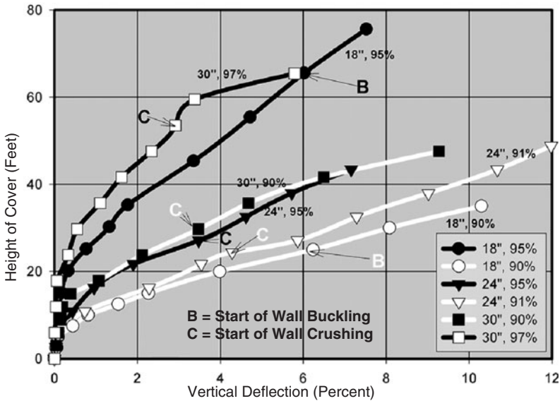
Figure 3.10 Vertical deflections for the six load-deflection tests on steel pipe. Note that the curves are concave downward and have knees corresponding to preconsolidation (compaction) of the soil.
