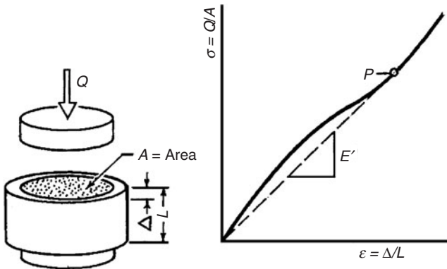
Figure 2.29 Confined compression soil test.
