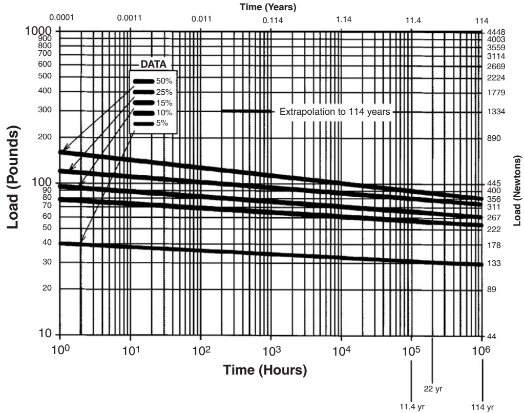
Figure 7.15 Relaxation curves for unfilled, notched PVC pipe rings at specified deflections and a temperature of 40°F.
