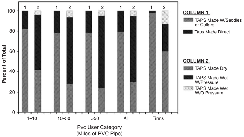
Figure 7.22 Average responses concerning taps made on AWWA C900/C905 PVC pipe for each PVC user group and engineering firms.
