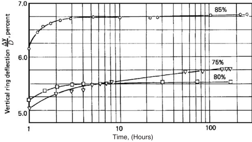
Figure 3.13 PVC pipe creep response.
