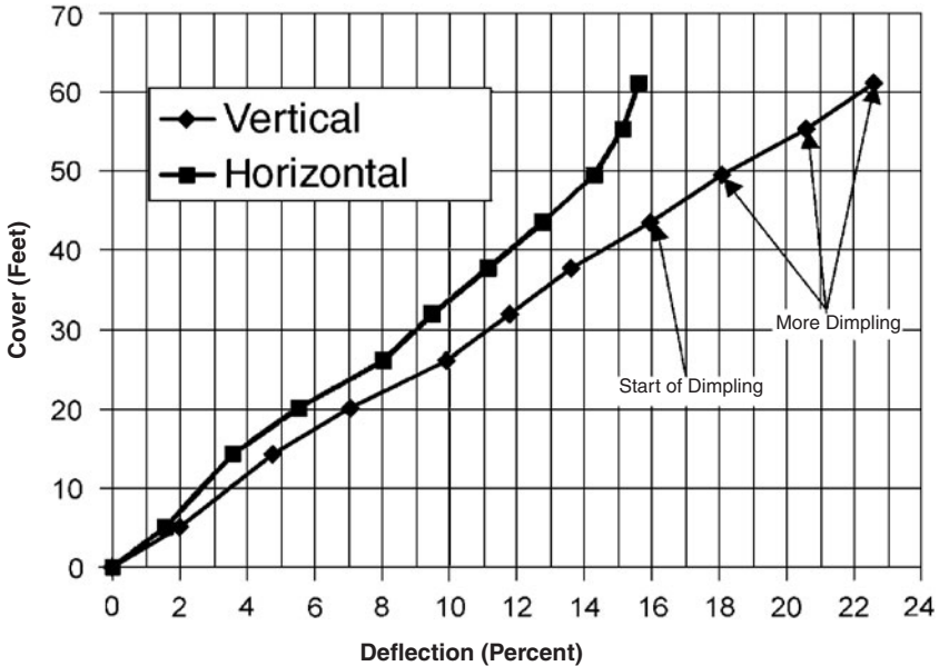
Figure 7.63 Load deflection curves for 60-in-diameter HDPE pipe. Soil is silty sand compacted to 75 percent of standard Proctor density. Measurements are made at center of pipe.
