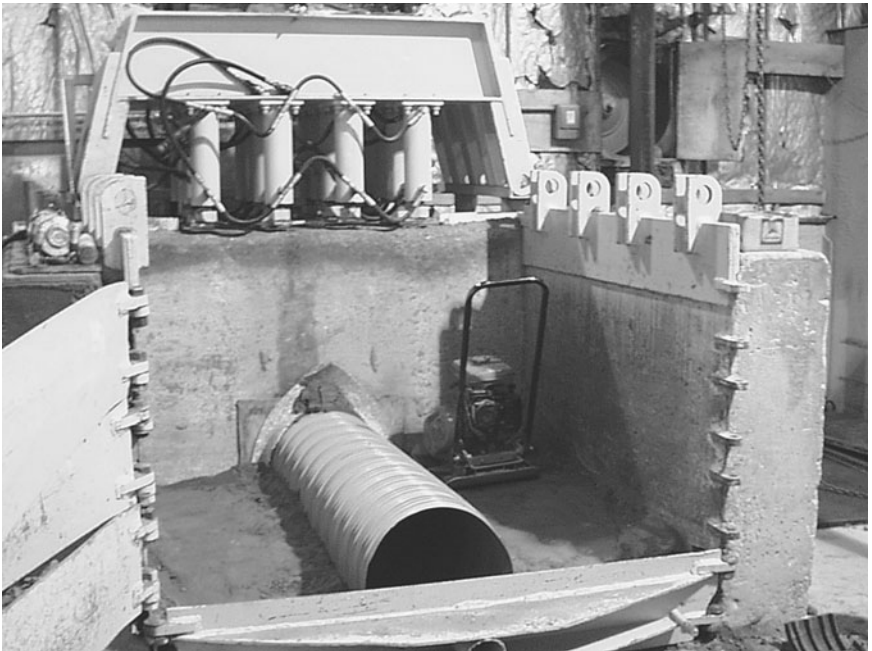
Figure 6.21 An 18-in ribbed pipe is being installed in small soil load cell at Utah State University.
