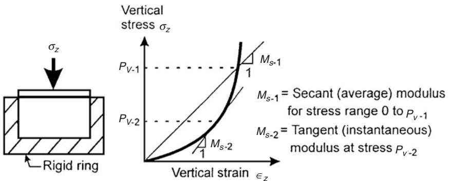
Figure 3.11 Constrained compression test schematic.
