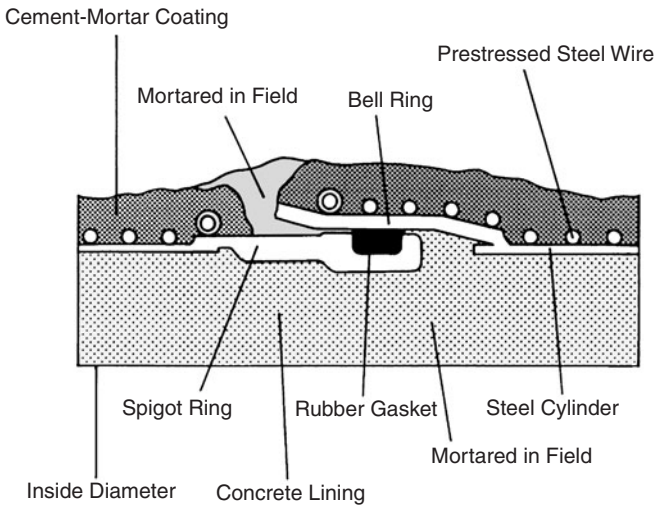
Figure 5.6 Wall cross section of lined cylinder pipe. (Reprinted, by permission, from Bulletin No. 200, United Concrete Pipe Corporation. )
