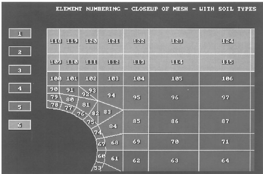
Figure 3.45 Printed output showing element numbering scheme of upper part of mesh in an FEA model.
