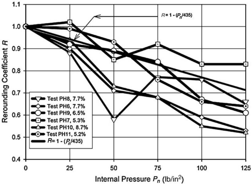
Figure 4.22 Rerounding coefficient from test data—poor haunch condition.
