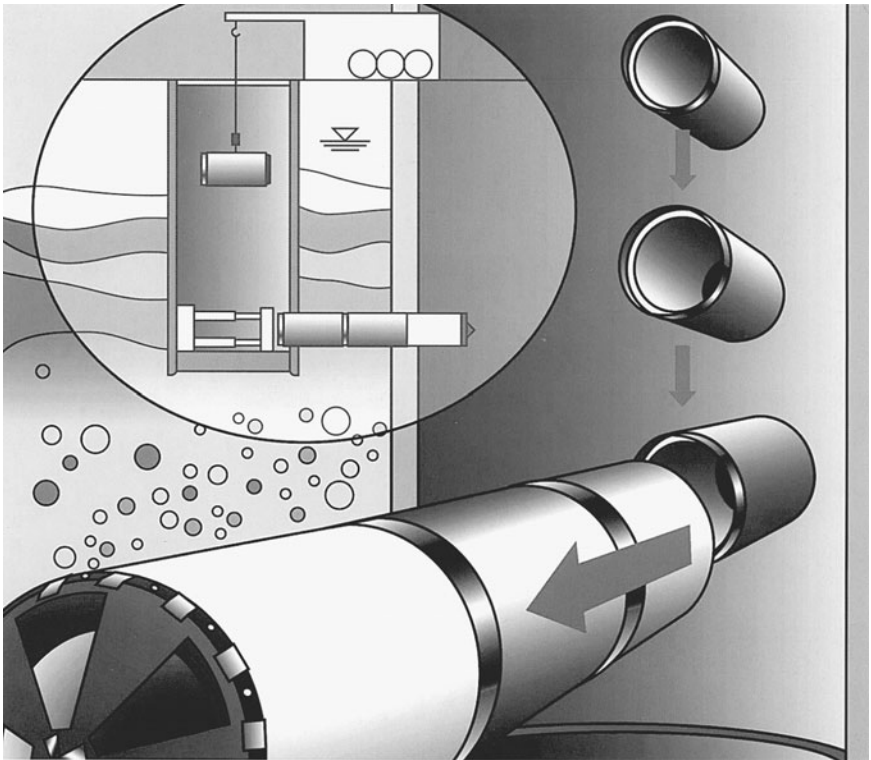
Figure 8.16 Diagram of how pipe is installed by jacking with a boring machine. (Courtesy of Meyer-Polycrete.)
