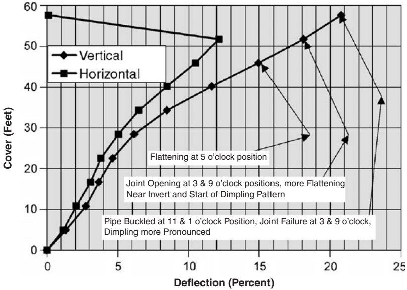
Figure 7.71 Load deflection curves for 48-in-diameter HDPE pipe. Soil is silty sand compacted to 77 percent of standard Proctor density. Measurements are made at center of pipe.
