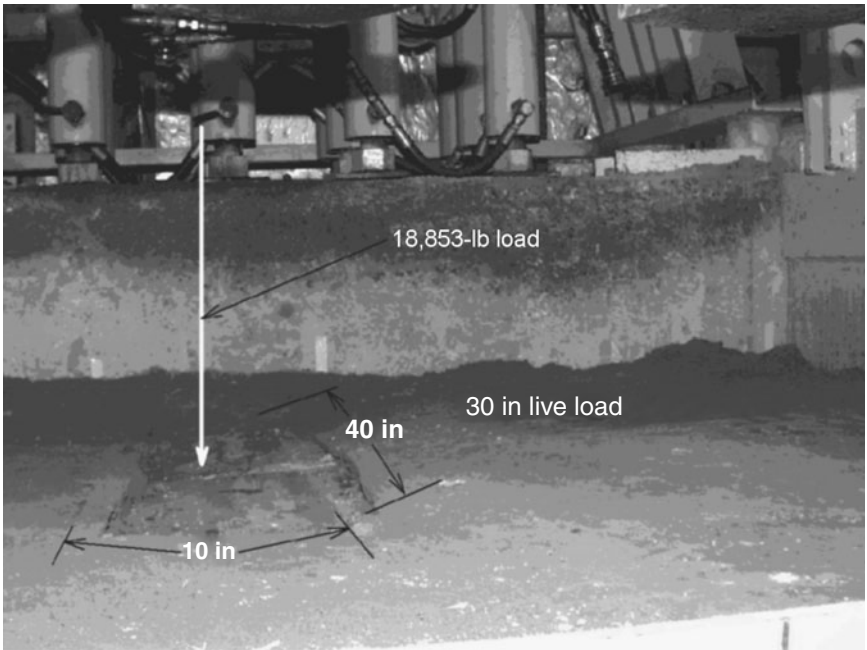
Figure 6.29 Application of an 18,853-lb load.
