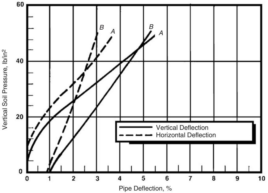
Figure 3.52 Vertical soil pressure versus pipe deflection. (A) Soil box data 90 percent relative compaction, silty sand; (B) FEA with compaction simulation.
