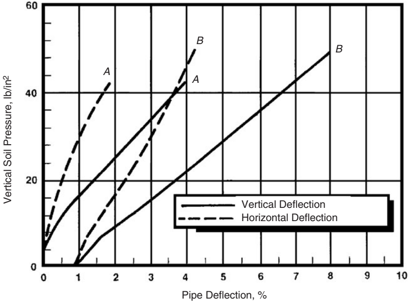
Figure 3.56 Vertical soil pressure versus pipe deflection. (A) Soil box data, 90 percent relative compaction, silty sand, and poor haunch support; (B) FEA with compaction simulation and poor haunch support.
