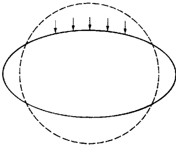
Figure 3.24 Ring deflection in a flexible pipe.
