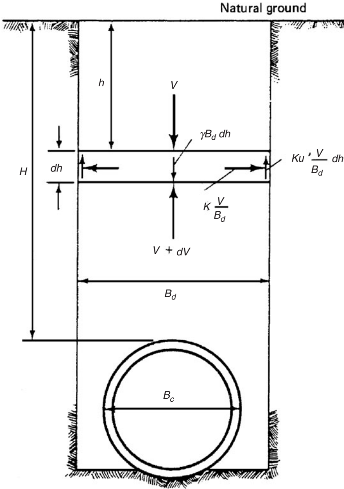
Figure 2.1 Basis for Marston's theory of loads on buried pipe. W_d = load on conduit per unit length along conduit in pounds per linear foot; e = base of natural logarithms; \gamma = unit weight of backfill, i.e., pounds per cubic foot; V = vertical pressure on any horizontal plane in backfill, in pounds per unit length of ditch; B_c = horizontal breadth (outside) of conduit, in feet; B_d = horizontal width of ditch at top of conduit, in feet; H = height of fill above top of conduit, in feet; h = distance from ground surface down to any horizontal plane in backfill, in feet; C_d = load coefficient for ditch conduits; \mu = \tan \phi = coefficient of internal friction of backfill; \mu' = \tan \phi' = coefficient of friction between backfill and sides of ditch; K = ratio of active lateral unit pressure to vertical unit pressure. (Reprinted, by permission, from Spangler and Handy, Soil Engineering , 4th ed., Harper & Row, 1982.)
