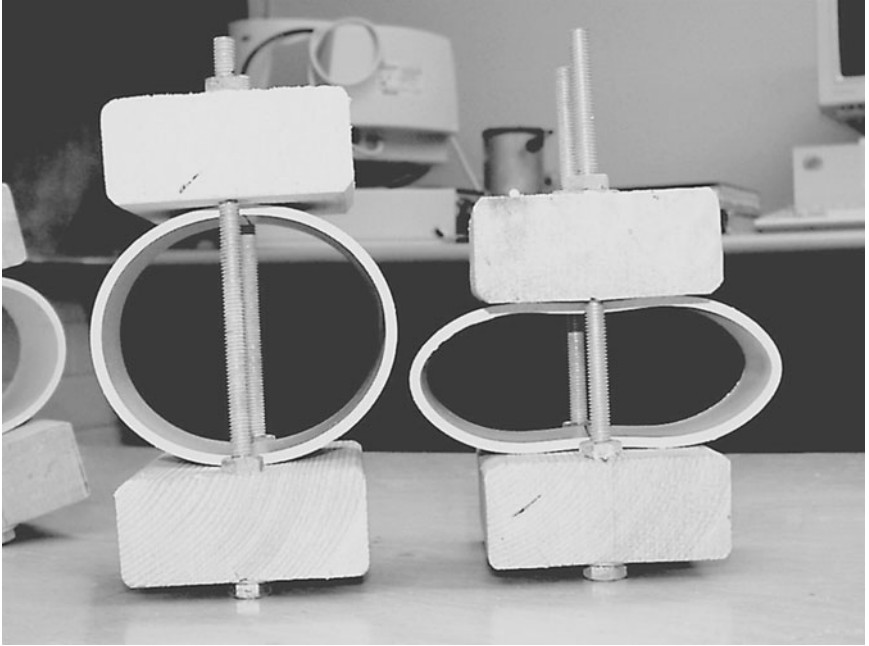
Figure 7.7 Pipe ring specimens held in constant deformation.
