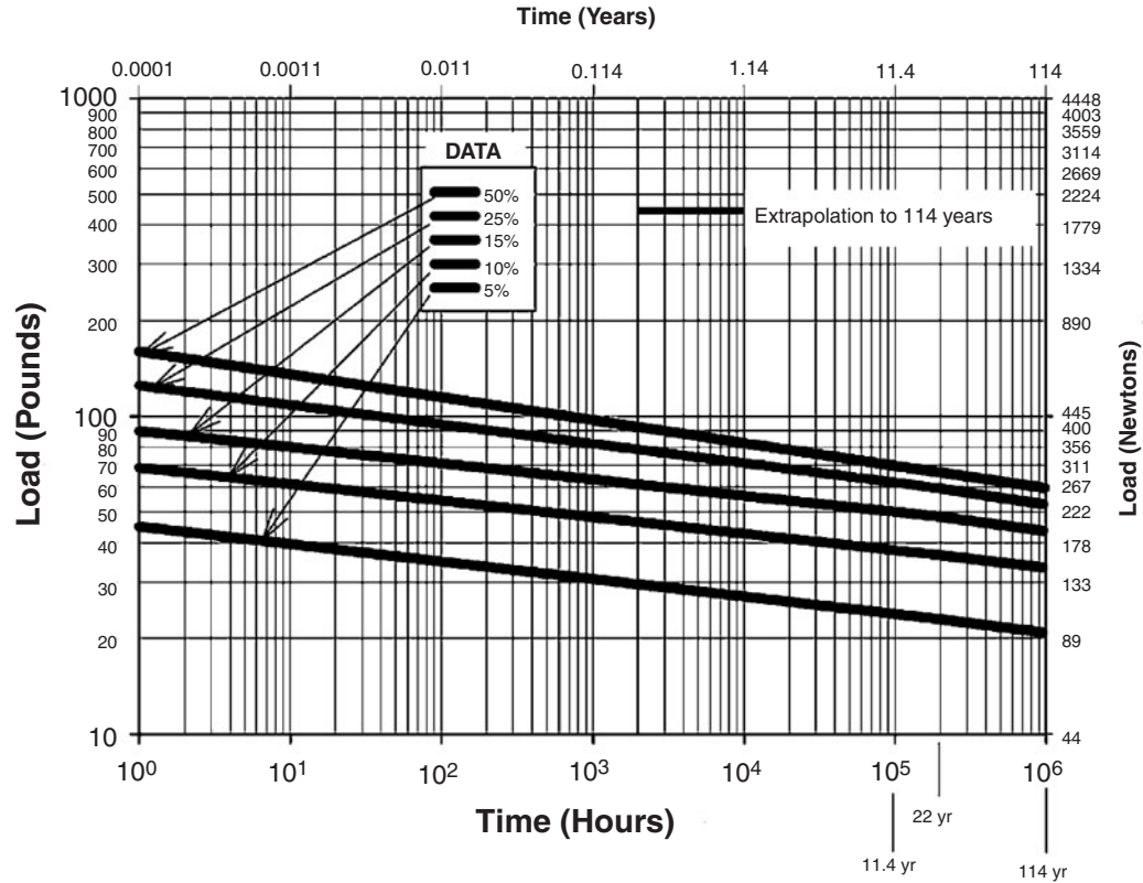
Figure 7.16 Relaxation curves for unfilled, unnotched PVC pipe rings at specified deflections and a temperature of 70°F.
