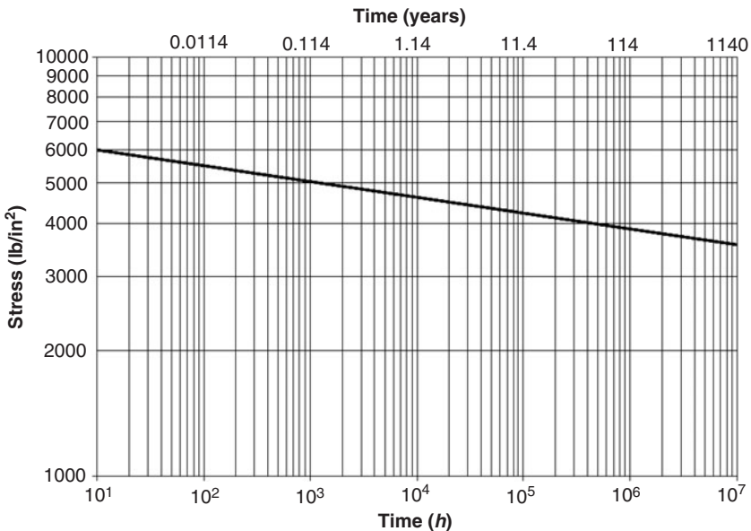
Figure 4.6 Stress regression line for PVC pressure pipe.
