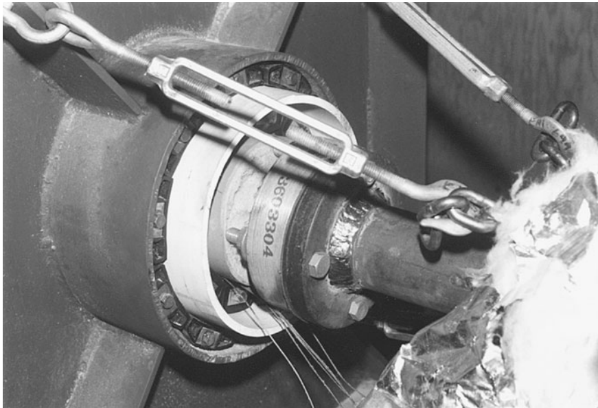
Figure 6.65 External connection and thrust restraint.
