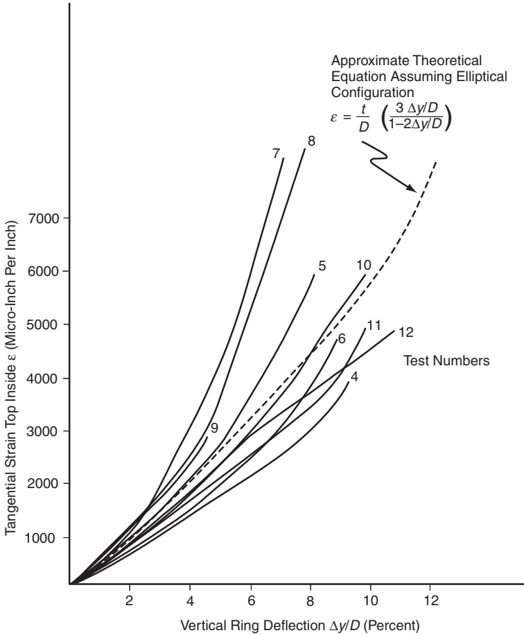
Figure 6.48 Strain in pipe wall as a function of percent of vertical deflection.
