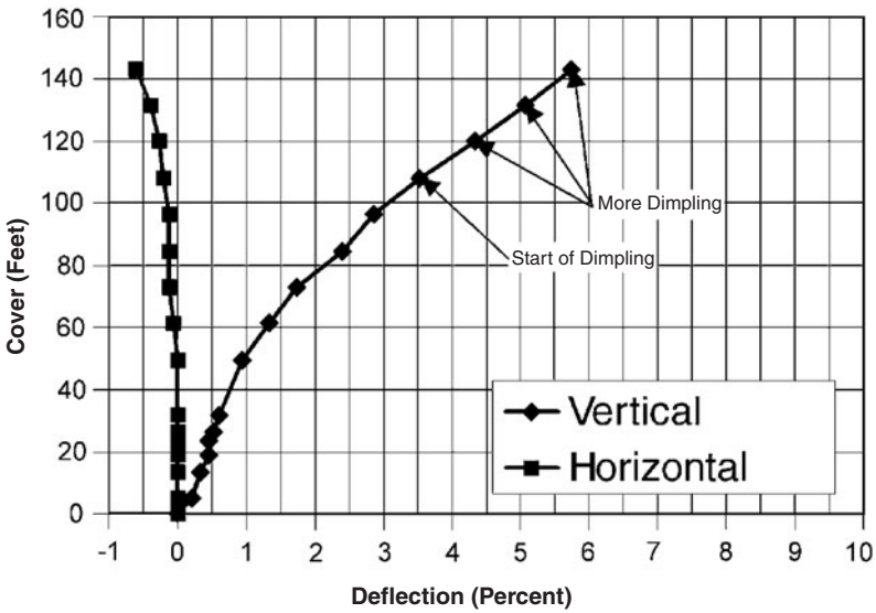
Figure 7.62 Load-deflection curves for 60-in-diameter HDPE pipe. Soil is silty sand compacted to 95 percent of standard Proctor density. Measurements are made at center of pipe.
