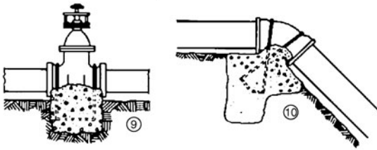
Figure 4.29 Types of thrust blocking. (Reprinted, by permission, from Handbook of PVC Pipe, 21 Uni-Bell PVC Pipe Association.)
