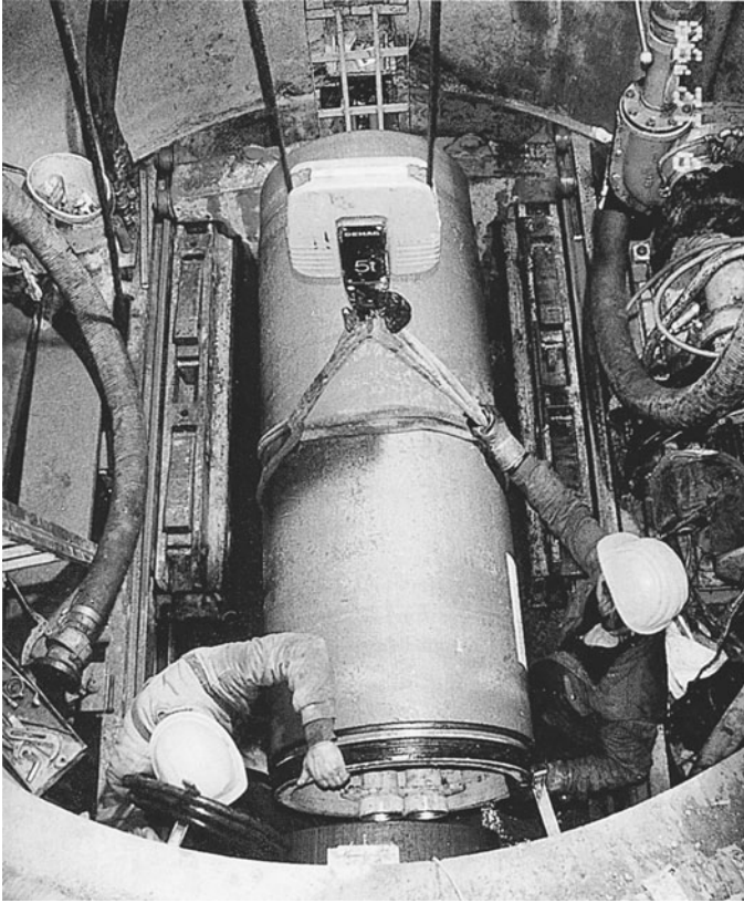
Figure 8.18 Polycrystalline pipe in jacking pit. (Courtesy of Meyer-Polycrystalline.)
