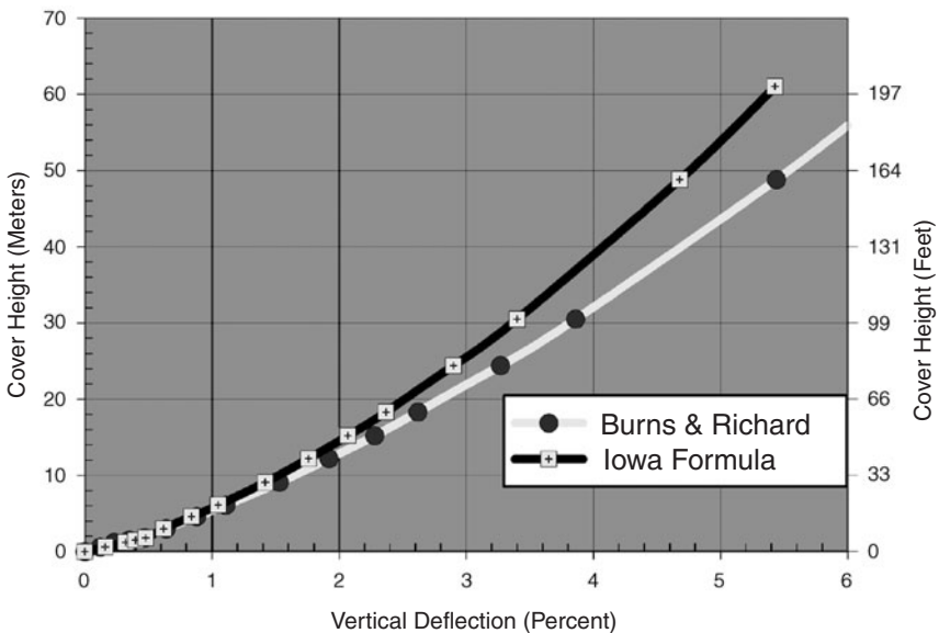
Figure 3.34 Comparison of the Burns and Richard solution with the Iowa formula for the case when the same overburden-dependent soil modulus is used in both solutions. Initial E' is 11.02 \text{ MPa} or 1600 \text{ lb/in}^2 .
