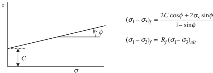
Figure 3.39 Variation of strength with confining pressure. (After Duncan et al. 6 )
