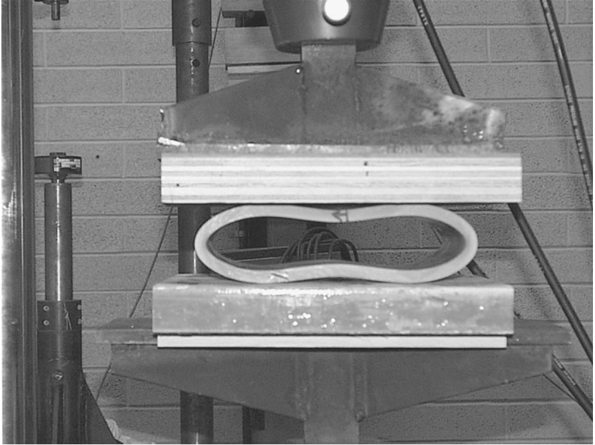
Figure 4.13 Prequalification flattening test (after flattening).
