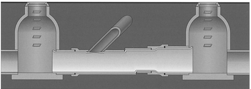
Figure 8.13 Diagram of liner pipe after expansion. The liner forms a permanent, tight-fitting new pipe. (Courtesy of Ultraliner.)
