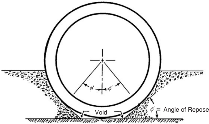
Figure 2.26 Rigid pipe cross section showing how voids are left if soil is not deliberately placed under the haunches.
