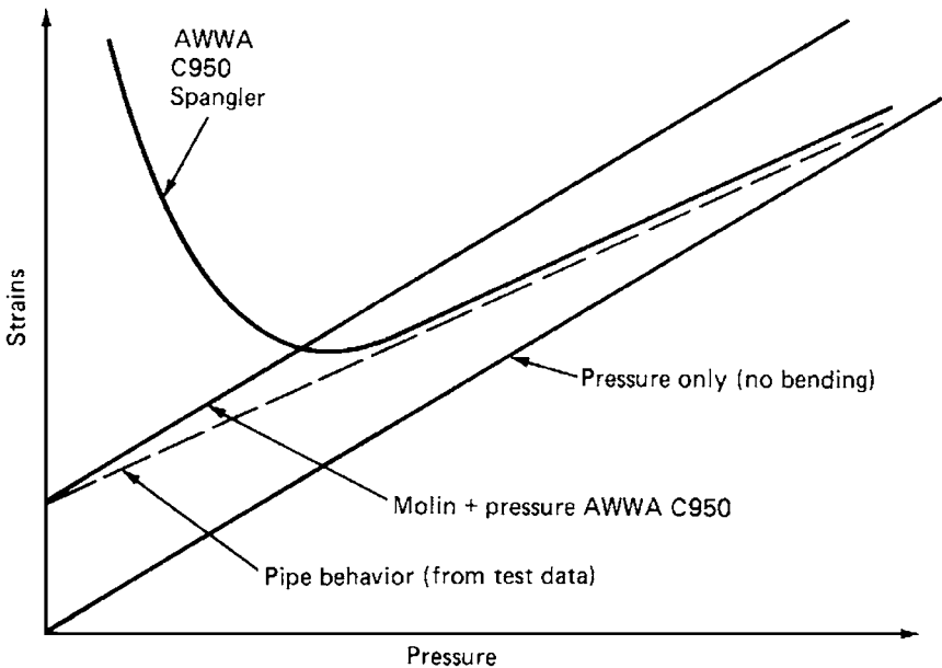
Figure 4.26 Typical plot for combined strains.
