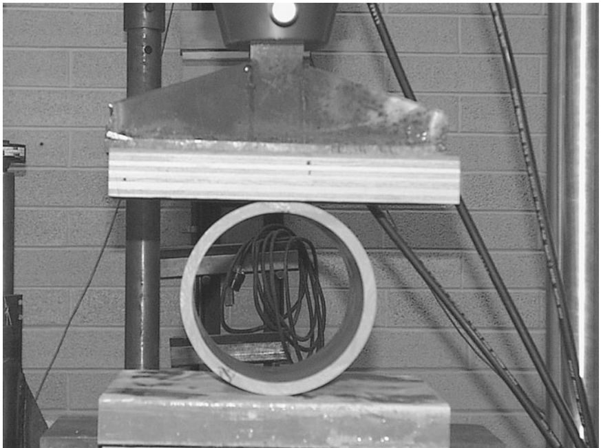
Figure 4.12 Prequalification flattening test (before flattening).
