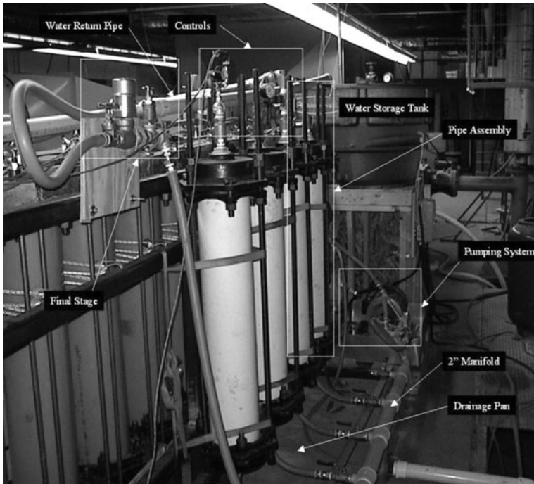
Figure 4.11 Pressure cycling test setup.
