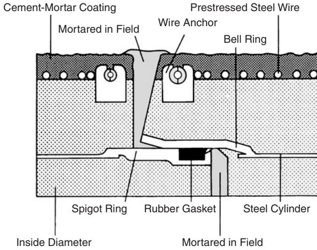
Figure 5.5 Wall cross section of embedded cylinder pipe. (Reprinted, by permission, from Bulletin No. 200, United Concrete Pipe Corporation. )
