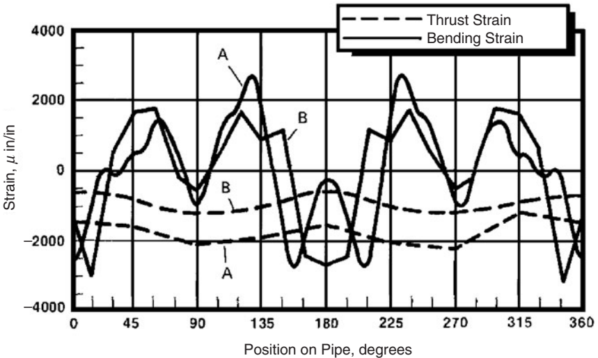
Figure 3.51 Pipe strain as function of circumferential position, conditions as in Fig. 3.50.
