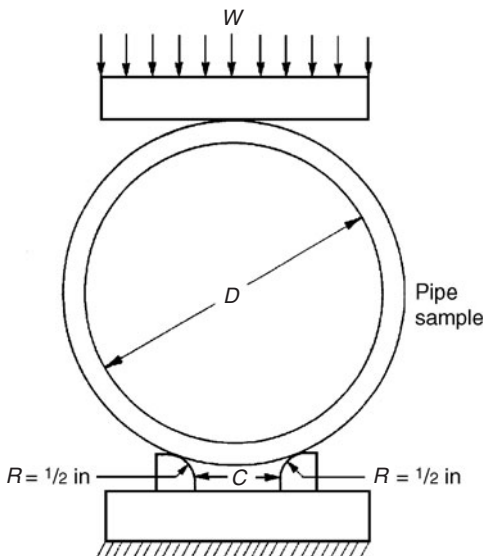
Figure 3.4 Three-edge bearing (wood block) schematic.
