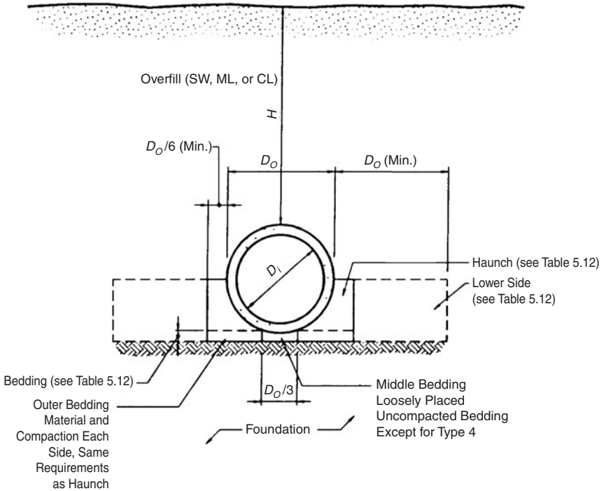
Figure 5.10 Standard embankment installations.
