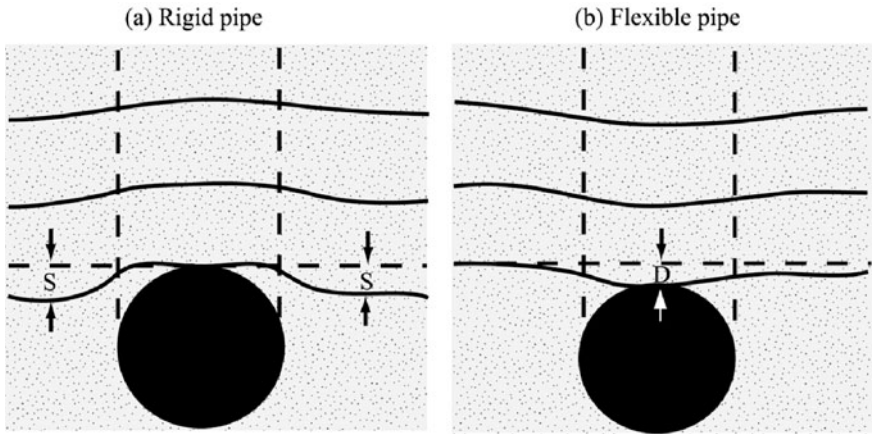
Figure 1.1 The effect of soil settlement on (a) rigid and (b) flexible pipes. S represents settlement of backfill for a rigid pipe. D represents vertical deflection of a flexible pipe as it deflects under earth pressure. (Reprinted, by permission, from AWWA Manual M-11, Steel Pipe Design and Installation , American Water Works Association, 1964.)
