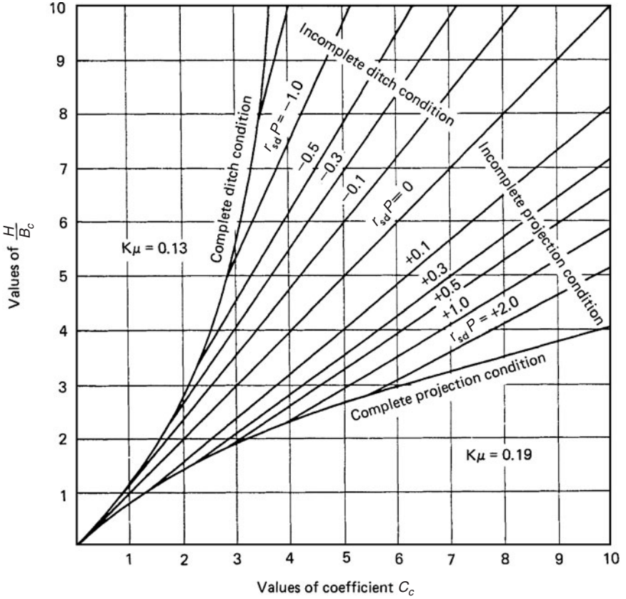
Figure 2.5 Diagram for coefficient C_c for positive projecting conduits. (Reprinted by permission, from Spangler and Handy, Soil Engineering , 4th ed., Harper & Row, 1982.)
