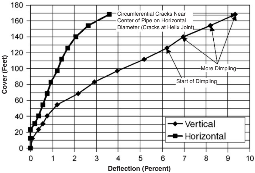
Figure 7.66 Load deflection curves for 42-in-diameter HDPE pipe. Soil is silty sand compacted to 95 percent of standard Proctor density. Measurements are made at center of pipe.
