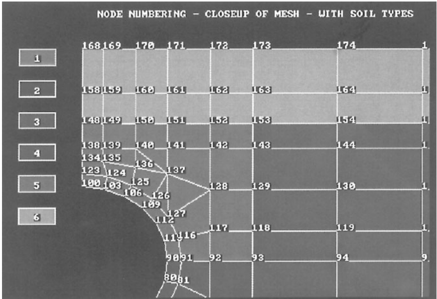
Figure 3.46 Printed output showing node numbering scheme of upper part of mesh in an FEA model.
