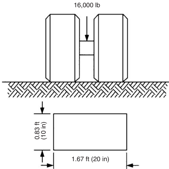
Figure 6.22 H-20 live load schematic.
