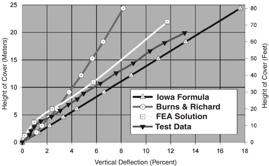
Figure 3.33 Comparison of test results with various analytical methods for a 48-in-diameter HDPE pipe buried in silty-sand soil compacted to 85 percent standard Proctor density.
