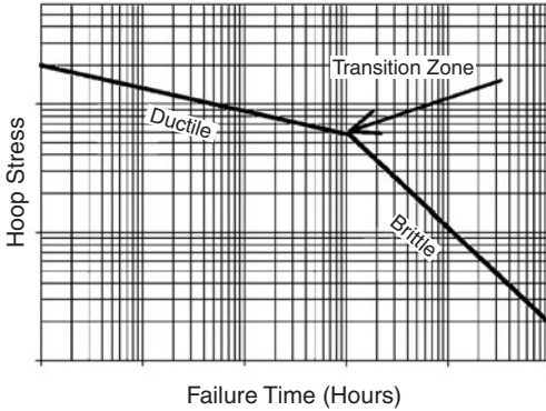
Figure 7.42 Schematic of stress regression for PE pipe.
