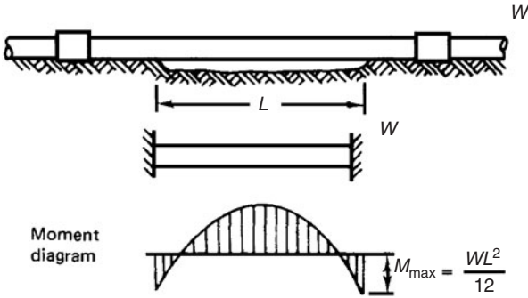
Figure 2.14 Longitudinal bending of conduits.
