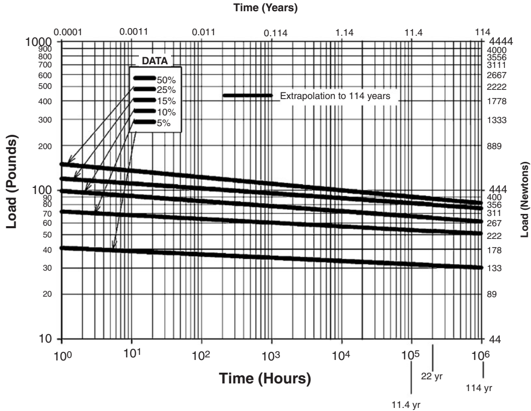
Figure 7.14 Relaxation curves for unfilled, unnotched PVC pipe rings at specified deflections and a temperature of 40°F.
