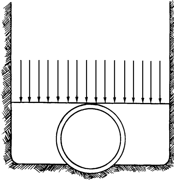
Figure 2.7 Load proportioning according to Marston's theory for a flexible pipe.
