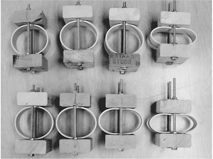
Figure 7.9 Pipe rings at various constant deflections.
