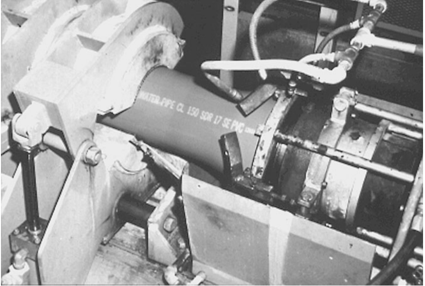
Figure 7.3 PVC pipe belling operation. (Reprinted by courtesy of Uni-Bell PVC Pipe Association.)
