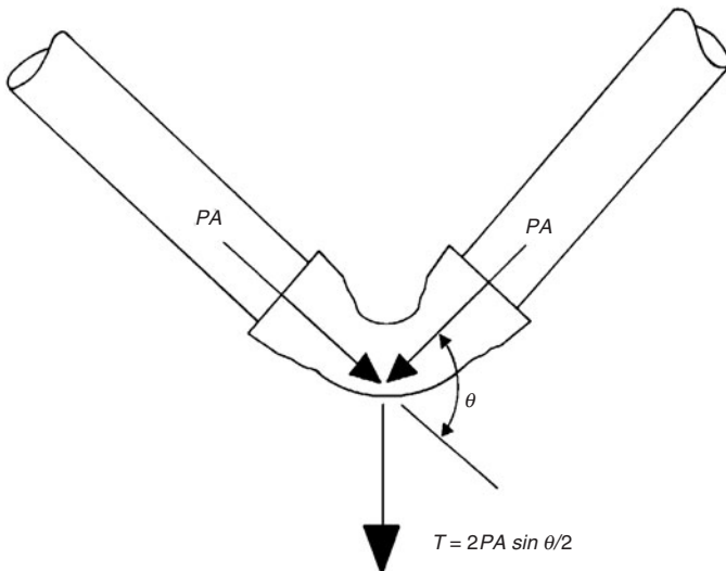
Figure 4.27 Thrust force. (Reprinted, by permission, from Thrust Restraint Design for Ductile Iron Pipe , Ductile Iron Pipe Research Association.)
