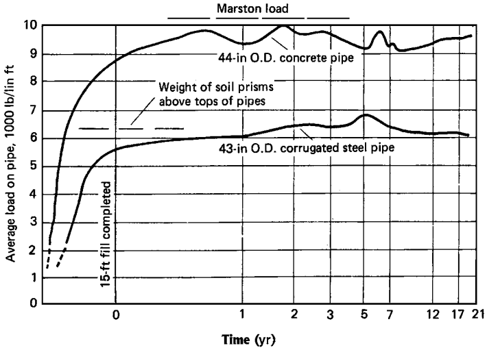
Figure 2.3 Measured loads on rigid and flexible pipe over a period of 21 years. (Reprinted, by permission, from Spangler and Handy, Soil Engineering , 4th ed., Harper & Row, 1982.)
