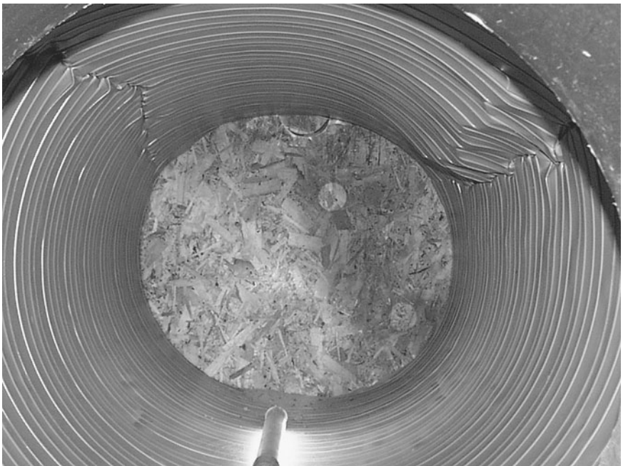
Figure 6.43 Steel-ribbed pipe (30-in diameter) at 42 ft of cover in silty-sand soil at 90 percent density.
