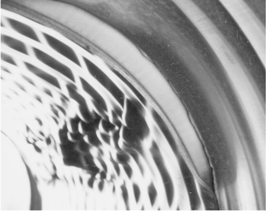
Figure 7.49 Test X-5, waffling pattern and local buckling (25 m of cover).
