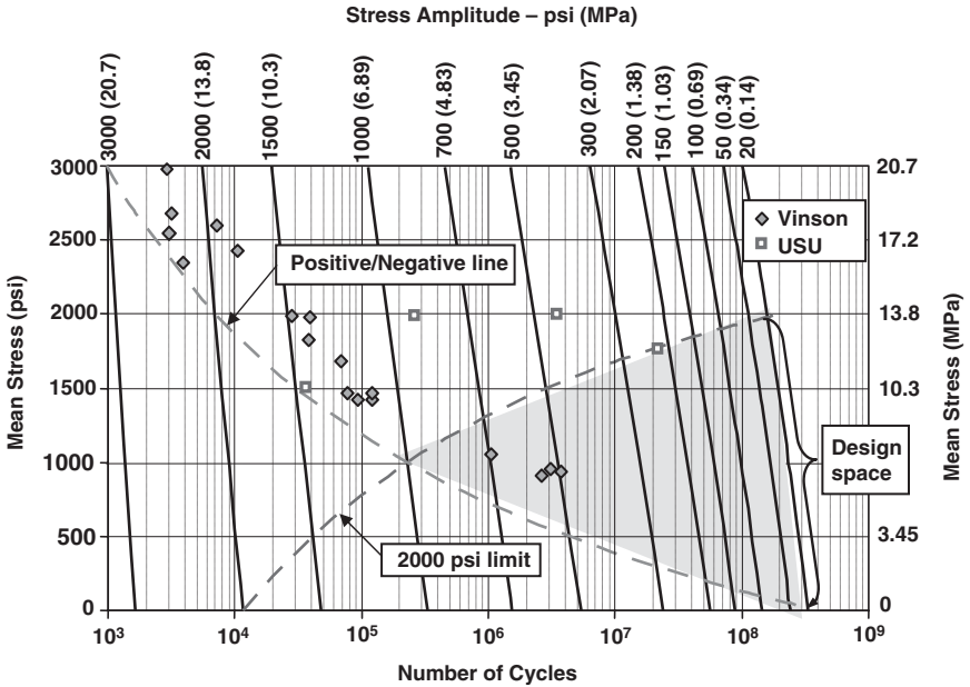
Figure 4.17 Plot of the number of cycles to failure vs. mean stress with design space shown shaded.
