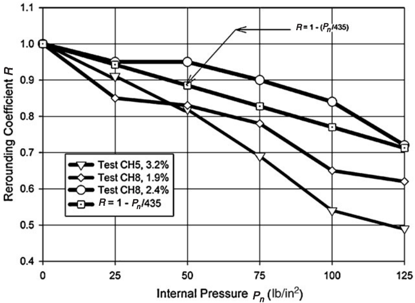
Figure 4.24 Rerounding coefficient from test data—complete haunch condition.
