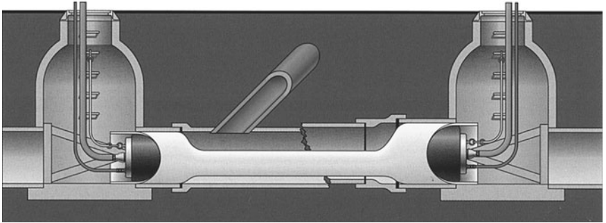
Figure 8.12 Diagram of plugged liner pipe to be expanded with steam pressure. (Courtesy of Ultraliner.)
