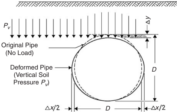
Figure 6.1 Ring deflection of buried flexible pipe.
