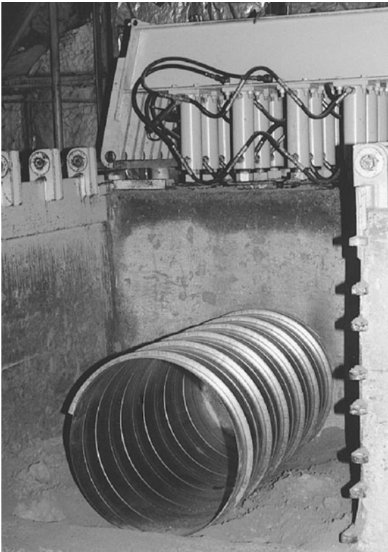
Figure 6.9 Placement of ribbed steel pipe in test cell.
