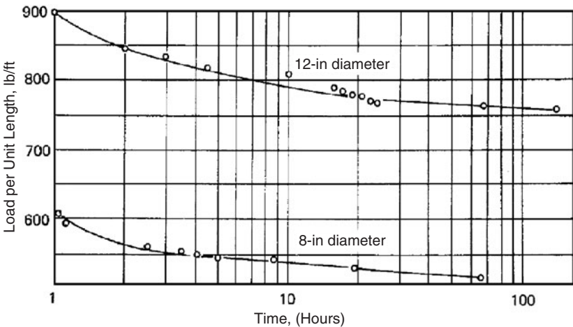
Figure 3.12 Stress relaxation curves.
