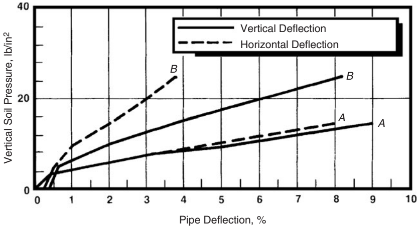
Figure 3.58 Vertical soil pressure versus pipe deflection. (A) Soil box data, 80 percent relative compaction; (B) FEA, no compaction simulation.
