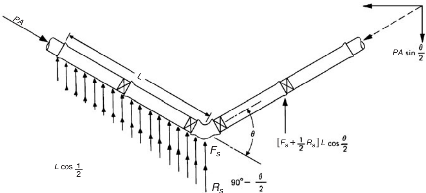
Figure 4.30 Free-body diagram for pipe with restrained joints. (Reprinted, by permission, from Thrust Restraint Design for Ductile Iron Pipe , Ductile Iron Pipe Research Association.)
