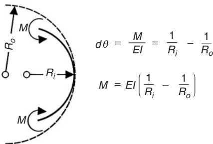
Figure 6.3 Relationship of moment to change in radius of curvature of pipe ring.
