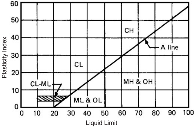
Figure 3.2 Plasticity chart. (Reprinted, by permission, from Asphalt Institute Soils Manual . 1 )
