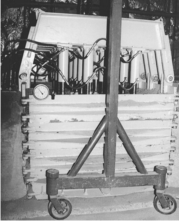
Figure 6.10 Test cell in operation—pistons of cylinders extended.
