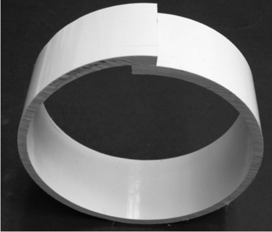
Figure 7.18 Angular closing due to frozen-in stresses.
