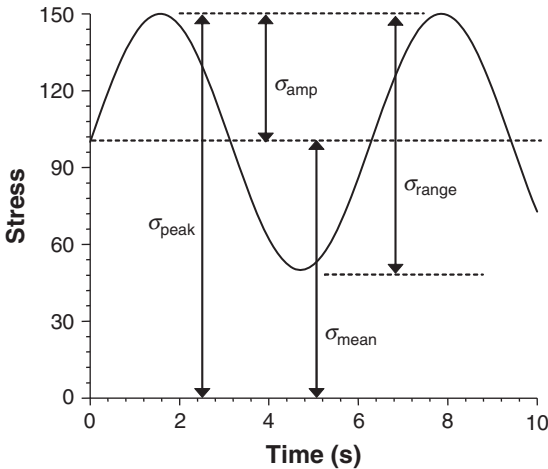
Figure 4.8 Illustration of stress terms.
