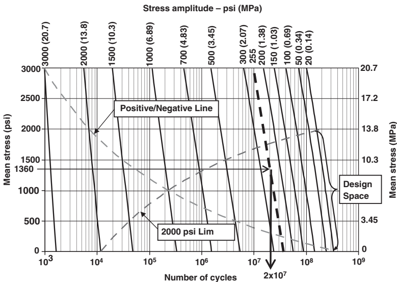
Figure 4.18 Number of cycles to failure for Example 4.2.
