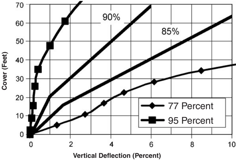
Figure 7.73 Vertical deflection curves for 48-in HDPE pipe at various soil densities. The solid lines are approximated curves for intermediate densities.
