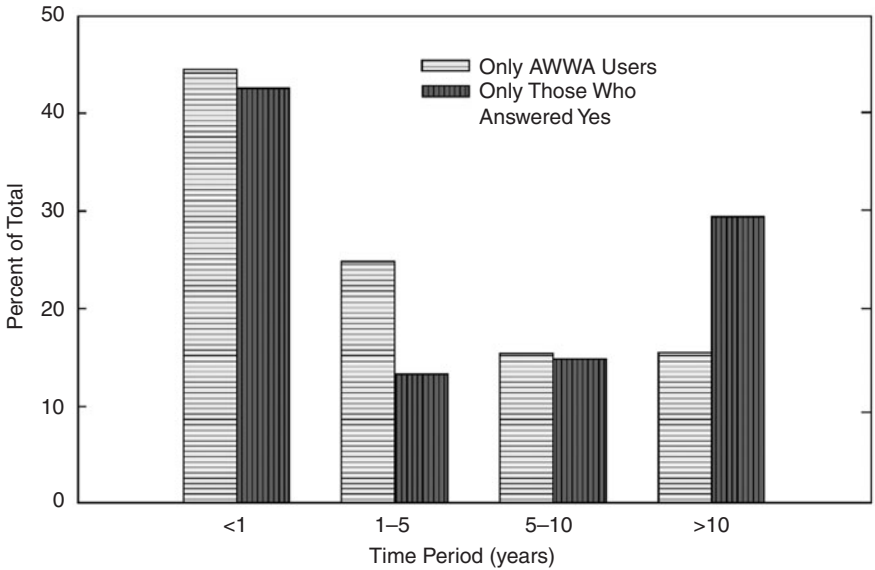
Figure 7.38 When PVC problems occurred—a comparison of those who reported using sunburned pipe with AWWA C900/C905 PVC pipe users.
