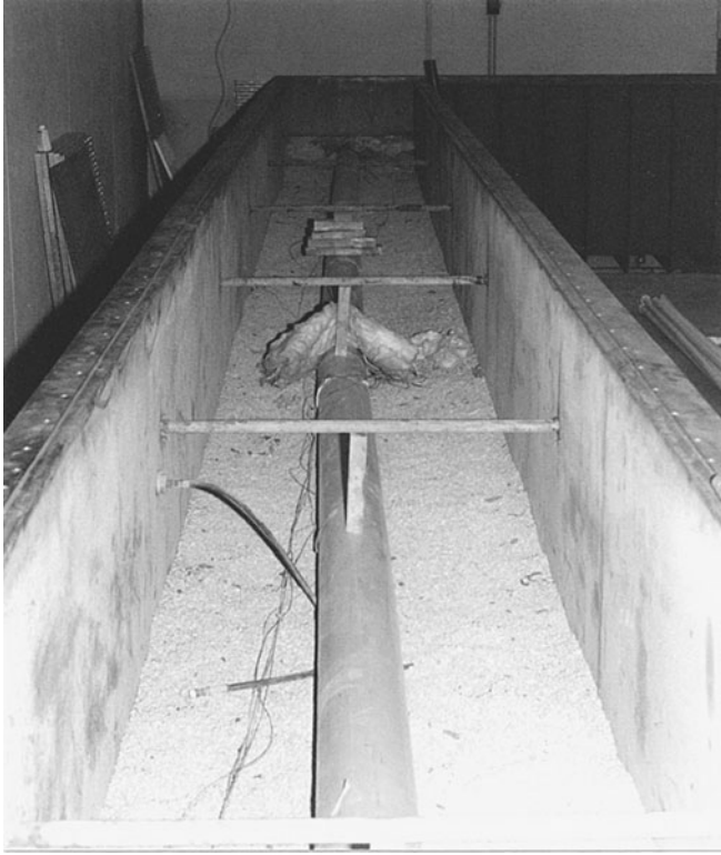
Figure 6.66 Condensate pipe in test cell.
