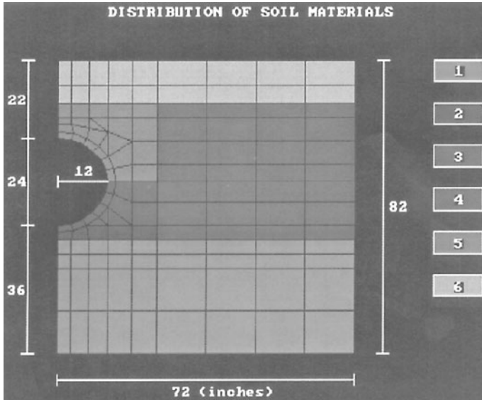
Figure 3.44 Photograph of a PC monitor display showing various soil types and/or compactions used in an FEA model.
