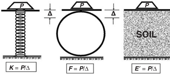
Figure 2.9 Graphic of spring, pipe, and soil.
