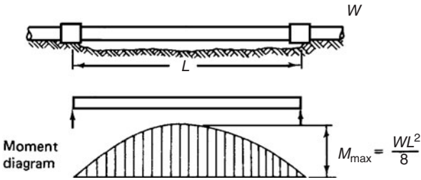
Figure 2.15 Longitudinal bending of conduits.
