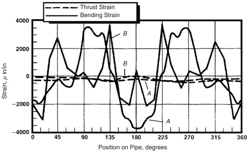
Figure 3.59 Pipe strain as function of circumferential position, conditions as in Fig. 3.58.
