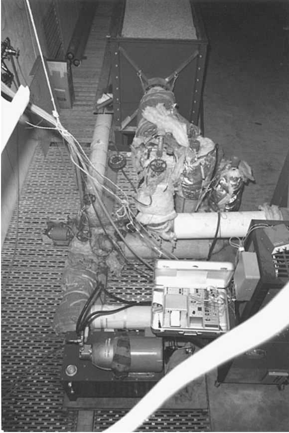
Figure 6.59 Looking down on the heating section located between the two test cells. Note the following: (1) Tops of two 5000-W immersion-type heaters (center right of photo). A third heater is concealed from view. (2) Motor that runs the circulation pump (center left of photo). (3) Insulation applied to external piping to conserve energy.
