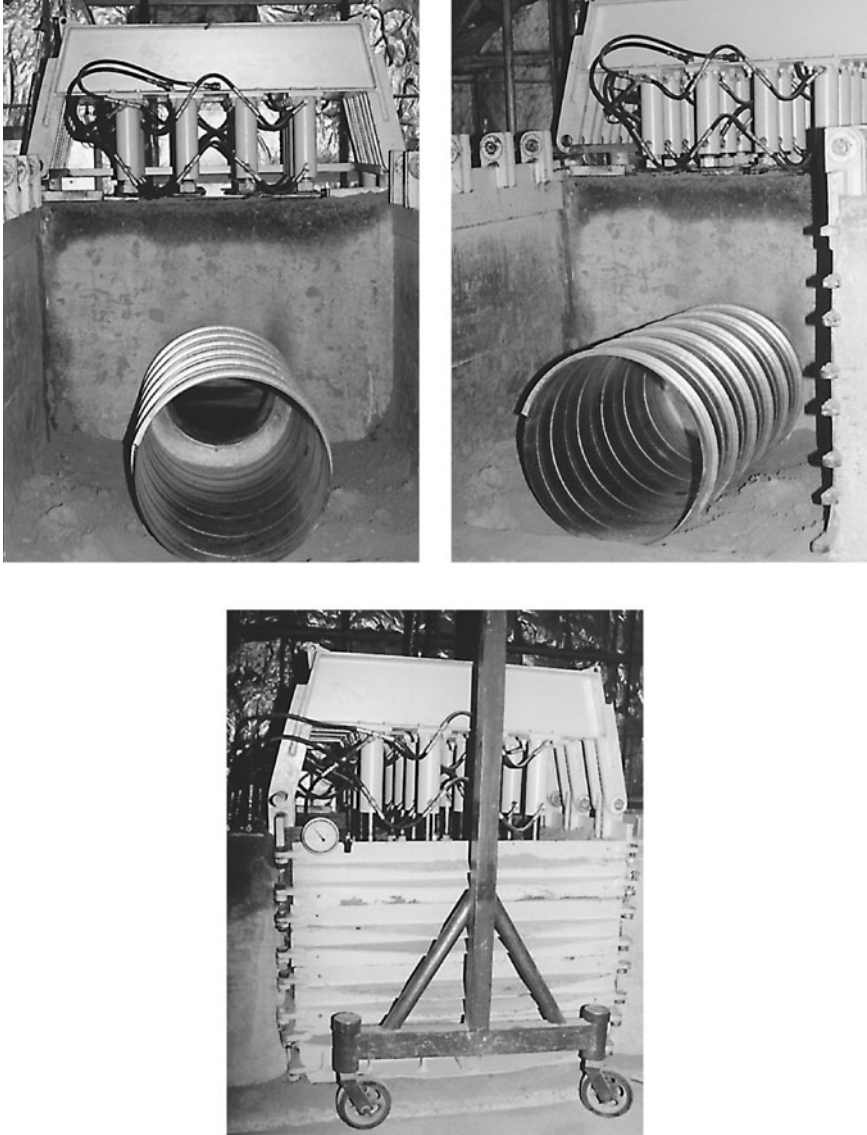
Figure 3.48 Small test cell at Utah State University.
