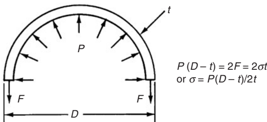
Figure 4.7 Stress due to internal pressure.
