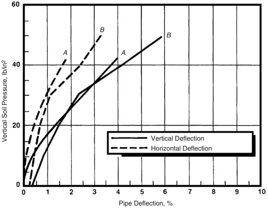
Figure 3.54 Vertical soil pressure versus pipe deflection. (A) Soil box data, 90 percent relative compaction, silty sand, and poor haunch support; (B) FEA, no compaction simulation, and poor haunch support.
