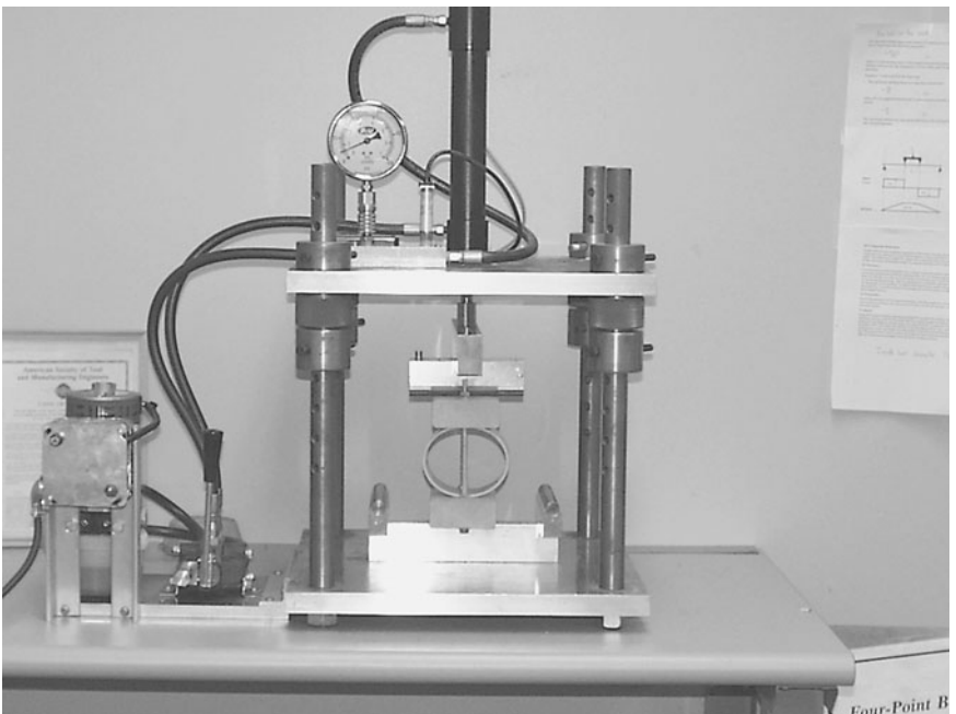
Figure 7.8 Pipe ring undergoing stress relaxation testing.
