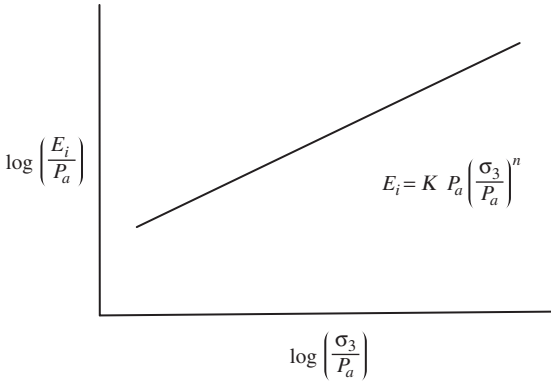
Figure 3.40 Variation of initial tangent modulus with confining pressure. (After Duncan et al. 6 )
