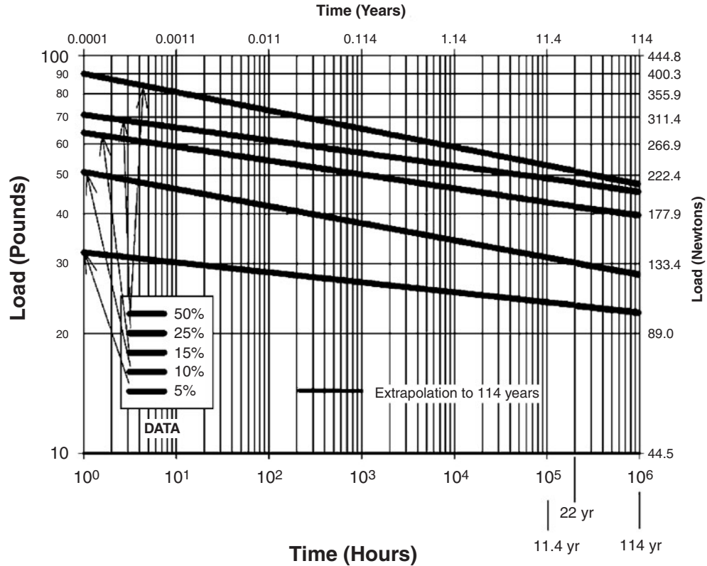
Figure 7.12 Relaxation curves for filled, unnotched PVC pipe rings at specified deflections and a temperature of 40°F.
