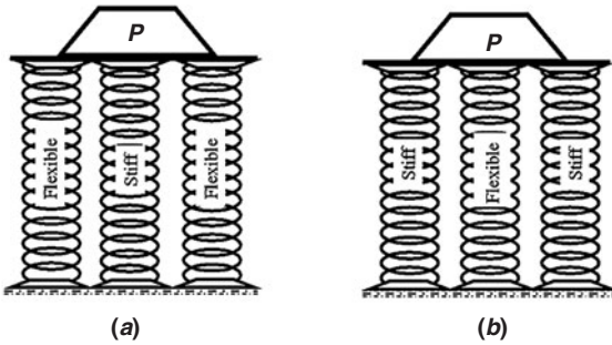
Figure 2.10 Flexible and stiff springs working together.
