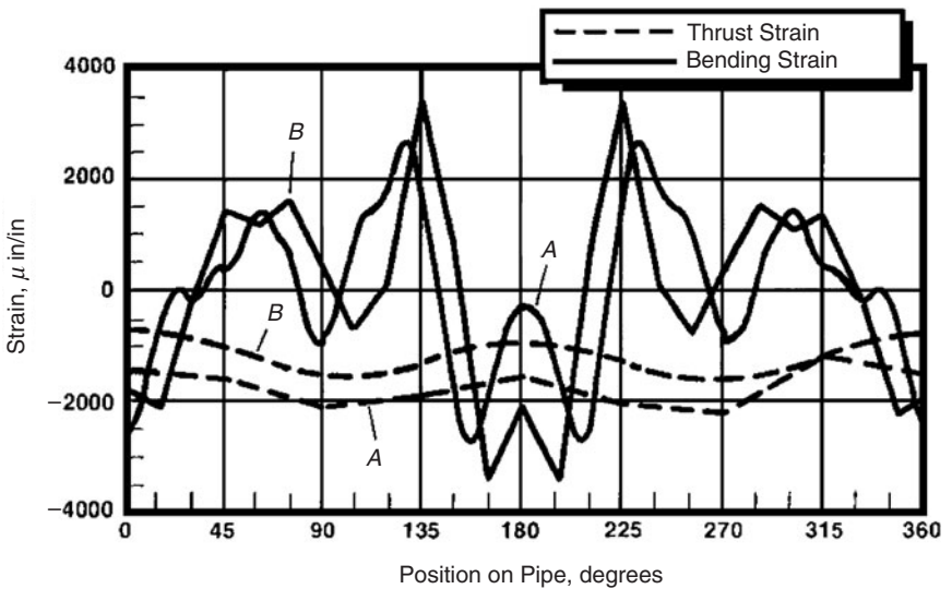
Figure 3.53 Pipe strain as function of circumferential position, conditions as in Fig. 3.52.
