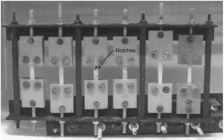
Figure 7.10 Uniaxial tensile stress relaxation specimens.
