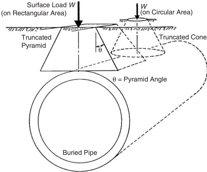
Figure 2.22 Soil stress models for minimum cover are free-body diagrams of truncated pyramid and cone showing shear planes on slope \theta at “punch-through.”
