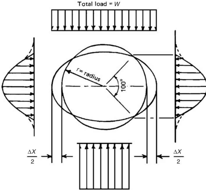
Figure 3.6 Basis of Spangler's derivation of the Iowa formula for deflection of buried pipes. \Delta X = D_L K W_c r^3 / (EI + 0.061er^4) (the Iowa formula), where e = 2h/\Delta X , 2r = D = pipe diameter, K = bedding constant, D_L = deflection lag factor, and EI = stiffness factor (related to pipe stiffness). (Reprinted, by permission, of Utah State University.)
