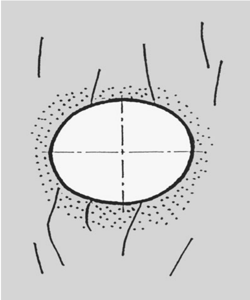
Figure 3.8 Soil slip planes in an embankment of sand compacted to 85 percent standard Proctor density.
