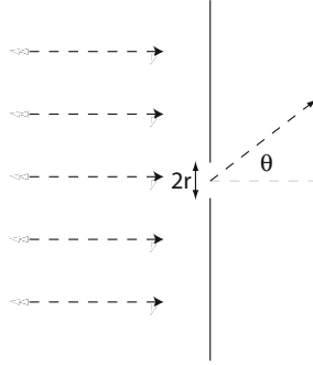
Figure 8.1. Transmission of light through a circular aperture or radius r in an infinitely thin opaque screen.
