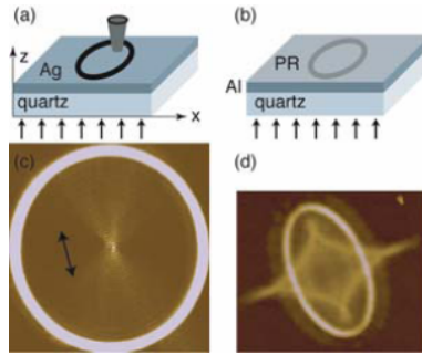
Figure 7.6. Generation and focusing of SPPs via illumination of circular or elliptic slits milled into a metallic film. The SPP intensity is monitored via near-field microscopy (a, c) or the exposure of a photoresist superstrate (b, d). Reprinted with permission from [Liu et al., 2005] Copyright 2005, American Chemical Society.
