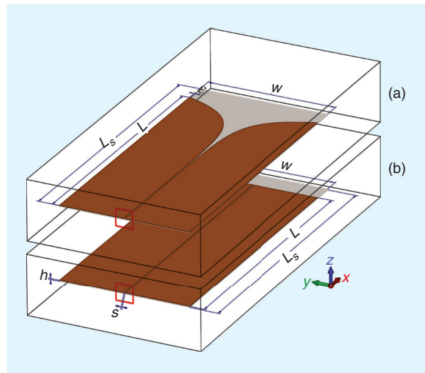
FIGURE 8. The structural models of (a) a Vivaldi antenna and (b) a slot line with excitation ports.
