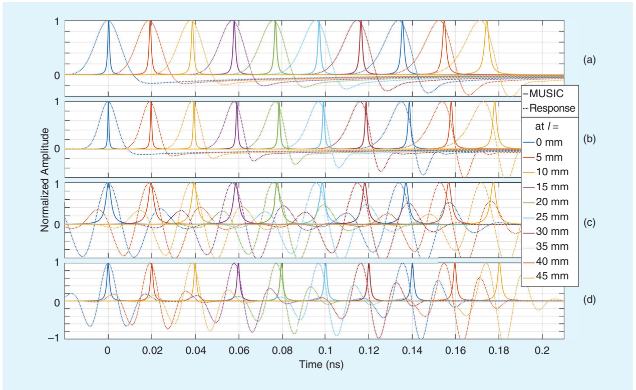
FIGURE 5. The MUSIC spectra and FDbM impulse response signals at the points along the slot line edge with analysis bands of (a) 0–60, (b) 0–90, (c) 20–60, and (d) 20–90 GHz.
