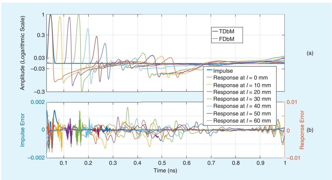
FIGURE 4. The impulse and responses pairs with (a) TDbM and FDbM and (b) the corresponding errors.
