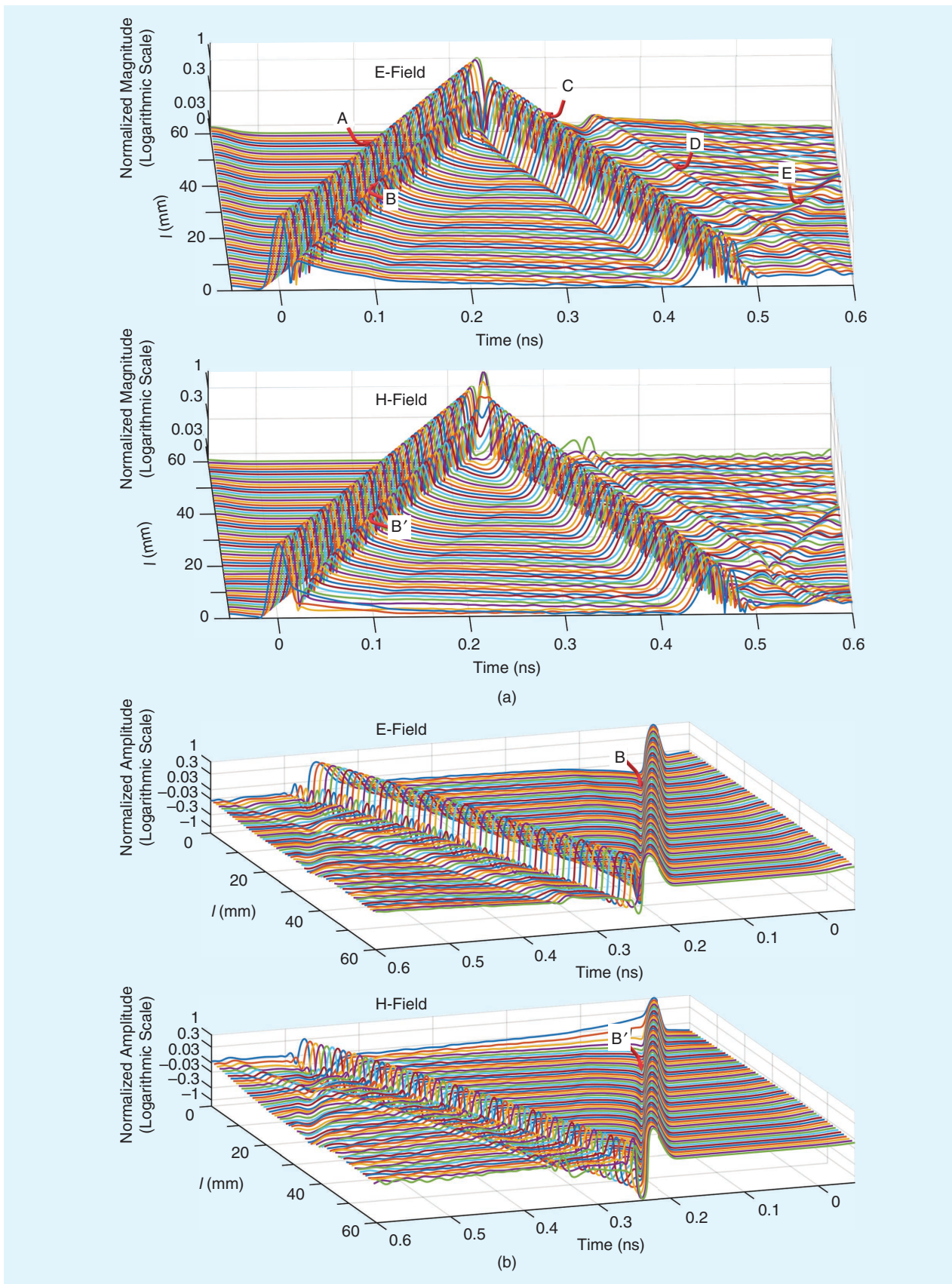
FIGURE 15. (a) The vector magnitude signals and (b) the curve normal/surface normal vector component signals of the E-/H-fields on the edge of the slot line versus time and versus distance from source l in the analysis band of 0–60 GHz.
