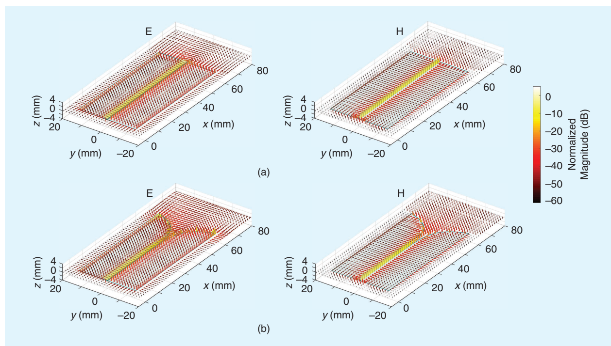
FIGURE 10. The E/H-field vectors at the time of the first peaks at the selected points on the analysis plane of (a) a slot line and (b) a Vivaldi antenna in the analysis bands of 0–30 GHz.
