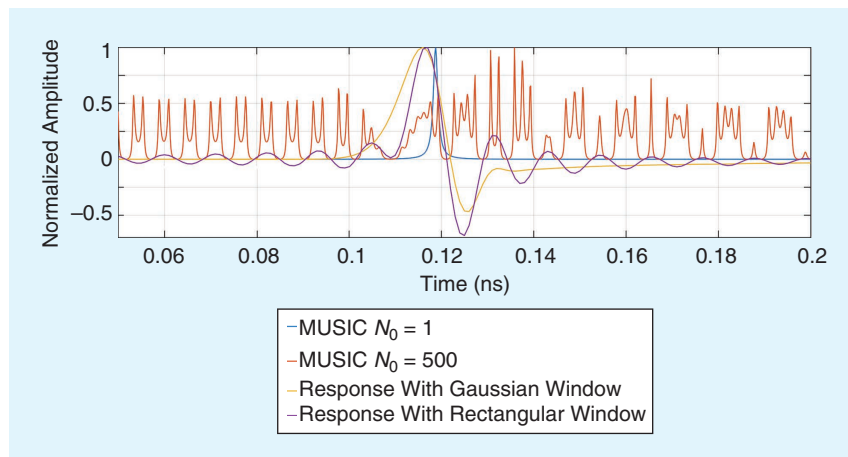
FIGURE 7. The MUSIC spectra and FDbM response signals at a point l = 30 mm along the slot line edge.
