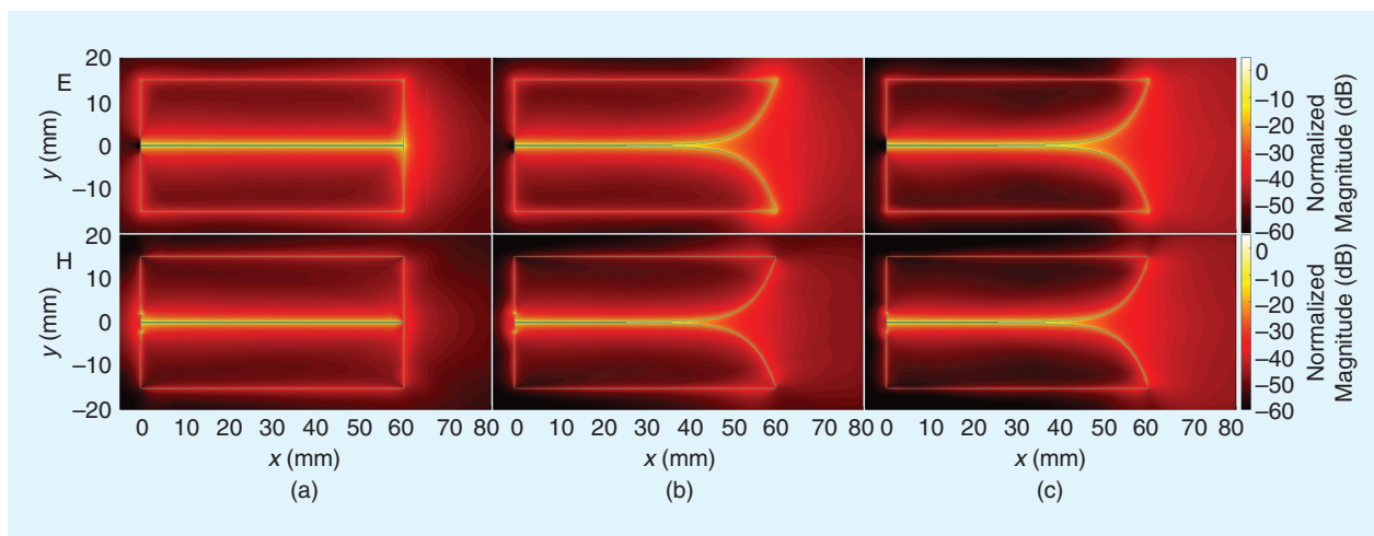
FIGURE 9. The maximum E/H-field vector magnitudes on the analysis plane z = \theta of (a) a slot line and (b) and (c) a Vivaldi antenna in the analysis bands of (a) and (b) 0–30 and (c) 0–60 GHz.
