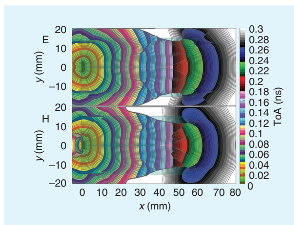
FIGURE 13. The ToAs based on the MUSIC spectra of E-/H-field vectors on the analysis plane of a Vivaldi antenna in the analysis band of 0–60 GHz.
