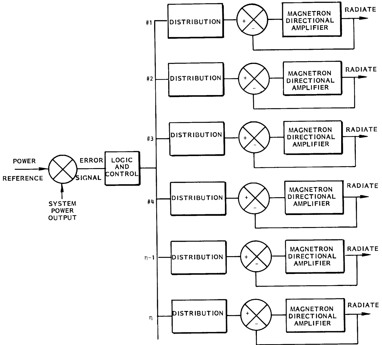
Figure 9-2. Control of Illumination Distribution by Logic and Control Center to Command Amount of Power Radiated from Each Step-Taper Level.
