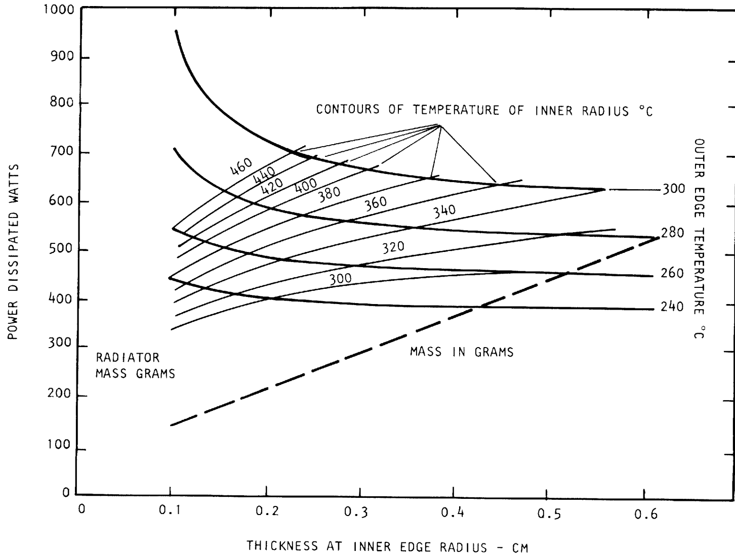
Figure 7-4. Information chart for selection of pyrographite radiator and determination of its mass. First, determine desired temperature at inner radius of radiator. Then select the desired value of power to be dissipated by the radiator and project this value horizontally until it intersects with the inner radius temperature curve. Vertical projection of this point determines both the thickness of the radiator at its inner edge and the mass of the radiator in grams. Temperature at edge of radiator may also be estimated.
