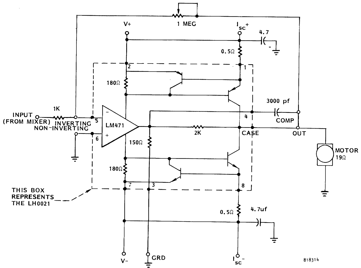
Figure 2-14. Schematic Diagram of Amplifier in Phase Tracking Feedback Loop.
