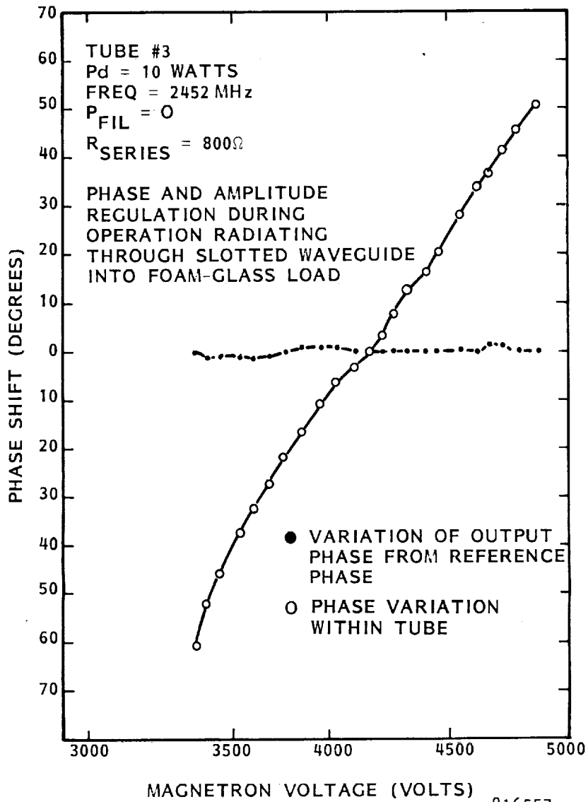
Figure 2-4. Phase Tracking of Output Phase to Reference Phase and Phase Shift through Magnetron Directional Amplifier as Function of Anode Voltage Level. Amplitude of Microwave Output is Held Constant.
