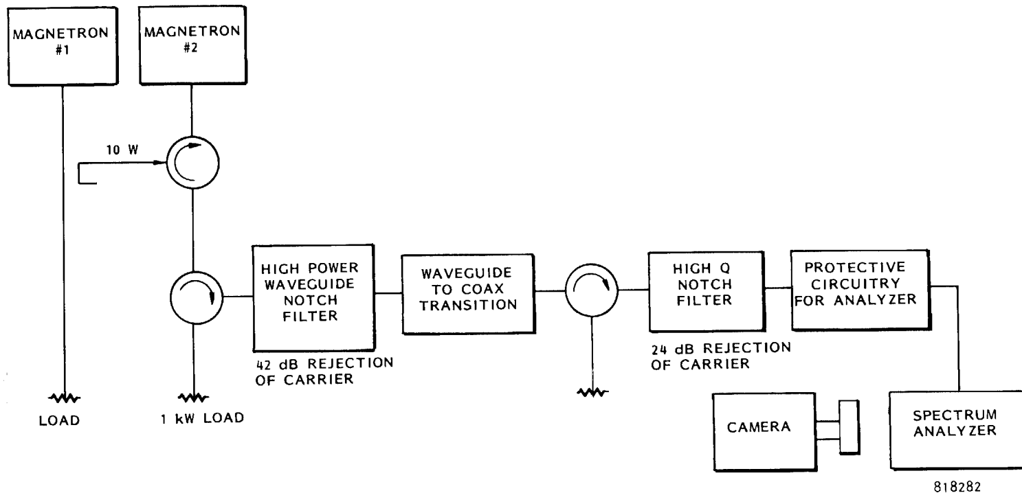
Figure 6-2. Improved Notched Filter Functional Test Block Diagram for Increased Sensitivity of Noise Measurements. Power not getting through high power waveguide filter is reflected back into a ferrite circulator and absorbed. Total filter consists of a cascade combination of a "T" section of WR 430 waveguide with a short in one arm adjusted to give minimum power transmission and a resonate cavity made from WR 284 tightly coupled to 3/4 inch coaxial line. A ferrite circulator is interposed between them to prevent coupling.
