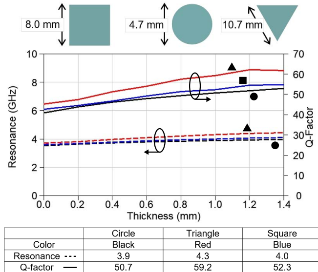
Fig. 10. Eigenmode analysis for resonant frequency and unloaded Q -factor for three canonical disk shapes as a function of disk thickness. A scalar \mu_{eff} is used in the HFSS simulations, calculated from Skyworks TTI-105 material parameters and with H_0 = 1750 Oe at f = 3.5 GHz. For example, for a thickness of 1.0 mm (table), the circular disk is resonant at 3.9 GHz with a corresponding Q=50.7 .
