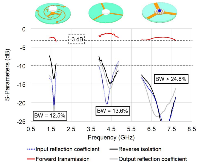
Fig. 22. Summary of measured S-parameters of three microstrip circulators designed with the same ferrite disk. The different frequency bands are a result of different magnetization distributions. The response at the 4.3-GHz center frequency is a result of a design using a nearly uniformly saturated disk, whereas the response at 1.6-GHz center frequency is obtained when the magnetization is nonuniform and below saturation. The 7-GHz response is due to a very inhomogeneous nonsaturated ferrite obtained from an array of PMs.
