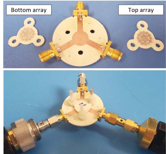
Fig. 19. Photograph of third prototype presented in Fig. 18. The circulator is designed to operate above FMR by applying a nonuniform MBF with an array of small PMs.
