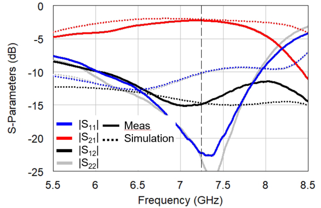
Fig. 20. Simulated and measured S-parameters of the circulator shown in Fig. 19. The measurements were performed with a two-port VNA, so isolation is measured by |S_{12}| . At 7.2GHz, measured parameters are |S_{11}| = -21.8 dB, |S_{21}| = -2.3 dB, and |S_{12}| = -15.0 dB.
