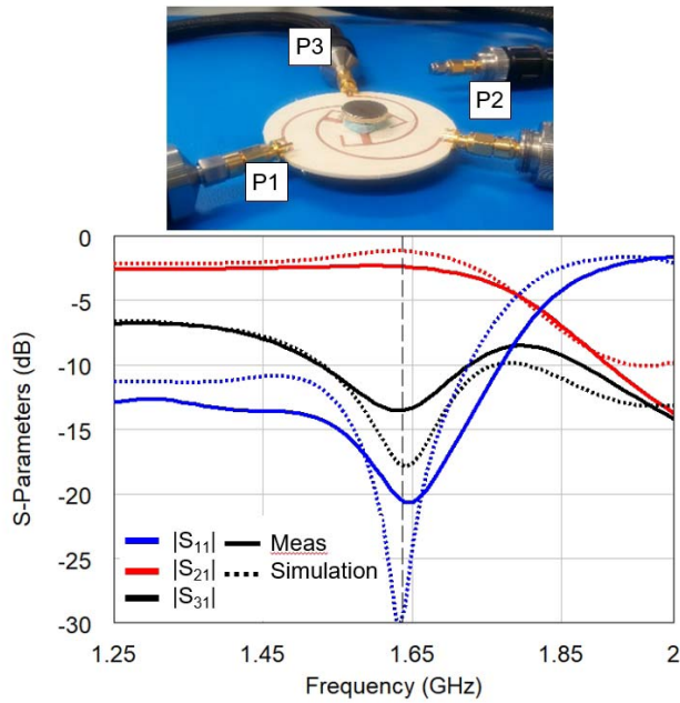
Fig. 17. Circulator operating in the UHF band having a reduced disk size by 40% [38]. The disk is initially designed to operate at 4.4GHz when the ferrite is uniformly saturated. Foam spacers are used to define the distance from the disk.
