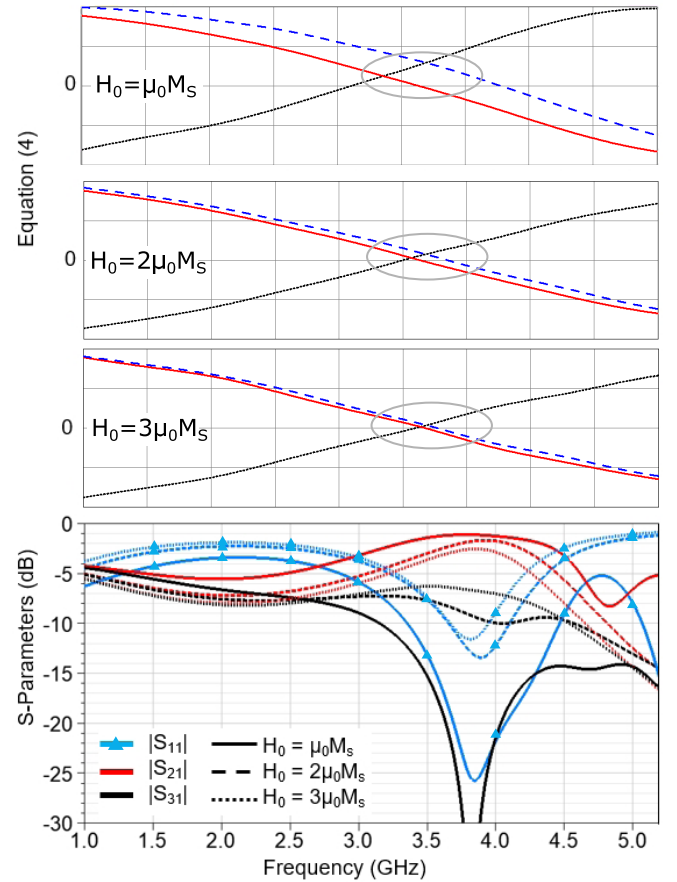
Fig. 7. Resonance analysis for n = 1 and H_0 = \mu_0 M_s, 2\mu_0 M_s, and 3\mu_0 M_s plotted with S-parameters, showing a relationship between (4) zero crossing, bandwidth, and MBF intensity. Three cases are traced: one considering \mu_{\text{eff}} as a scalar isotropic quantity (red solid line) and two counter-propagating modes resulting from a tensor [\mu] (dotted and dashed lines). Bottom: S-parameters resulting from the driven analysis for the three cases of the internal field.
