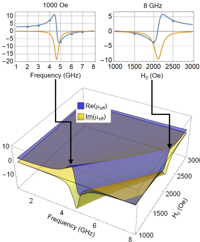
Fig. 6. Simulated real (blue, triangle) and imaginary (yellow) effective permeability \mu_{\text{eff}} for the Skyworks TTI-105 material over a frequency range f = [1, 8] GHz and H_0 = [1000, 3000] Oe. The 2-D graphs in the insets illustrate the local behavior with one of the variables fixed.
