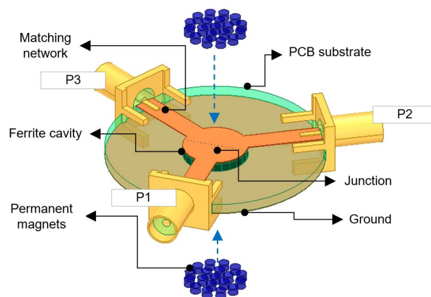
Fig. 1. Overall geometry of a Y-junction ferrite circulator. The PMs produce an MBF in the ferrite. A wave input at port P1 is transmitted to P2 with low insertion loss, whereas P3 is isolated (counterclockwise circulation) or transmitted to P3 with P2 isolated (clockwise), depending on the resonator mode and direction of MBF. The microstrip junction is above the ferrite disk and the PMs (shown here as an array) are placed immediately above and below the disk.
