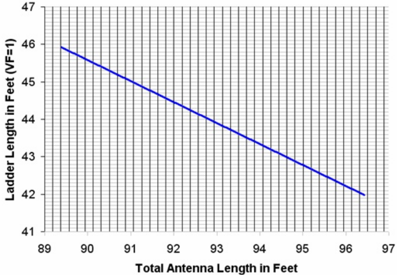
ZS6BKW Antenna/Ladder Feed
