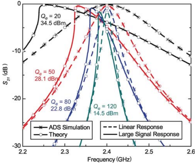
Fig. 8. Large-signal simulation of resonators with different external couplings.
