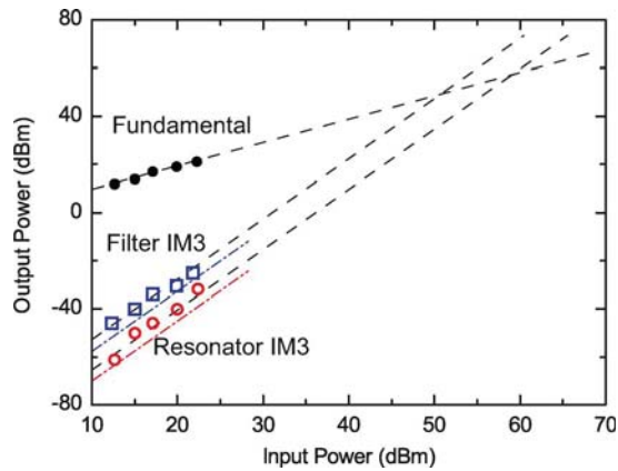
Fig. 21. Measured fundamental output power and IM3 for EVA resonators and filters. The dashed–dotted lines represent simulation results.
