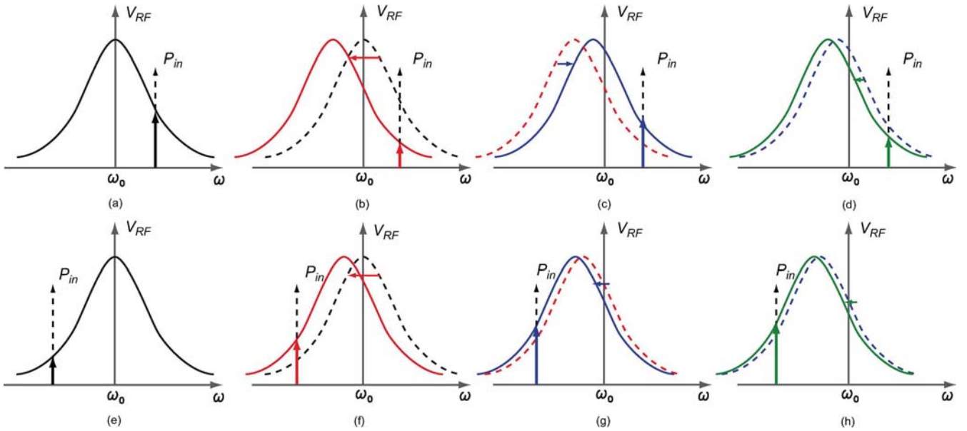
Fig. 3. Conceptual explanation of the frequency distortion with moderate input power. (a)–(d) Input signal higher than the resonant frequency leads to a negative feedback process. (e)–(h) Input signal lower than the resonant frequency leads to a positive feedback process.
