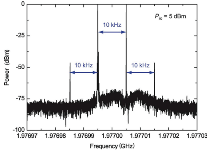
Fig. 20. Example measured output spectrum for the two-tone test of the EVA resonator with P_{in} = 5 dBm and \Delta f = 10 kHz.
