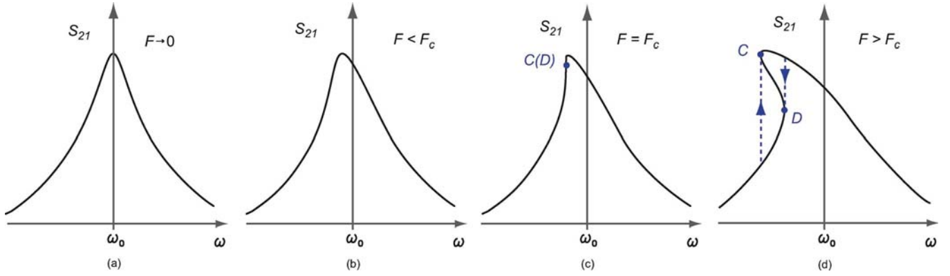
Fig. 2. Frequency responses of the nonlinear MEMS EVA resonator with different input power levels. (a) Symmetric response with very small input. (b) Frequency distortion with medium input power. (c) Onset of bifurcation. (d) Bifurcation.
