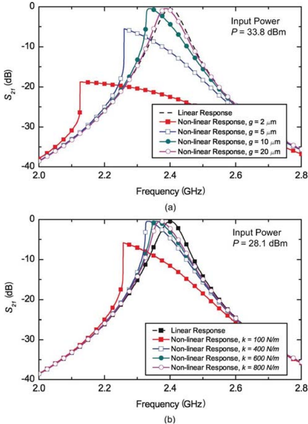
Fig. 9. Large-signal simulation of resonators with (a) different capacitive gaps and (b) different spring constant. The resonant frequency and C_r are kept the same by setting appropriate post radius. The nominal parameters of the simulated resonator are listed in Table I.
