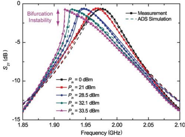
Fig. 18. Measured and simulated self-actuation characteristics of the EVA tunable resonator.
