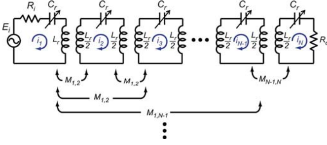
Fig. 4. Schematic of a general coupled-resonator MEMS EVA tunable filter. The graph follows the convention of [17].
