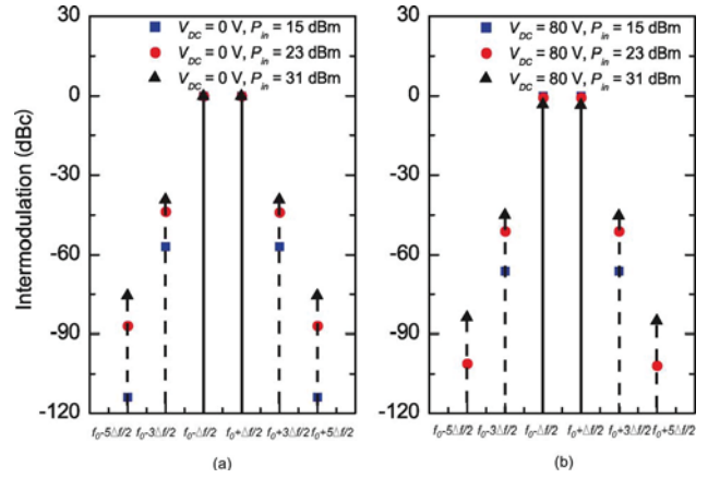
Fig. 12. Simulated spectrum of IMD products of an EVA tunable resonator with (a) 0 V and (b) 80 V actuation voltage. Parameters of the simulated resonator is listed in Table I.
