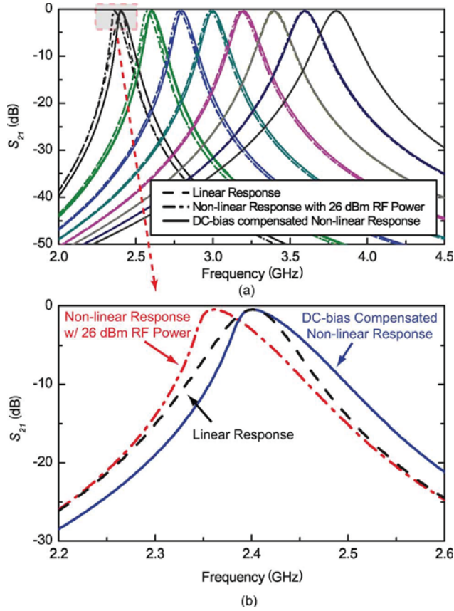
Fig. 11. (a) Simulated linear and nonlinear responses of an EVA tunable resonator with varying dc bias voltages. (b) Close-up plot of the tunable resonator at 2.4 GHz showing compensation for frequency drift by applying additional dc bias.
