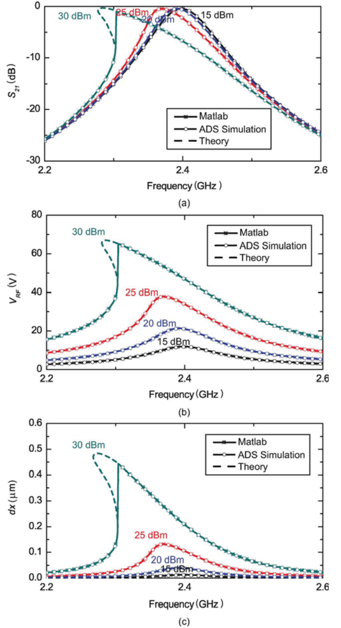
Fig. 7. ADS simulation of large-signal responses of a MEMS EVA tunable resonator using nonlinear circuit model shown in Fig. 1. (a) S_{21} . (b) RF voltage on the varactor. (c) Diaphragm deflection under different input power levels.
