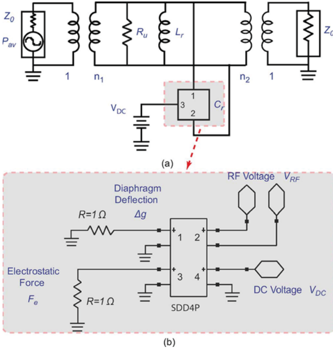
Fig. 6. (a) Nonlinear circuit model for the EVA tunable resonator. (b) Nonlinear varactor model using Agilent ADS four-port SDD.
