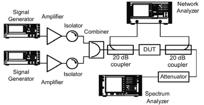
Fig. 19. Measurement setup for two-tone intermodulation characterization.
