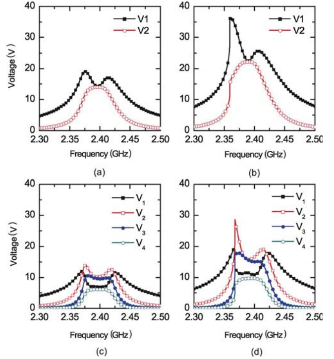
Fig. 15. Simulated RF voltage on the resonator in a two-pole filter and four-pole filter. (a) P_{in} = 15 dBm. (b) P_{in} = 19 dBm. (c) P_{in} = 11 dBm. (d) P_{in} = 15 dBm.
