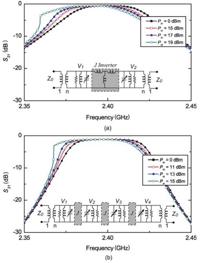
Fig. 14. Simulated nonlinear responses of (a) two-pole and (b) four-pole 2% Butterworth filter.
