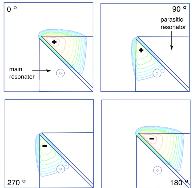
FIGURE 4. Electric-field magnitude throughout one frequency cycle at 2.45 GHz. Both patches operate in the TE 110 -mode (reduced size), with a phase difference of approximately 90° between both resonators.
