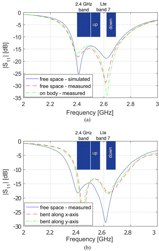
FIGURE 6. The antenna shows good impedance matching to a 50 \Omega reference impedance under the different operating conditions. (a) Free space (simulated and measured) and on-body (measured) agree well, and (b) stable performance is observed when the antenna is bent around a cylinder with radius of 9 cm.
