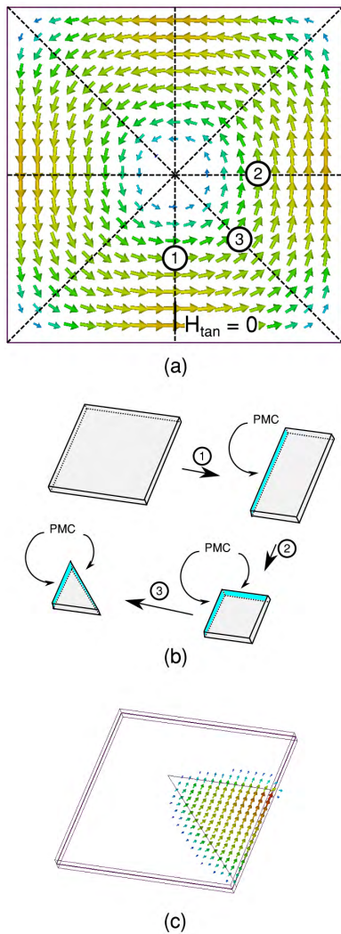
FIGURE 3. Half-mode miniaturization. (a) Symmetry planes of a rectangular cavity. The tangential component of the magnetic field is zero, mimicking a Perfect Magnetic Conductor (PMC). (b) The cavity can be miniaturized by removing half of the cavity. The open boundary acts as a virtual magnetic wall. This can be repeated for each remaining symmetry plane. (c) An 8th mode cavity has a much smaller footprint, but the same operating frequency and mode distribution as the original cavity.
