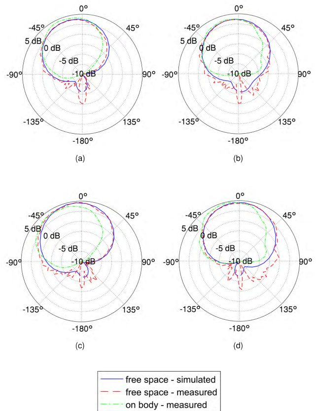
FIGURE 7. Radiation pattern of the proposed antenna. The simulated and measured free-space total gain and measured on-body gain are shown in (a) the horizontal (xz) plane at 2.45 GHz, (b) the vertical (yz) plane at 2.45 GHz, (c) the horizontal (xz) plane at 2.655 GHz and (d) the vertical (yz) plane at 2.655 GHz.
