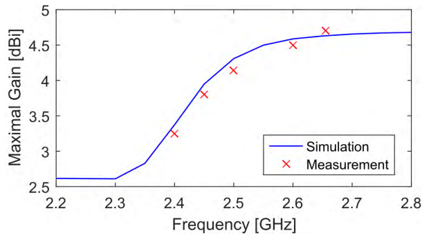
FIGURE 8. Simulated and measured maximal gain of the proposed antenna.
