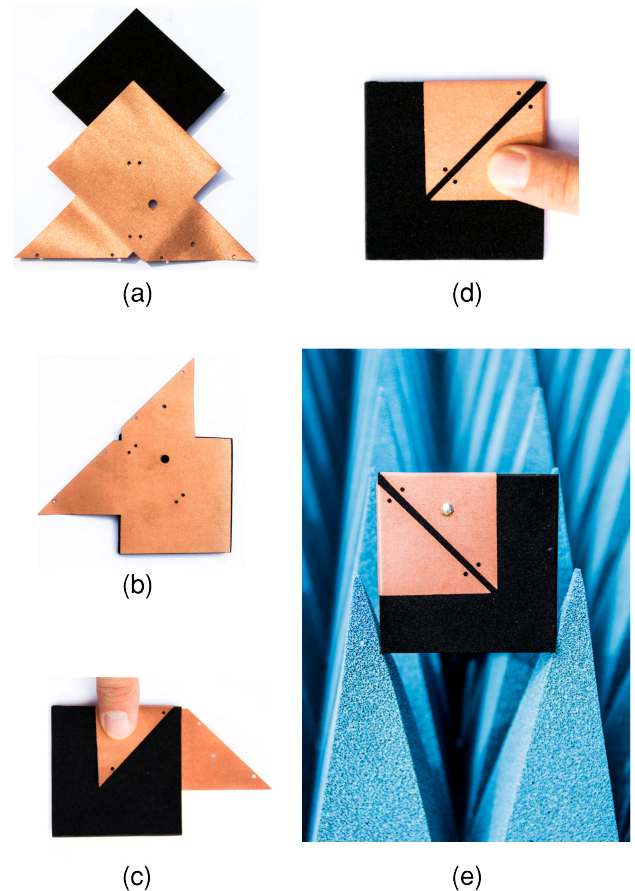
FIGURE 5. Assembly of the wearable antenna. (a) Substrate and e-textile are patterned with laser cutter. The conductive parts are made from a single sheet and small alignment holes in substrate and conductor are used to facilitate reliable manufacturing. (b) The ground plane is glued to the back side of the substrate. (c) The first resonator is created by folding the flap over the substrate. (d) The second resonator is realized accordingly. (e) Photograph of the finalized antenna.
