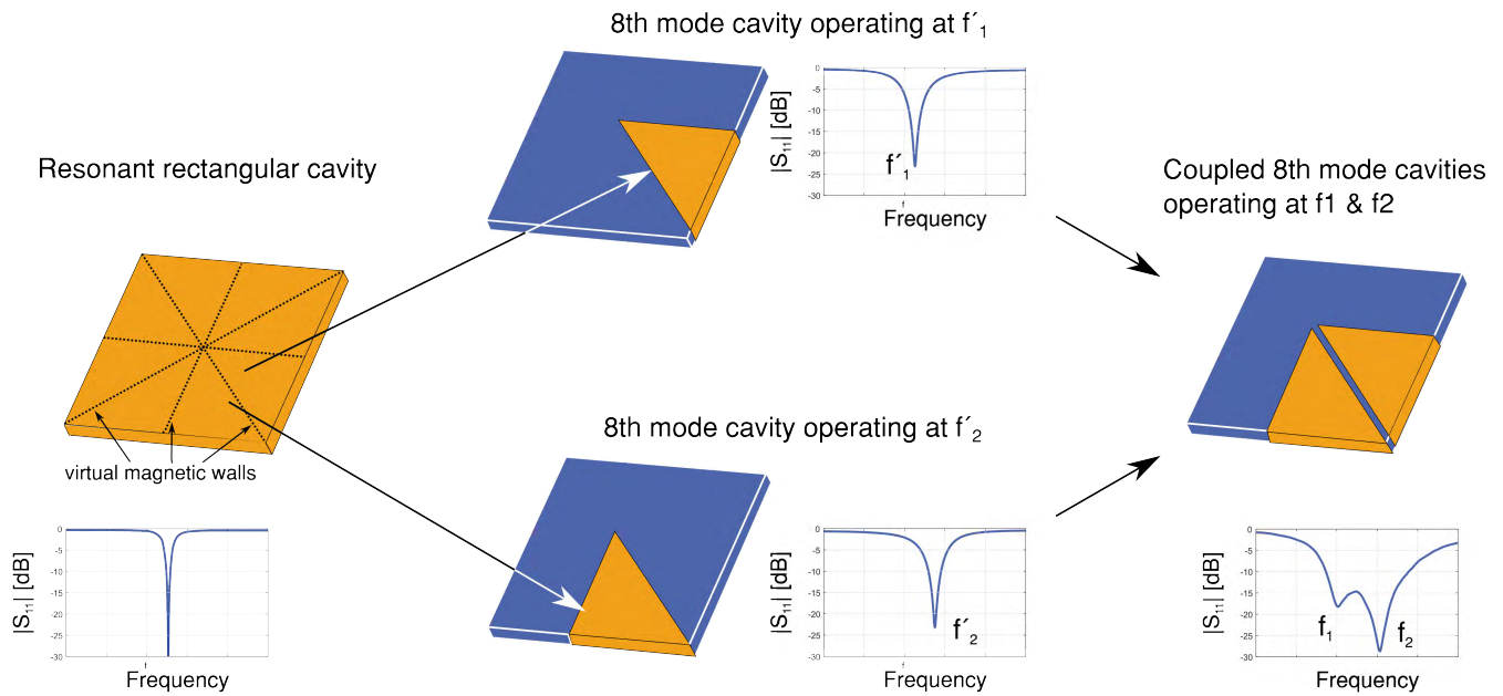
FIGURE 2. Design evolution from left to right. Starting point is a resonant rectangular cavity. By bisected along virtual magnetic walls (where tangential components of the magnetic field vanish), two miniaturized resonant cavities are obtained. They operate at two closely spaced frequencies and occupy only 1/8^{\text{th}} of the original resonator area. Through combination of the leaking resonators, a coupled-cavity system yields wideband operation in combination with a small footprint.
