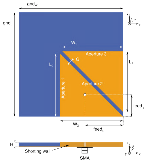
FIGURE 1. The proposed novel antenna topology: a system of two coupled eighth-mode resonators excited by a low-complexity probe feed. L1 = 29.5 , W1 = 29.5 , L2 = 30.5 , W2 = 30.5 , G = 1.41 , gnd_w = 50 , gnd_l = 50 , H = 3.5 , feed_x = 18.5 , feed_y = 10.5 (all dimensions in mm). Substrate parameters: \epsilon_r = 1.495 , \tan \delta = 0.015 .
