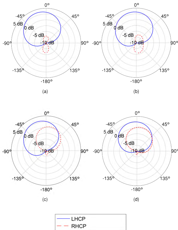
FIGURE 9. Simulated LHCP and RHCP components of the antenna gain at (a) the horizontal (xz) plane at 2.45 GHz, (b) the vertical (yz) plane at 2.45 GHz, (c) the horizontal (xz) plane at 2.655 GHz and (d) the vertical (yz) plane at 2.655 GHz.
