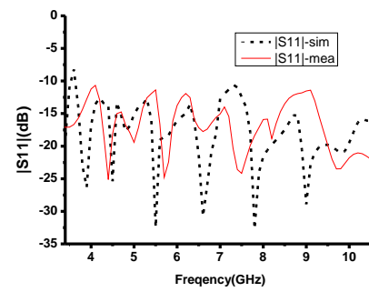
Fig. 15. |S_{11}| of the feed antenna
