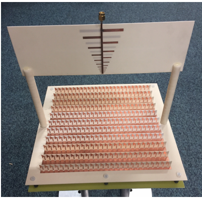
Fig. 12. Photograph of the TCDR.
