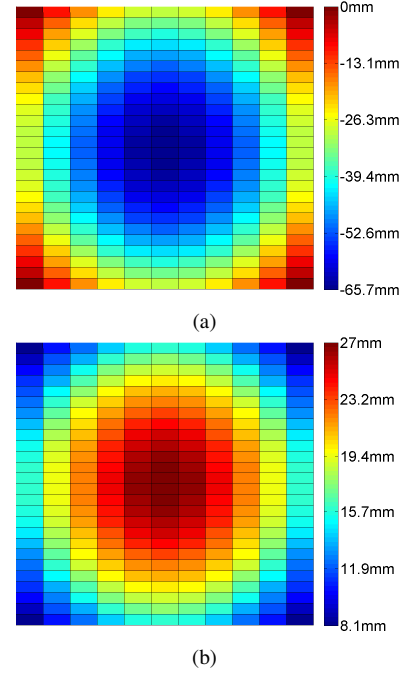
Fig. 6. Required (a) equivalent distance delay and (b) length of the delay line for each element on the reflecting surface.
