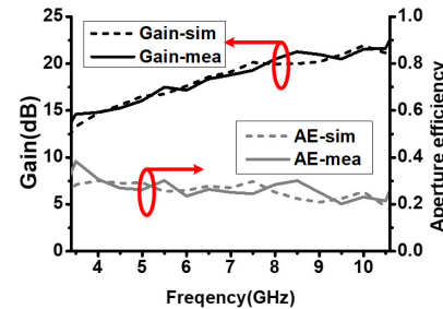
Fig. 16. Simulated and measured gains and aperture efficiency.
