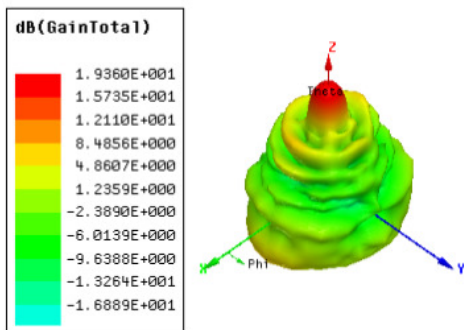
Fig. 14. Simulated 3D pattern at 7GHz.
