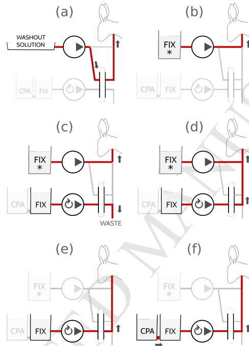
Figure 3: Initial fixation was accomplished by replacing the container of washout solution (a) with a container of 2L of fixative with additives (FIX*) and bypassing the filter (b) to avoid fixative dilution by fluid in the filter. While this initial fixative perfusion was underway, we cleared the filter of blood washout solution by perfusing it with fixative in parallel using the computer-controlled pump (c). Transfer to computer control was accomplished by joining the two pathways (d) and gradually decreasing the speed of the manual pump, causing the computer to increase the rate of the computer-controlled pump to compensate, without disrupting flow to the cephalon (e). After 45 min of total fixation time, we started the CPA ramp (f).
