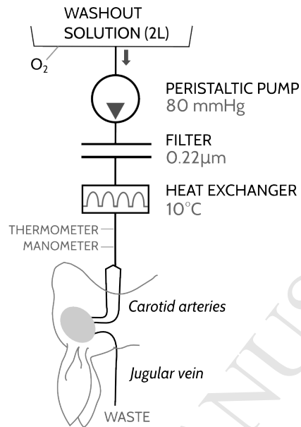
Figure 1: The washout cart was used to wash out the rabbit's blood, then to move the cephalon to the CPA circuit (Fig. 2) for fixation and cryoprotectant introduction. The washout circuit consisted of a 2L reservoir of oxygenated blood washout solution, a 0.22 μm filter, heat exchanger (ice water and heat exchanger pump not pictured), and a thermometer and manometer to monitor perfusion parameters.
