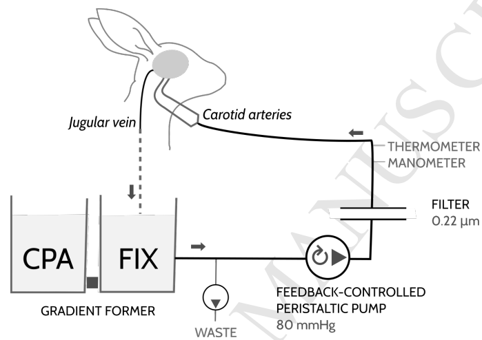
Figure 2: The CPA circuit was entirely contained in a fume hood, and was used to fix the rabbit brain and to introduce CPA. It consisted of a gradient generator, a computer-controlled peristaltic pump, a waste pump, a 0.22 \mu\text{m} filter, and a digital manometer and thermometer. The gradient generator consisted of adjacent reservoirs of cryoprotectant solution (CPA) and fixative solution (FIX) connected by a short tube. The fixative reservoir was continuously stirred by a magnetic stir bar. A waste pump was used to lower the level of the gradient generator and create the gradient. The computer adjusted the flow rate of the feedback-controlled perfusion pump to maintain constant pressure of the cephalon. To mimic standard neurobiology procedures, fixation was done at approximately room temperature. We used a series of switches to transition the cephalon to this circuit without interrupting flow (see Fig. 3).
